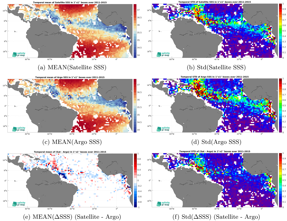
Figure 6: Temporal mean (left) and Std (right) of SSS from Aquarius SSS L4 OI v5 - Weekly (IPRC) (top), Argo (middle), and of \Delta\text{SSS} (Satellite - Argo). Only match-up pairs are used to generate these maps.
