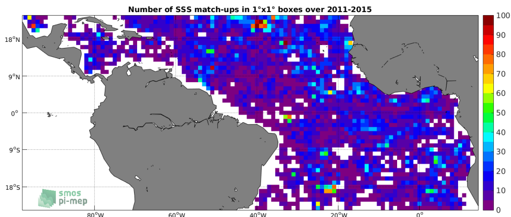
Figure 4: Number of SSS match-ups between Argo SSS and the Aquarius-L4-IPRC-V5-WEEKLY SSS product for the Tropical Atlantic Ocean Pi-MEP region over 1^\circ \times 1^\circ boxes and for the full satellite product period.
