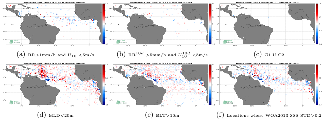
Figure 12: Temporal mean gridded over spatial boxes of size 1^\circ \times 1^\circ of \Delta SSS (Aquarius-L4-IPRC-V5-WEEKLY - Argo) for 6 different subdatasets corresponding to: RR > 1\text{mm/h} and U_{10} < 5\text{m/s} (a), RR^{10d} > 5\text{mm/h} and U_{10}^{10d} < 5\text{m/s} (b), C1 U C2 (c), MLD < 20\text{m} (d), BLT > 10\text{m} (e), Locations where WOA2013 SSS STD > 0.2 (f).
