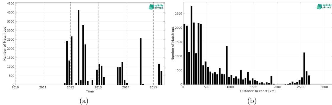
Figure 1: Number of match-ups between TSG (SAMOS) and Aquarius SSS L4 OI v5 - Monthly (IPRC) SSS as a function of time (a) and as function of the distance to coast (b) over the Tropical Atlantic Ocean Pi-MEP region and for the full satellite product period.
