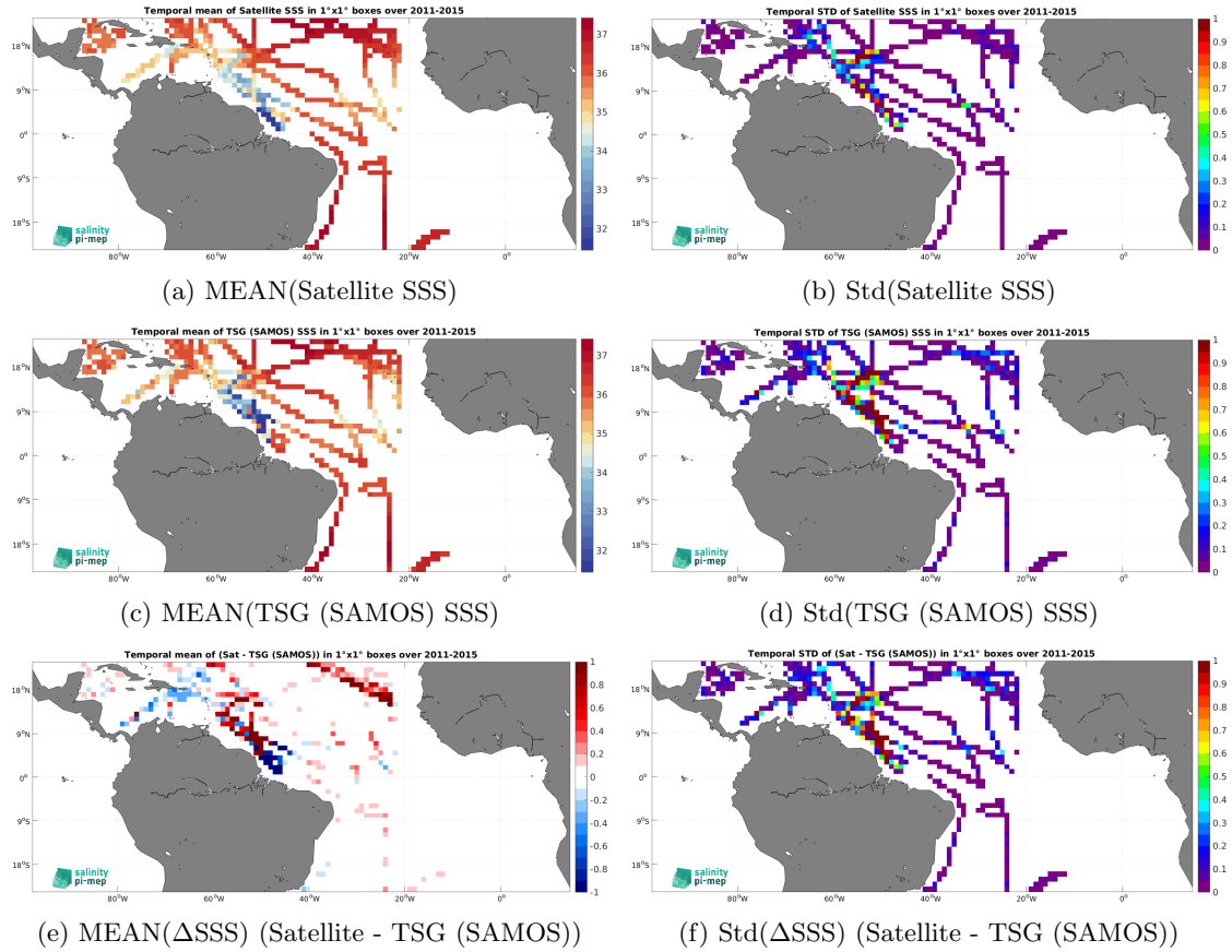
Figure 6: Temporal mean (left) and Std (right) of SSS from Aquarius SSS L4 OI v5 - Monthly (IPRC) (top), TSG (SAMOS) (middle), and of \Delta\text{SSS} (Satellite - TSG (SAMOS)). Only match-up pairs are used to generate these maps.
