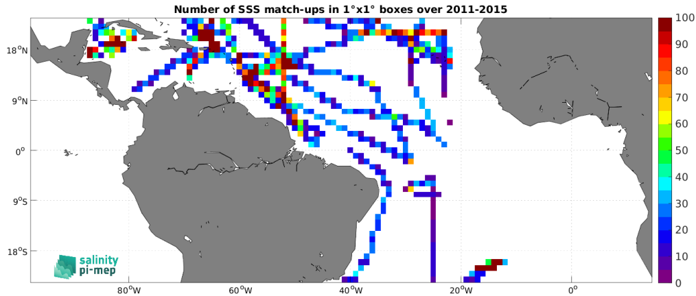
Figure 4: Number of SSS match-ups between TSG (SAMOS) SSS and the Aquarius SSS L4 OI v5 - Monthly (IPRC) SSS product for the Tropical Atlantic Ocean Pi-MEP region over 1^\circ \times 1^\circ boxes and for the full satellite product period.
