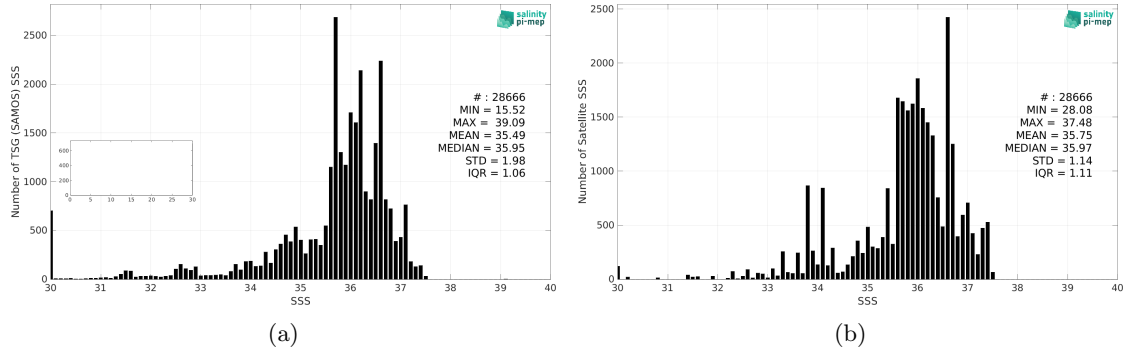
Figure 2: Histograms of SSS from TSG (SAMOS) (a) and Aquarius SSS L4 OI v5 - Monthly (IPRC) (b) considering all match-up pairs per bins of 0.1 over the Tropical Atlantic Ocean Pi-MEP region and for the full satellite product period.
