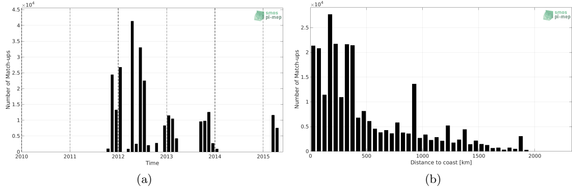
Figure 1: Number of match-ups between TSG (SAMOS) and Aquarius SSS L4 OI v5 - Monthly (IPRC) SSS as a function of time (a) and as function of the distance to coast (b) over the Tropical Atlantic Ocean Pi-MEP region and for the full satellite product period.
