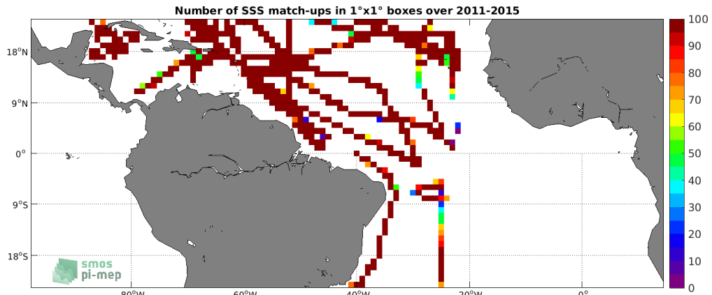
Figure 4: Number of SSS match-ups between TSG (SAMOS) SSS and the Aquarius SSS L4 OI v5 - Monthly (IPRC) SSS product for the Tropical Atlantic Ocean Pi-MEP region over 1°x1° boxes and for the full satellite product period.
