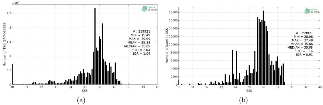
Figure 2: Histograms of SSS from TSG (SAMOS) (a) and Aquarius SSS L4 OI v5 - Monthly (IPRC) (b) considering all match-up pairs per bins of 0.1 over the Tropical Atlantic Ocean Pi-MEP region and for the full satellite product period.
