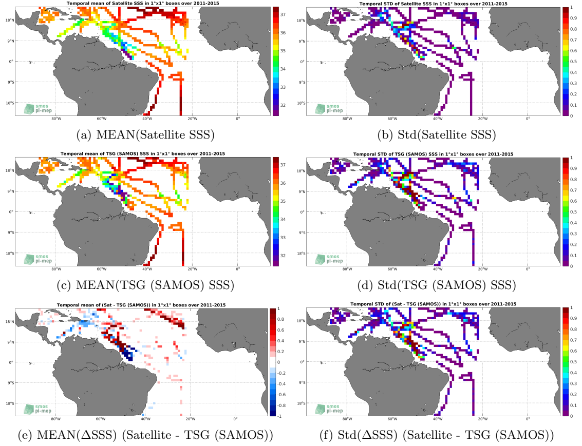
Figure 6: Temporal mean (left) and Std (right) of SSS from Aquarius SSS L4 OI v5 - Monthly (IPRC) (top), TSG (SAMOS) (middle), and of \Delta SSS (Satellite - TSG (SAMOS)). Only match-up pairs are used to generate these maps.
