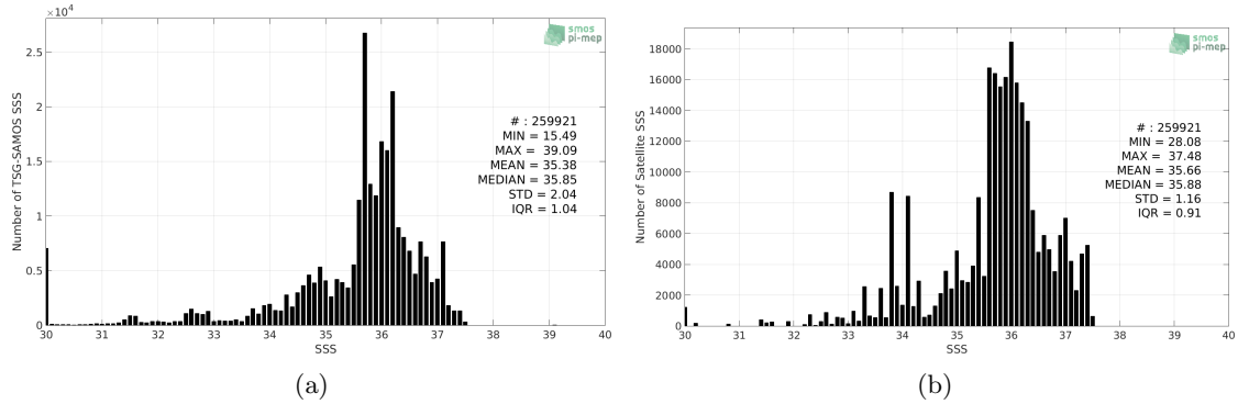
Figure 2: Histograms of SSS from TSG-SAMOS (a) and Aquarius-L4-IPRC-V5-MONTHLY (b) considering all match-up pairs per bins of 0.1 over the Tropical Atlantic Ocean Pi-MEP region and for the full satellite product period.
