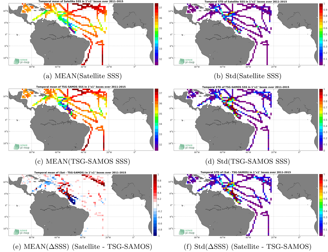
Figure 6: Temporal mean (left) and Std (right) of SSS from Aquarius-L4-IPRC-V5-MONTHLY (top), TSG-SAMOS (middle), and of \Delta SSS (Satellite - TSG-SAMOS). Only match-up pairs are used to generate these maps.
