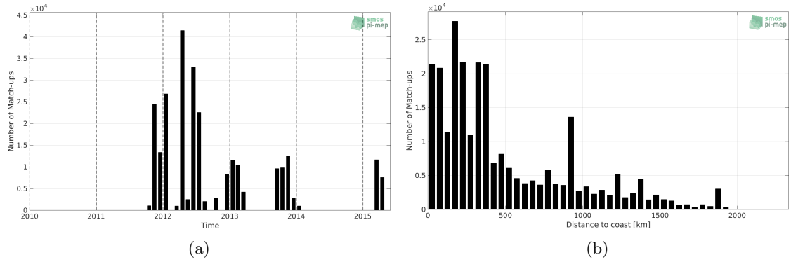
Figure 1: Number of match-ups between TSG-SAMOS and Aquarius-L4-IPRC-V5-MONTHLY SSS as a function of time (a) and as function of the distance to coast (b) over the Tropical Atlantic Ocean Pi-MEP region and for the full satellite product period.
