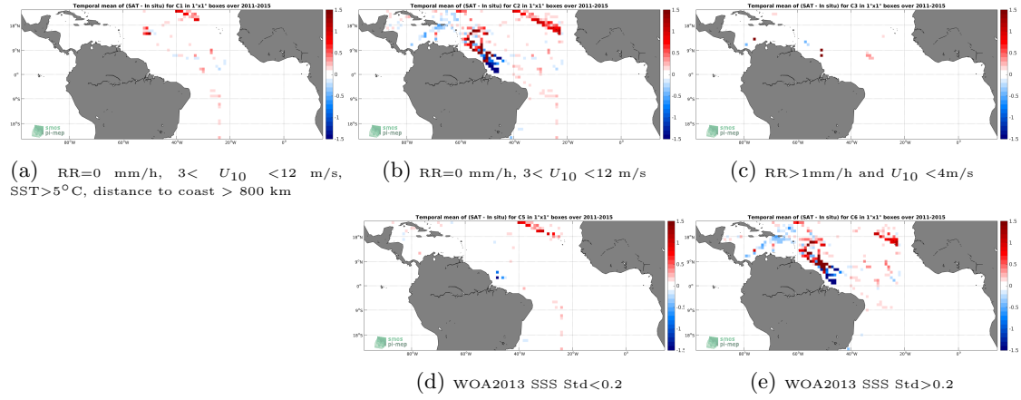
Figure 12: Temporal mean gridded over spatial boxes of size 1^\circ \times 1^\circ of \Delta SSS (Aquarius-L4-IPRC-V5-MONTHLY - TSG-SAMOS) for 5 different subdatasets corresponding to:RR=0 mm/h, 3 < U_{10} < 12 m/s, SST >5^\circ\text{C} , distance to coast > 800 km (a), RR=0 mm/h, 3 < U_{10} < 12 m/s (b), RR >1 mm/h and U_{10} < 4 m/s (c), WOA2013 SSS Std <0.2 (d), WOA2013 SSS Std >0.2 (e).
