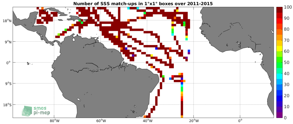
Figure 4: Number of SSS match-ups between TSG-SAMOS SSS and the Aquarius-L4-IPRC-V5-MONTHLY SSS product for the Tropical Atlantic Ocean Pi-MEP region over 1°x1° boxes and for the full satellite product period.
