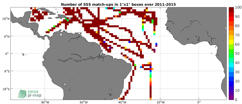
Figure 4: Number of SSS match-ups between TSG-SAMOS SSS and the Aquarius-L4-IPRC-V5-MONTHLY SSS product for the Tropical Atlantic Ocean Pi-MEP region over 1^\circ \times 1^\circ boxes and for the full satellite product period.
