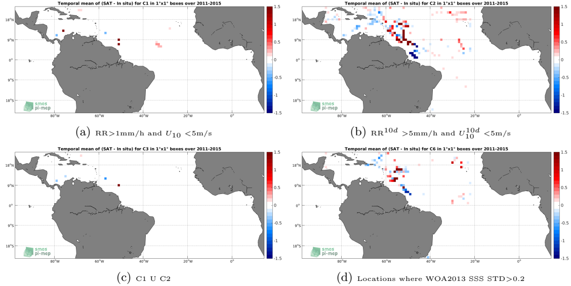
Figure 12: Temporal mean gridded over spatial boxes of size 1^\circ \times 1^\circ of \Delta SSS (Aquarius-L4-IPRC-V5-MONTHLY - TSG-SAMOS) for 4 different subdatasets corresponding to: RR > 1mm/h and U_{10} < 5\text{m/s} (a), RR^{10d} > 5\text{mm/h} and U_{10}^{10d} < 5\text{m/s} (b), C1 U C2 (c), Locations where WOA2013 SSS STD > 0.2 (d).
