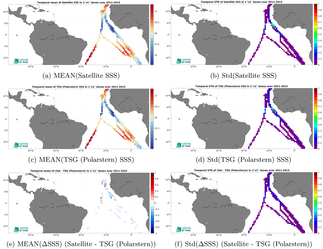
Figure 7: Temporal mean (left) and Std (right) of SSS from Aquarius SSS L4 OI v5 - Monthly (IPRC) (top), TSG (Polarstern) (middle), and of \Delta\text{SSS} (Satellite - TSG (Polarstern)). Only match-up pairs are used to generate these maps.
