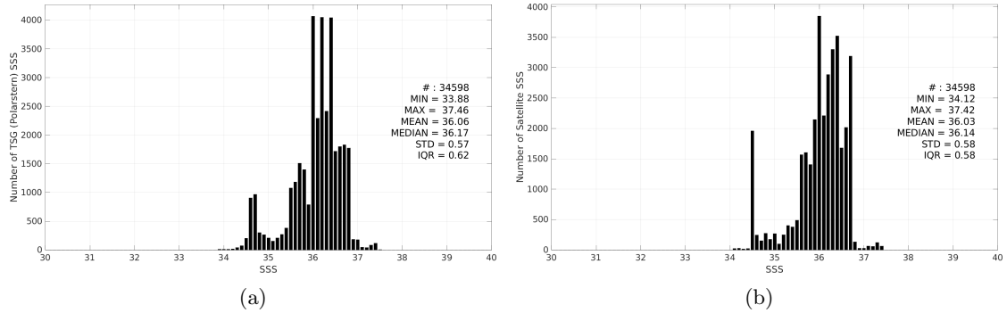
Figure 3: Histograms of SSS from TSG (Polarstern) (a) and Aquarius SSS L4 OI v5 - Monthly (IPRC) (b) considering all match-up pairs per bins of 0.1 over the Tropical Atlantic Ocean Pi-MEP region and for the full satellite product period.
