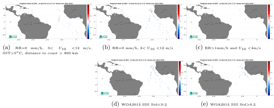
Figure 14: Temporal mean gridded over spatial boxes of size 1^\circ \times 1^\circ of \Delta SSS (Aquarius SSS L4 OI v5 - Monthly (IPRC) - TSG (Polarstern)) for 5 different subdatasets corresponding to:RR=0 mm/h, 3 < U_{10} < 12 m/s, SST >5^\circ\text{C} , distance to coast > 800 km (a), RR=0 mm/h, 3 < U_{10} < 12 m/s (b), RR >1 mm/h and U_{10} < 4 m/s (c), WOA2013 SSS Std <0.2 (d), WOA2013 SSS Std >0.2 (e).
