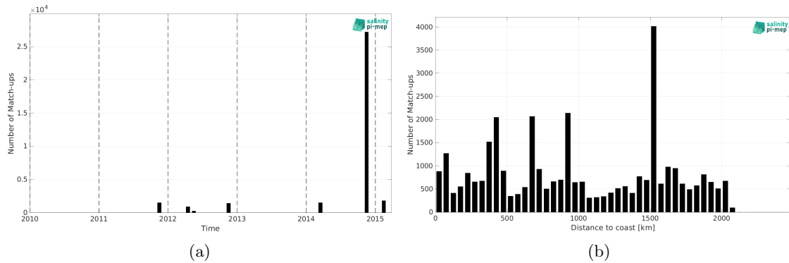
Figure 2: Number of match-ups between TSG (Polarstern) and Aquarius SSS L4 OI v5 - Monthly (IPRC) SSS as a function of time (a) and as function of the distance to coast (b) over the Tropical Atlantic Ocean Pi-MEP region and for the full satellite product period.
