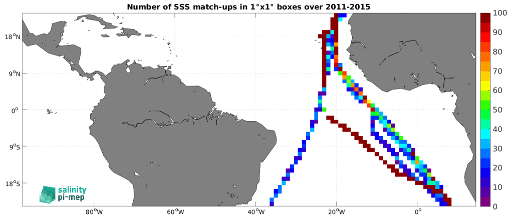
Figure 5: Number of SSS match-ups between TSG (Polarstern) SSS and the Aquarius SSS L4 OI v5 - Monthly (IPRC) SSS product for the Tropical Atlantic Ocean Pi-MEP region over 1^\circ \times 1^\circ boxes and for the full satellite product period.
