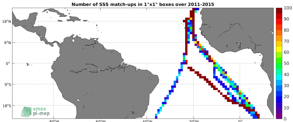
Figure 4: Number of SSS match-ups between TSG (Polarstern) SSS and the Aquarius SSS L4 OI v5 - Monthly (IPRC) SSS product for the Tropical Atlantic Ocean Pi-MEP region over 1°x1° boxes and for the full satellite product period.
