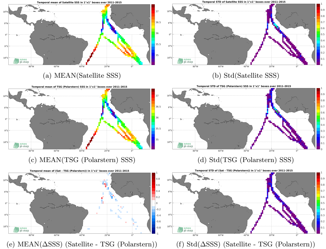
Figure 6: Temporal mean (left) and Std (right) of SSS from Aquarius SSS L4 OI v5 - Monthly (IPRC) (top), TSG (Polarstern) (middle), and of \Delta SSS (Satellite - TSG (Polarstern)). Only match-up pairs are used to generate these maps.
