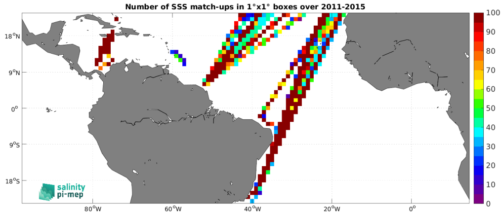
Figure 5: Number of SSS match-ups between TSG (LEGOS-DM) SSS and the Aquarius SSS L4 OI v5 - Monthly (IPRC) SSS product for the Tropical Atlantic Ocean Pi-MEP region over 1^\circ \times 1^\circ boxes and for the full satellite product period.
