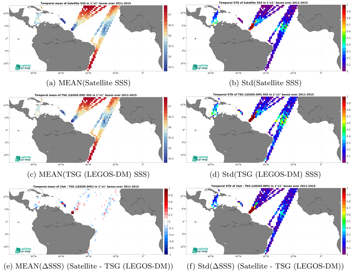
Figure 7: Temporal mean (left) and Std (right) of SSS from Aquarius SSS L4 OI v5 - Monthly (IPRC) (top), TSG (LEGOS-DM) (middle), and of \Delta\text{SSS} (Satellite - TSG (LEGOS-DM)). Only match-up pairs are used to generate these maps.
