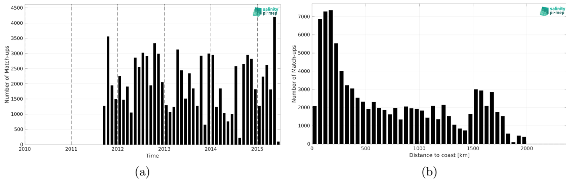
Figure 2: Number of match-ups between TSG (LEGOS-DM) and Aquarius SSS L4 OI v5 - Monthly (IPRC) SSS as a function of time (a) and as function of the distance to coast (b) over the Tropical Atlantic Ocean Pi-MEP region and for the full satellite product period.
