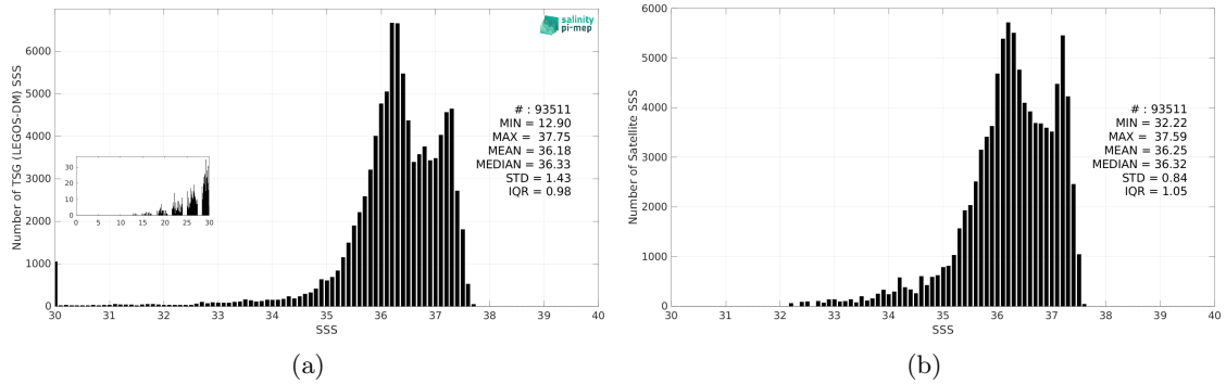
Figure 3: Histograms of SSS from TSG (LEGOS-DM) (a) and Aquarius SSS L4 OI v5 - Monthly (IPRC) (b) considering all match-up pairs per bins of 0.1 over the Tropical Atlantic Ocean Pi-MEP region and for the full satellite product period.
