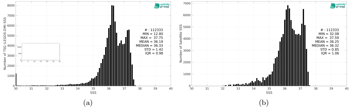
Figure 2: Histograms of SSS from TSG (LEGOS-DM) (a) and Aquarius SSS L4 OI v5 - Monthly (IPRC) (b) considering all match-up pairs per bins of 0.1 over the Tropical Atlantic Ocean Pi-MEP region and for the full satellite product period.
