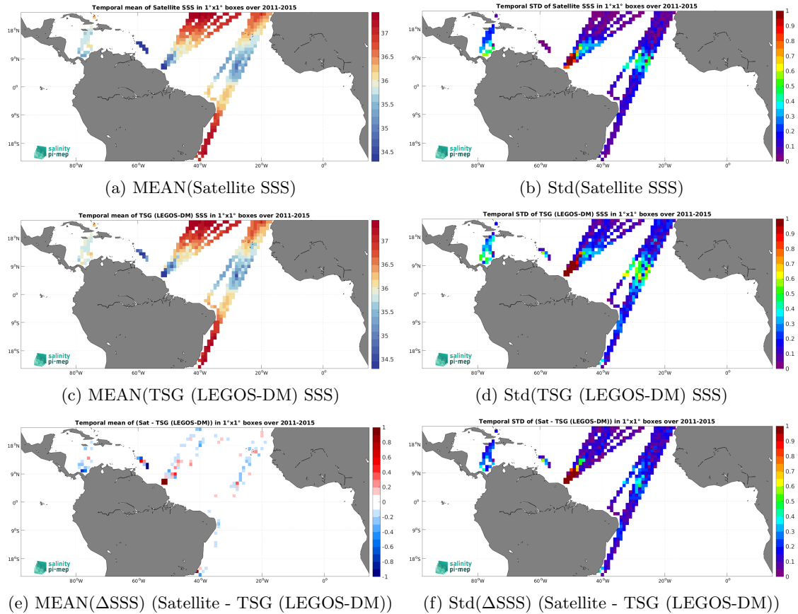
Figure 6: Temporal mean (left) and Std (right) of SSS from Aquarius SSS L4 OI v5 - Monthly (IPRC) (top), TSG (LEGOS-DM) (middle), and of \Delta\text{SSS}(\text{Satellite} - \text{TSG (LEGOS-DM)}) . Only match-up pairs are used to generate these maps.
