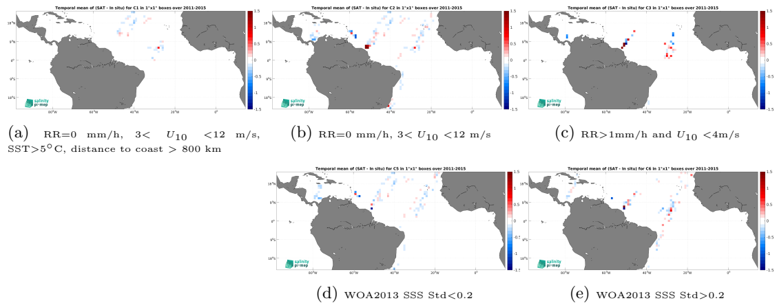
Figure 12: Temporal mean gridded over spatial boxes of size 1^\circ \times 1^\circ of \Delta\text{SSS} (Aquarius SSS L4 OI v5 - Monthly (IPRC) - TSG (LEGOS-DM)) for 5 different subdatasets corresponding to:RR=0 mm/h, 3 < U_{10} < 12 m/s, SST >5^\circ\text{C} , distance to coast > 800 km (a), RR=0 mm/h, 3 < U_{10} < 12 m/s (b), RR >1 mm/h and U_{10} < 4 m/s (c), WOA2013 SSS Std <0.2 (d), WOA2013 SSS Std >0.2 (e).
