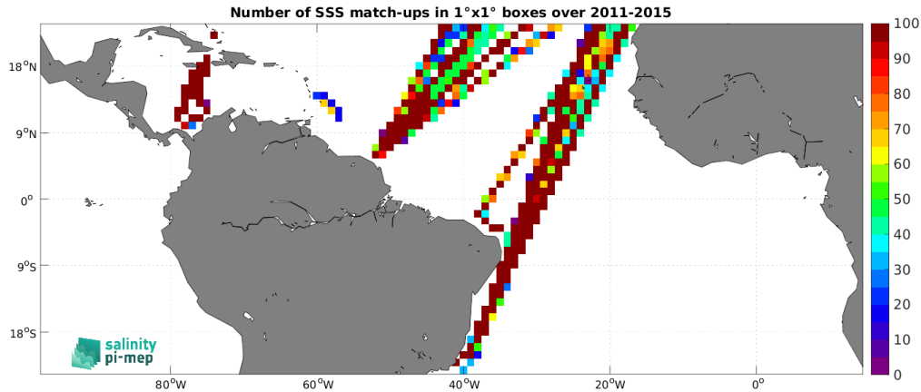
Figure 4: Number of SSS match-ups between TSG (LEGOS-DM) SSS and the Aquarius SSS L4 OI v5 - Monthly (IPRC) SSS product for the Tropical Atlantic Ocean Pi-MEP region over 1^\circ \times 1^\circ boxes and for the full satellite product period.
