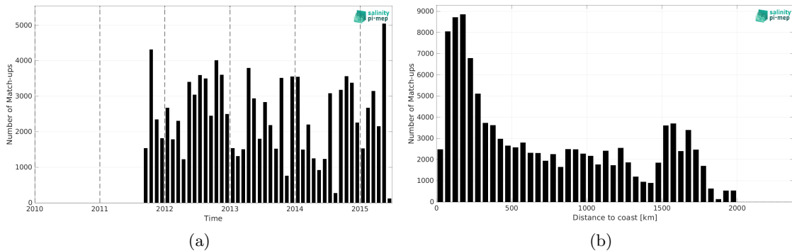
Figure 1: Number of match-ups between TSG (LEGOS-DM) and Aquarius SSS L4 OI v5 - Monthly (IPRC) SSS as a function of time (a) and as function of the distance to coast (b) over the Tropical Atlantic Ocean Pi-MEP region and for the full satellite product period.
