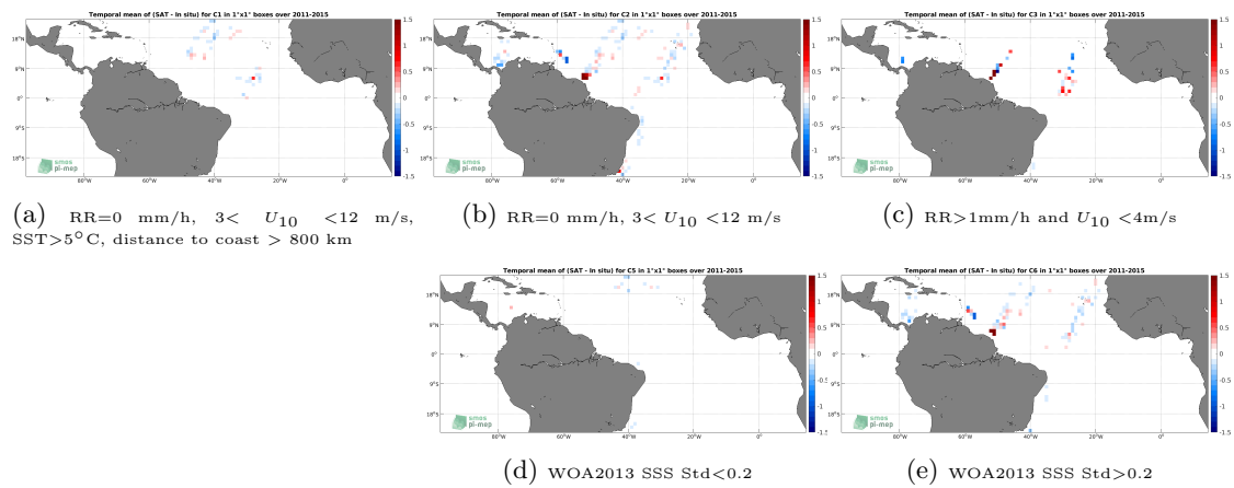
Figure 12: Temporal mean gridded over spatial boxes of size 1^\circ \times 1^\circ of \Delta SSS (Aquarius SSS L4 OI v5 - Monthly (IPRC) - TSG (LEGOS-DM)) for 5 different subdatasets corresponding to:RR=0 mm/h, 3 < U_{10} < 12 m/s, SST > 5^\circ\text{C} , distance to coast > 800 km (a), RR=0 mm/h, 3 < U_{10} < 12 m/s (b), RR > 1 mm/h and U_{10} < 4 m/s (c), WOA2013 SSS Std < 0.2 (d), WOA2013 SSS Std > 0.2 (e).
