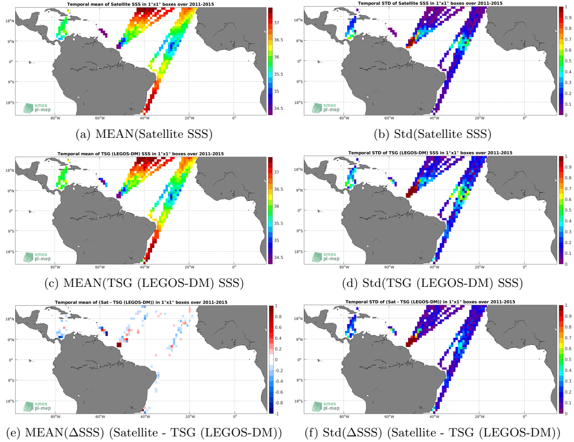
Figure 6: Temporal mean (left) and Std (right) of SSS from Aquarius SSS L4 OI v5 - Monthly (IPRC) (top), TSG (LEGOS-DM) (middle), and of \Delta SSS (Satellite - TSG (LEGOS-DM)). Only match-up pairs are used to generate these maps.
