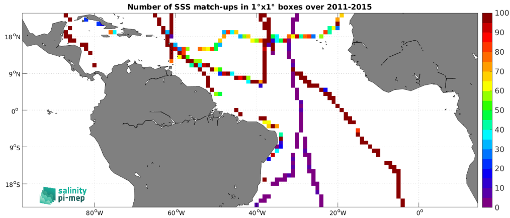
Figure 5: Number of SSS match-ups between TSG (GOSUD-Sailing-ship) SSS and the Aquarius SSS L4 OI v5 - Monthly (IPRC) SSS product for the Tropical Atlantic Ocean Pi-MEP region over 1^\circ \times 1^\circ boxes and for the full satellite product period.
