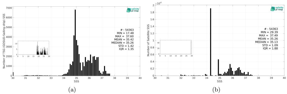
Figure 3: Histograms of SSS from TSG (GOSUD-Sailing-ship) (a) and Aquarius SSS L4 OI v5 - Monthly (IPRC) (b) considering all match-up pairs per bins of 0.1 over the Tropical Atlantic Ocean Pi-MEP region and for the full satellite product period.
