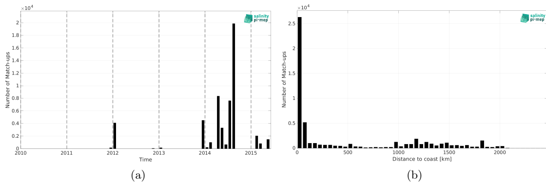
Figure 2: Number of match-ups between TSG (GOSUD-Sailing-ship) and Aquarius SSS L4 OI v5 - Monthly (IPRC) SSS as a function of time (a) and as function of the distance to coast (b) over the Tropical Atlantic Ocean Pi-MEP region and for the full satellite product period.
