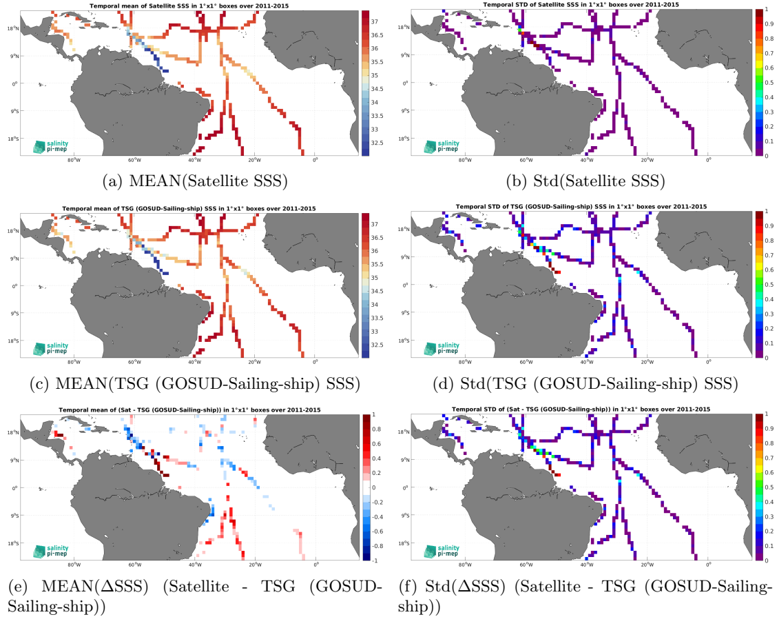
Figure 6: Temporal mean (left) and Std (right) of SSS from Aquarius SSS L4 OI v5 - Monthly (IPRC) (top), TSG (GOSUD-Sailing-ship) (middle), and of \Delta\text{SSS} (Satellite - TSG (GOSUD-Sailing-ship)). Only match-up pairs are used to generate these maps.
