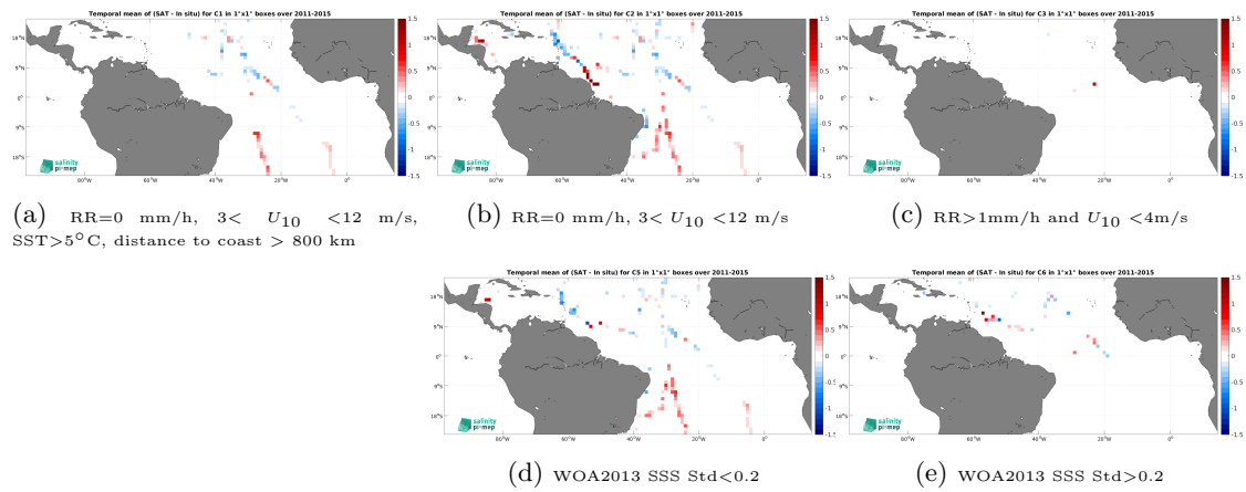
Figure 12: Temporal mean gridded over spatial boxes of size 1^\circ \times 1^\circ of \Delta SSS (Aquarius SSS L4 OI v5 - Monthly (IPRC) - TSG (GOSUD-Sailing-ship)) for 5 different subdatasets corresponding to:RR=0 mm/h, 3 < U_{10} < 12 m/s, SST >5^\circ\text{C} , distance to coast > 800 km (a), RR=0 mm/h, 3 < U_{10} < 12 m/s (b), RR >1 mm/h and U_{10} < 4 m/s (c), WOA2013 SSS Std <0.2 (d), WOA2013 SSS Std >0.2 (e).
