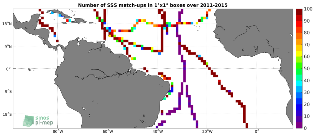
Figure 4: Number of SSS match-ups between TSG-GOSUD-Sailing-ship SSS and the Aquarius-L4-IPRC-V5-MONTHLY SSS product for the Tropical Atlantic Ocean Pi-MEP region over 1°x1° boxes and for the full satellite product period.
