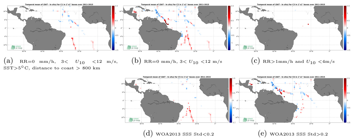
Figure 12: Temporal mean gridded over spatial boxes of size 1^\circ \times 1^\circ of \Delta SSS (Aquarius-L4-IPRC-V5-MONTHLY - TSG-GOSUD-Sailing-ship) for 5 different subdatasets corresponding to:RR=0 mm/h, 3 < U_{10} < 12 m/s, SST>5°C, distance to coast > 800 km (a), RR=0 mm/h, 3 < U_{10} < 12 m/s (b), RR>1mm/h and U_{10} < 4 m/s (c), WOA2013 SSS Std<0.2 (d), WOA2013 SSS Std>0.2 (e).
