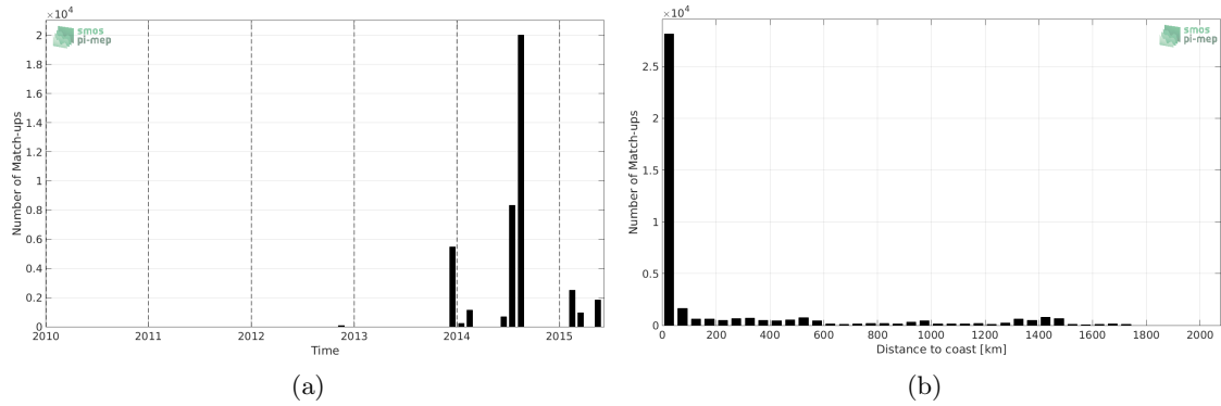
Figure 1: Number of match-ups between TSG-GOSUD-Sailing-ship and Aquarius-L4-IPRC-V5-MONTHLY SSS as a function of time (a) and as function of the distance to coast (b) over the Tropical Atlantic Ocean Pi-MEP region and for the full satellite product period.
