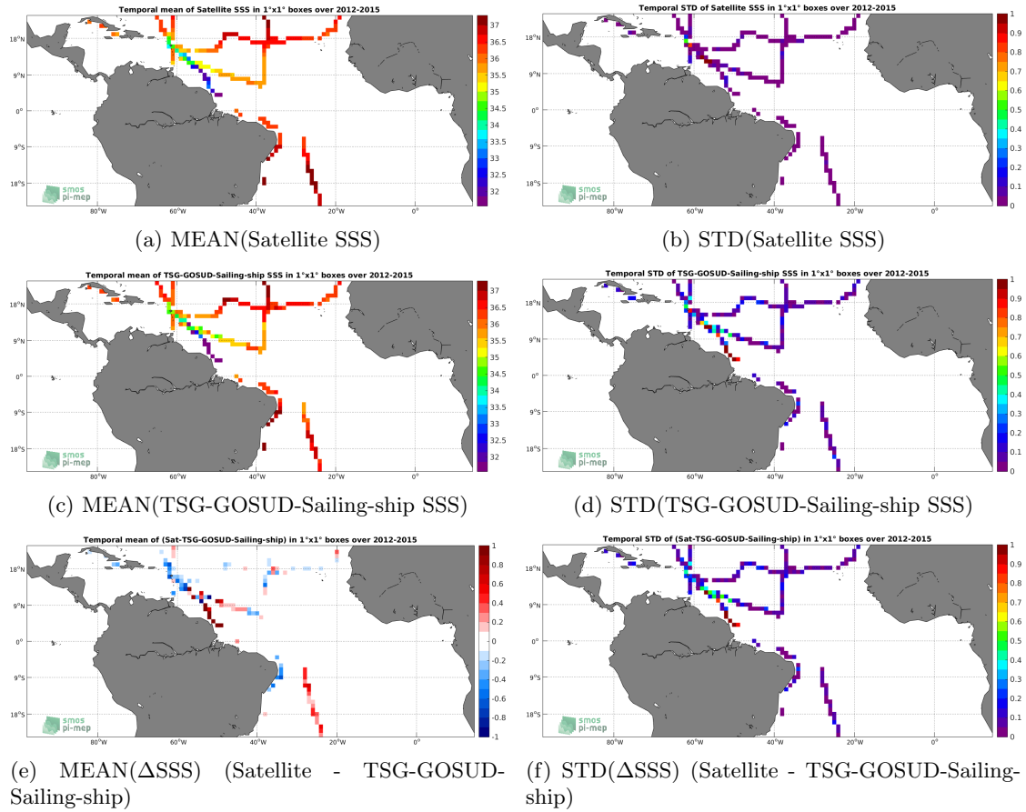
Figure 6: Temporal mean (left) and STD (right) of SSS from Aquarius-L4-IPRC-V5-MONTHLY (top), TSG-GOSUD-Sailing-ship (middle), and of \Delta SSS (Satellite - TSG-GOSUD-Sailing-ship). Only match-up pairs are used to generate these maps.
