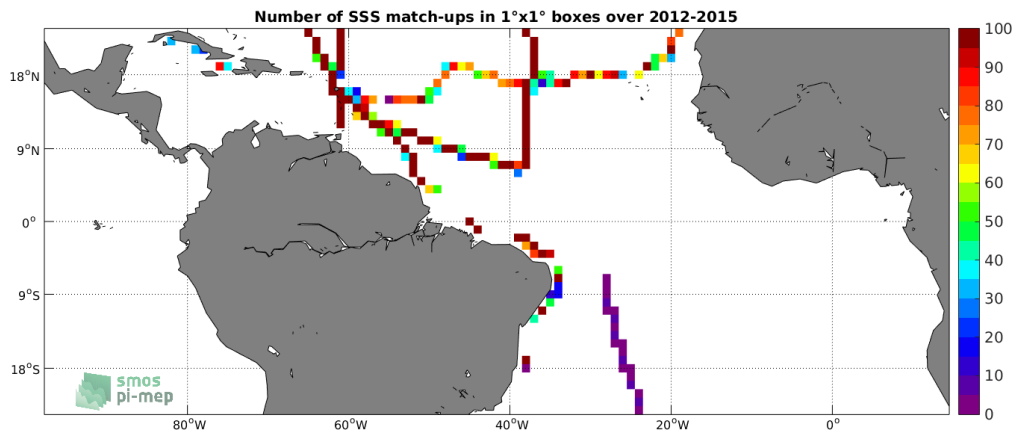
Figure 4: Number of SSS match-ups between TSG-GOSUD-Sailing-ship SSS and the Aquarius-L4-IPRC-V5-MONTHLY SSS product for the Tropical Atlantic Ocean Pi-MEP region over 1^\circ \times 1^\circ boxes and for the full satellite product period.
