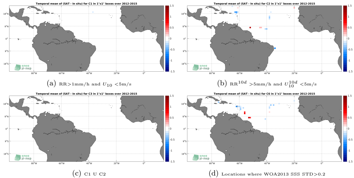
Figure 12: Temporal mean gridded over spatial boxes of size 1^\circ \times 1^\circ of \Delta SSS (Aquarius-L4-IPRC-V5-MONTHLY - TSG-GOSUD-Sailing-ship) for 4 different subdatasets corresponding to: RR > 1mm/h and U_{10} < 5\text{m/s} (a), RR^{10d} > 5\text{mm/h} and U_{10}^{10d} < 5\text{m/s} (b), C1 U C2 (c), Locations where WOA2013 SSS STD > 0.2 (d).
