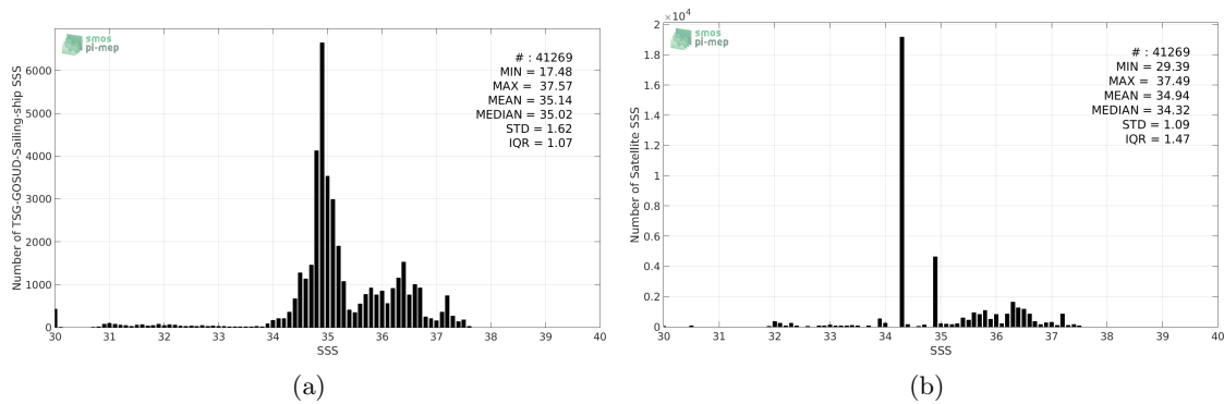
Figure 2: Histograms of SSS from TSG-GOSUD-Sailing-ship (a) and Aquarius-L4-IPRC-V5-MONTHLY (b) considering all match-up pairs per bins of 0.1 over the Tropical Atlantic Ocean Pi-MEP region and for the full satellite product period.
