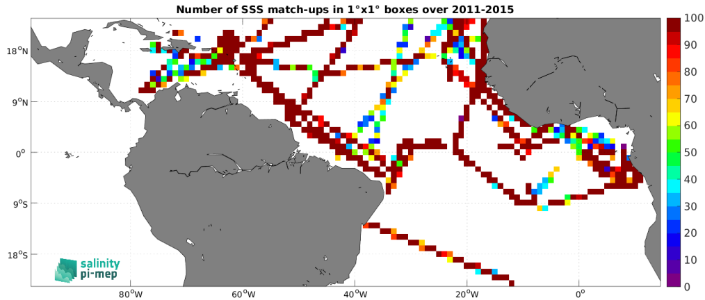
Figure 5: Number of SSS match-ups between TSG (GOSUD-Research-vessel) SSS and the Aquarius SSS L4 OI v5 - Monthly (IPRC) SSS product for the Tropical Atlantic Ocean Pi-MEP region over 1^\circ \times 1^\circ boxes and for the full satellite product period.
