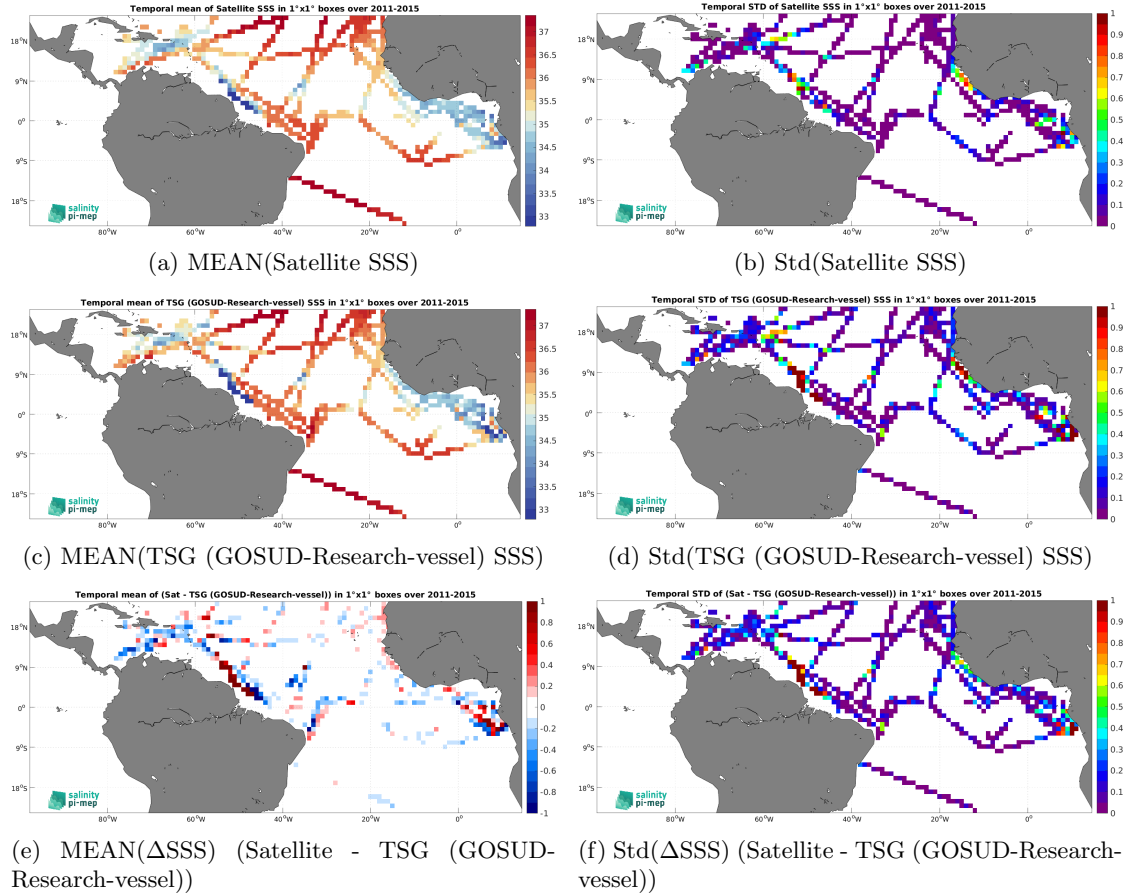
Figure 7: Temporal mean (left) and Std (right) of SSS from Aquarius SSS L4 OI v5 - Monthly (IPRC) (top), TSG (GOSUD-Research-vessel) (middle), and of \Delta\text{SSS} (Satellite - TSG (GOSUD-Research-vessel)). Only match-up pairs are used to generate these maps.
