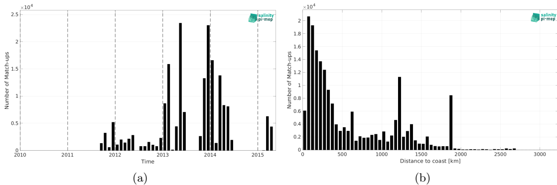
Figure 2: Number of match-ups between TSG (GOSUD-Research-vessel) and Aquarius SSS L4 OI v5 - Monthly (IPRC) SSS as a function of time (a) and as function of the distance to coast (b) over the Tropical Atlantic Ocean Pi-MEP region and for the full satellite product period.
