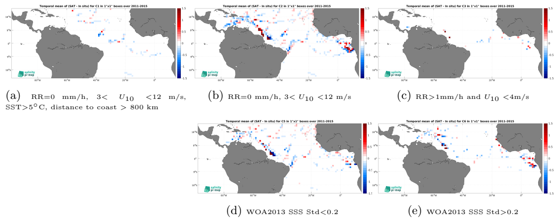
Figure 14: Temporal mean gridded over spatial boxes of size 1^\circ \times 1^\circ of \Delta SSS (Aquarius SSS L4 OI v5 - Monthly (IPRC) - TSG (GOSUD-Research-vessel)) for 5 different subdatasets corresponding to:RR=0 mm/h, 3 < U_{10} < 12 m/s, SST >5^\circ\text{C} , distance to coast > 800 km (a), RR=0 mm/h, 3 < U_{10} < 12 m/s (b), RR >1 mm/h and U_{10} < 4 m/s (c), WOA2013 SSS Std <0.2 (d), WOA2013 SSS Std >0.2 (e).
