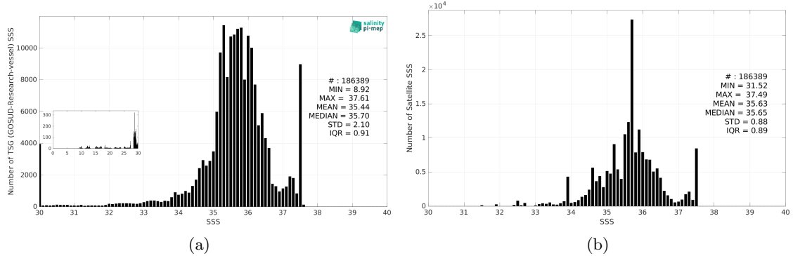
Figure 3: Histograms of SSS from TSG (GOSUD-Research-vessel) (a) and Aquarius SSS L4 OI v5 - Monthly (IPRC) (b) considering all match-up pairs per bins of 0.1 over the Tropical Atlantic Ocean Pi-MEP region and for the full satellite product period.
