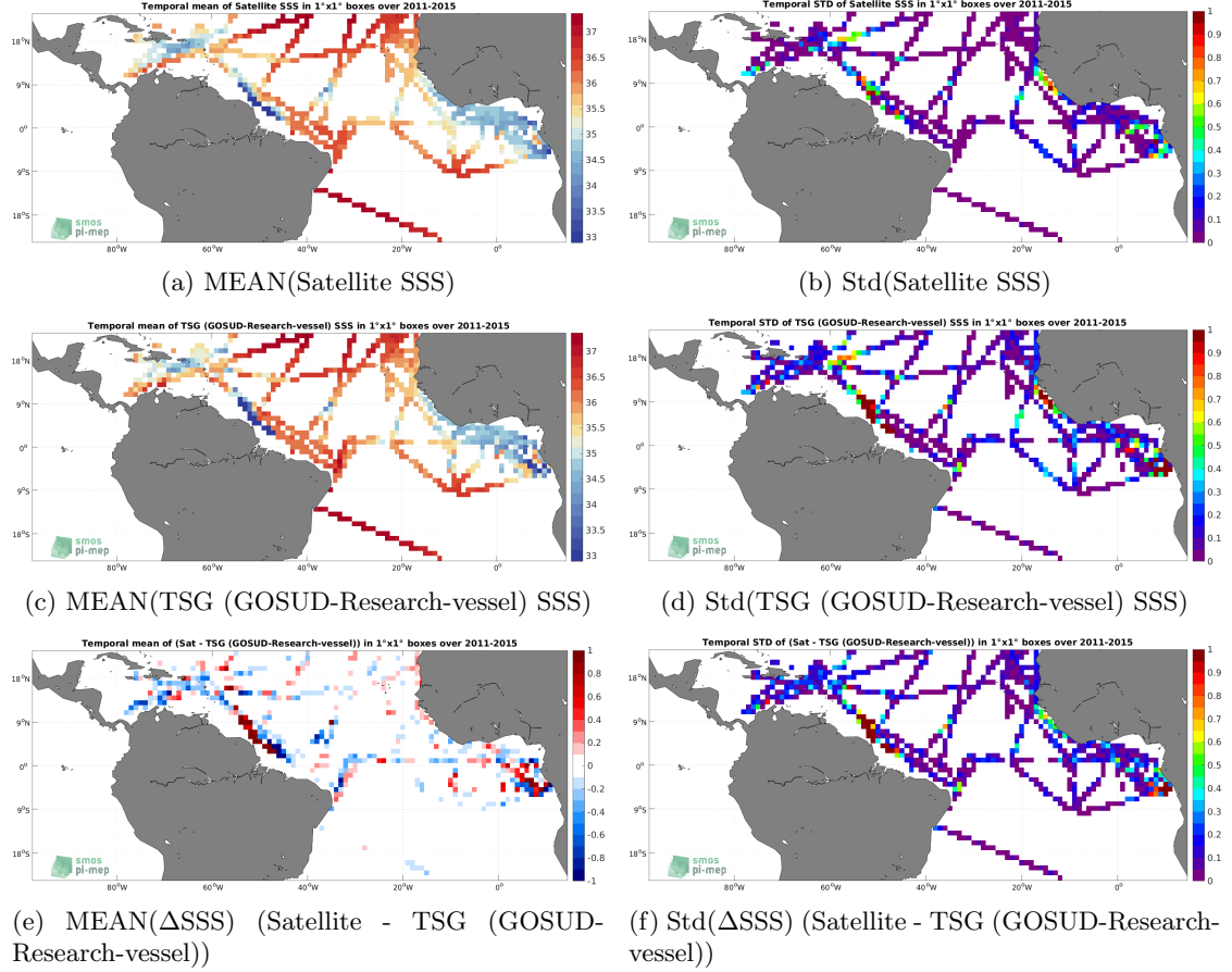
Figure 6: Temporal mean (left) and Std (right) of SSS from Aquarius SSS L4 OI v5 - Monthly (IPRC) (top), TSG (GOSUD-Research-vessel) (middle), and of \Delta\text{SSS} (Satellite - TSG (GOSUD-Research-vessel)). Only match-up pairs are used to generate these maps.
