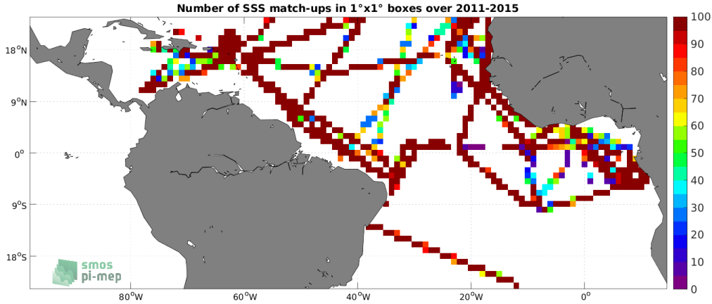
Figure 4: Number of SSS match-ups between TSG (GOSUD-Research-vessel) SSS and the Aquarius SSS L4 OI v5 - Monthly (IPRC) SSS product for the Tropical Atlantic Ocean Pi-MEP region over 1^\circ \times 1^\circ boxes and for the full satellite product period.
