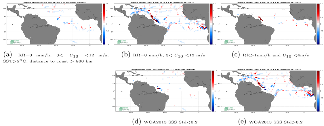
Figure 12: Temporal mean gridded over spatial boxes of size 1^\circ \times 1^\circ of \Delta SSS (Aquarius SSS L4 OI v5 - Monthly (IPRC) - TSG (GOSUD-Research-vessel)) for 5 different subdatasets corresponding to: RR=0 mm/h, 3 < U_{10} < 12 m/s, SST >5^\circ\text{C} , distance to coast > 800 km (a), RR=0 mm/h, 3 < U_{10} < 12 m/s (b), RR >1 mm/h and U_{10} < 4 m/s (c), WOA2013 SSS Std <0.2 (d), WOA2013 SSS Std >0.2 (e).
