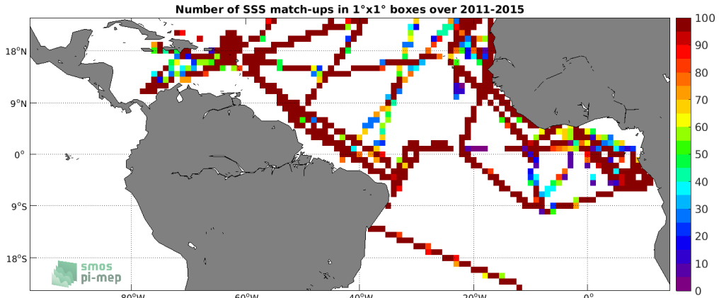
Figure 4: Number of SSS match-ups between TSG (GOSUD-Research-vessel) SSS and the Aquarius SSS L4 OI v5 - Monthly (IPRC) SSS product for the Tropical Atlantic Ocean Pi-MEP region over 1^\circ \times 1^\circ boxes and for the full satellite product period.
