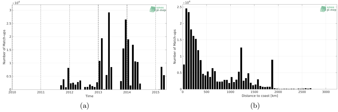
Figure 1: Number of match-ups between TSG (GOSUD-Research-vessel) and Aquarius SSS L4 OI v5 - Monthly (IPRC) SSS as a function of time (a) and as function of the distance to coast (b) over the Tropical Atlantic Ocean Pi-MEP region and for the full satellite product period.
