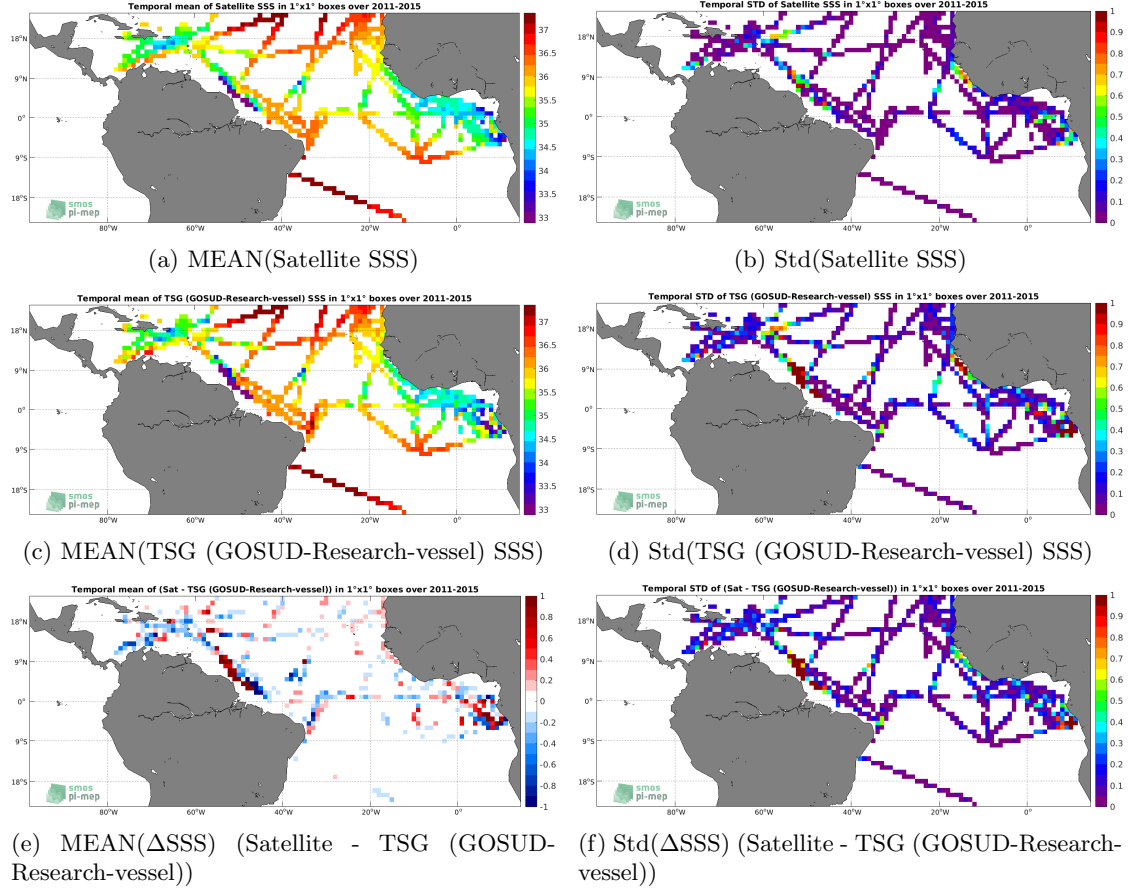
Figure 6: Temporal mean (left) and Std (right) of SSS from Aquarius SSS L4 OI v5 - Monthly (IPRC) (top), TSG (GOSUD-Research-vessel) (middle), and of \Delta SSS (Satellite - TSG (GOSUD-Research-vessel)). Only match-up pairs are used to generate these maps.
