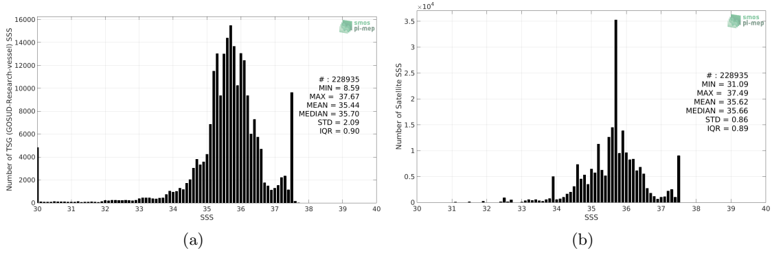
Figure 2: Histograms of SSS from TSG (GOSUD-Research-vessel) (a) and Aquarius SSS L4 OI v5 - Monthly (IPRC) (b) considering all match-up pairs per bins of 0.1 over the Tropical Atlantic Ocean Pi-MEP region and for the full satellite product period.
