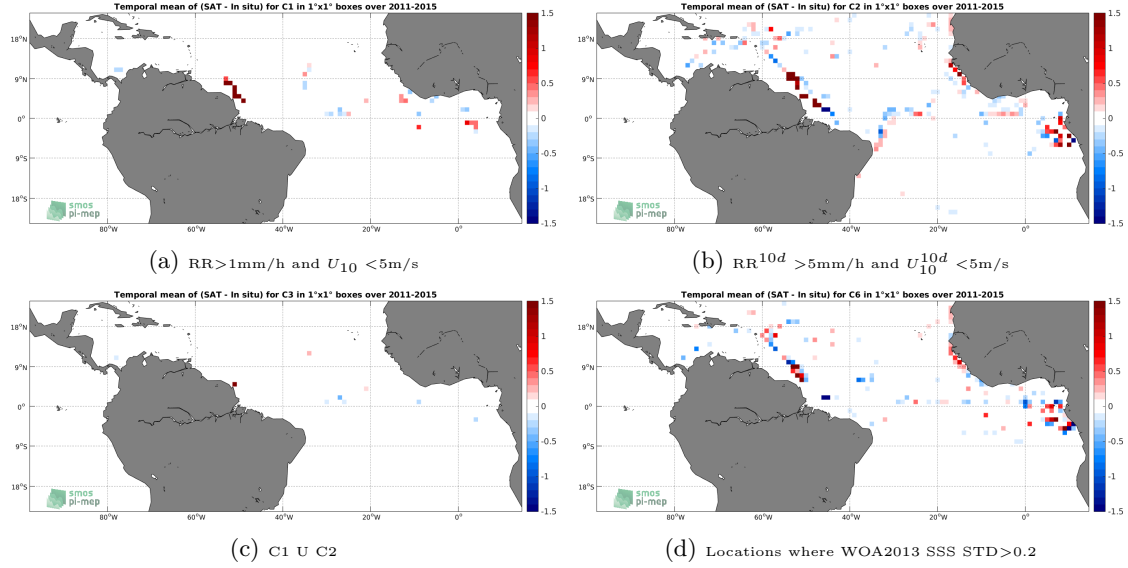
Figure 12: Temporal mean gridded over spatial boxes of size 1^\circ \times 1^\circ of \Delta SSS (Aquarius-L4-IPRC-V5-MONTHLY - TSG-GOSUD-Research-vessel) for 4 different subdatasets corresponding to: RR > 1mm/h and U_{10} < 5\text{m/s} (a), RR^{10d} > 5\text{mm/h} and U_{10}^{10d} < 5\text{m/s} (b), C1 U C2 (c), Locations where WOA2013 SSS STD > 0.2 (d).
