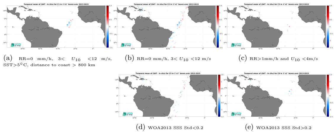
Figure 14: Temporal mean gridded over spatial boxes of size 1^\circ \times 1^\circ of \Delta SSS (Aquarius SSS L4 OI v5 - Monthly (IPRC) - TSG (CSIC-UTM)) for 5 different subdatasets corresponding to:RR=0 mm/h, 3 < U_{10} < 12 m/s, SST >5^\circ\text{C} , distance to coast > 800 km (a), RR=0 mm/h, 3 < U_{10} < 12 m/s (b), RR >1 mm/h and U_{10} < 4 m/s (c), WOA2013 SSS Std <0.2 (d), WOA2013 SSS Std >0.2 (e).
