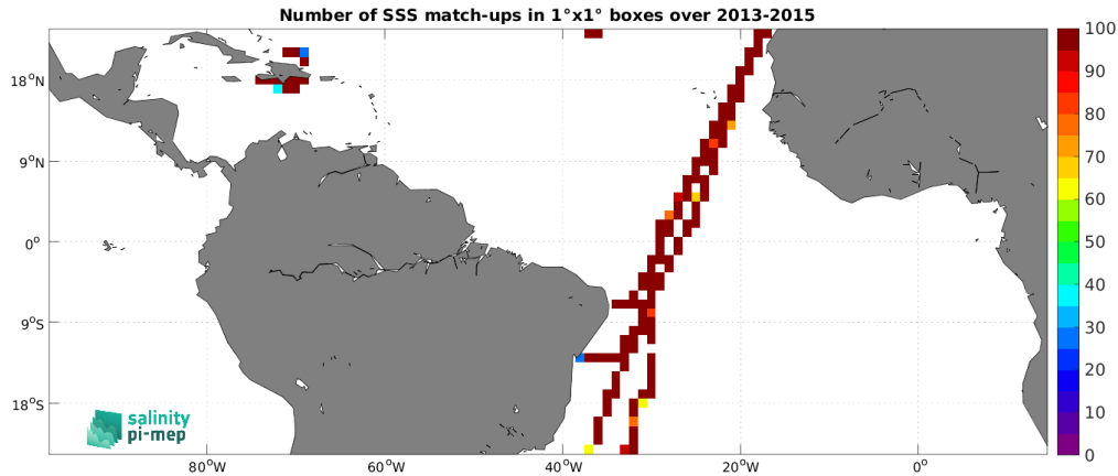
Figure 5: Number of SSS match-ups between TSG (CSIC-UTM) SSS and the Aquarius SSS L4 OI v5 - Monthly (IPRC) SSS product for the Tropical Atlantic Ocean Pi-MEP region over 1^\circ \times 1^\circ boxes and for the full satellite product period.
