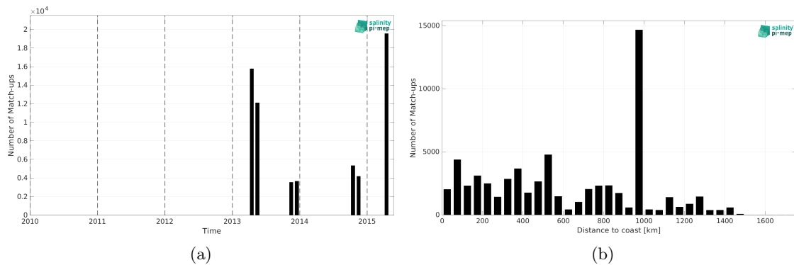
Figure 2: Number of match-ups between TSG (CSIC-UTM) and Aquarius SSS L4 OI v5 - Monthly (IPRC) SSS as a function of time (a) and as function of the distance to coast (b) over the Tropical Atlantic Ocean Pi-MEP region and for the full satellite product period.
