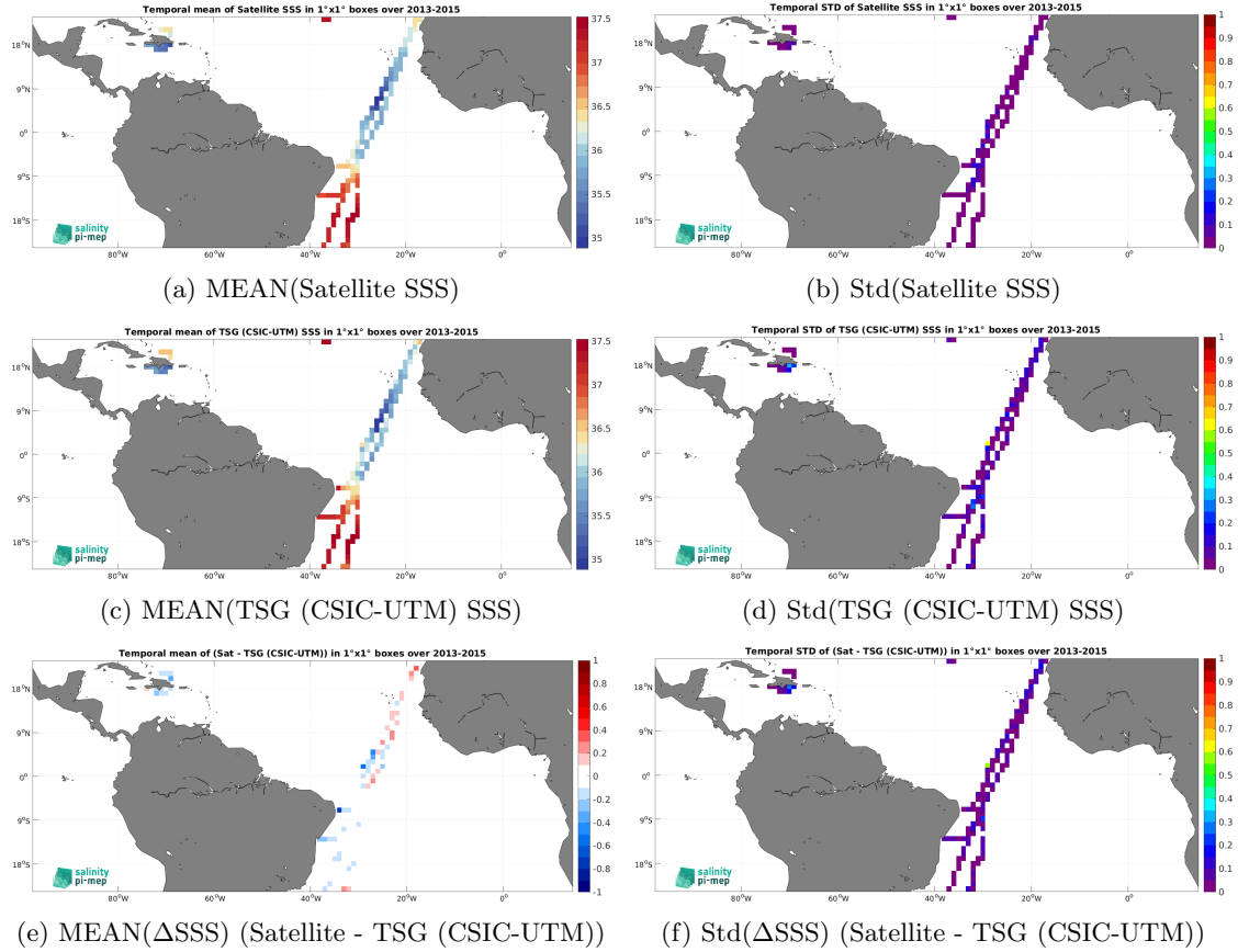
Figure 7: Temporal mean (left) and Std (right) of SSS from Aquarius SSS L4 OI v5 - Monthly (IPRC) (top), TSG (CSIC-UTM) (middle), and of \Delta\text{SSS} (Satellite - TSG (CSIC-UTM)). Only match-up pairs are used to generate these maps.
