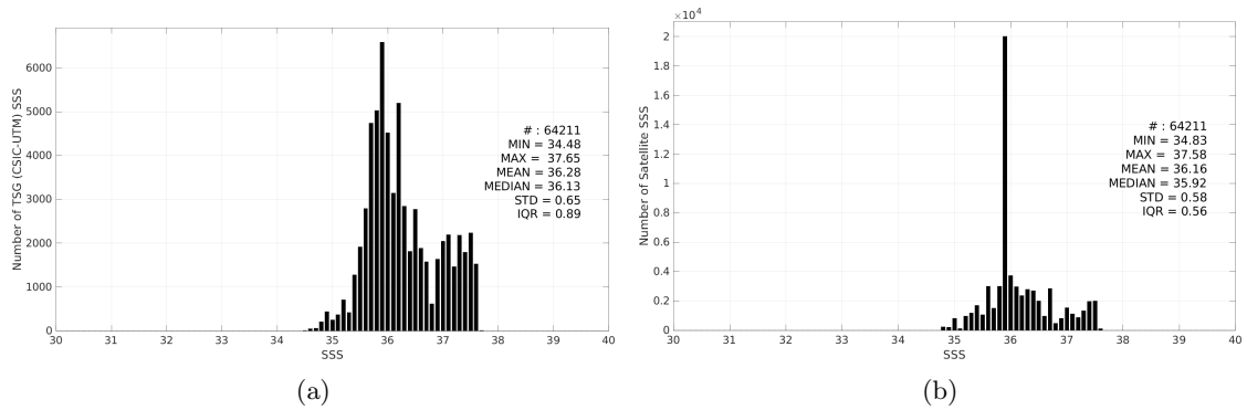
Figure 3: Histograms of SSS from TSG (CSIC-UTM) (a) and Aquarius SSS L4 OI v5 - Monthly (IPRC) (b) considering all match-up pairs per bins of 0.1 over the Tropical Atlantic Ocean Pi-MEP region and for the full satellite product period.
