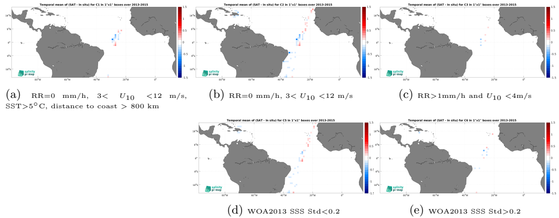
Figure 12: Temporal mean gridded over spatial boxes of size 1^\circ \times 1^\circ of \Delta SSS (Aquarius SSS L4 OI v5 - Monthly (IPRC) - TSG (CSIC-UTM)) for 5 different subdatasets corresponding to:RR=0 mm/h, 3 < U_{10} < 12 m/s, SST >5^\circ\text{C} , distance to coast > 800 km (a), RR=0 mm/h, 3 < U_{10} < 12 m/s (b), RR >1 mm/h and U_{10} < 4 m/s (c), WOA2013 SSS Std <0.2 (d), WOA2013 SSS Std >0.2 (e).
