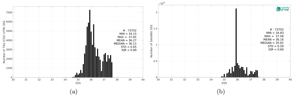
Figure 2: Histograms of SSS from TSG (CSIC-UTM) (a) and Aquarius SSS L4 OI v5 - Monthly (IPRC) (b) considering all match-up pairs per bins of 0.1 over the Tropical Atlantic Ocean Pi-MEP region and for the full satellite product period.
