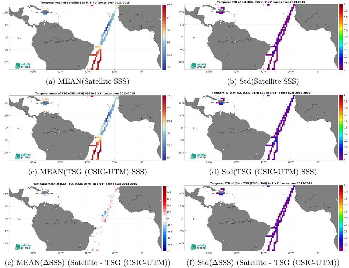
Figure 6: Temporal mean (left) and Std (right) of SSS from Aquarius SSS L4 OI v5 - Monthly (IPRC) (top), TSG (CSIC-UTM) (middle), and of \Delta\text{SSS} (Satellite - TSG (CSIC-UTM)). Only match-up pairs are used to generate these maps.
