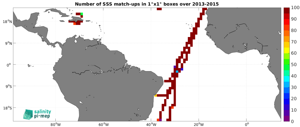
Figure 4: Number of SSS match-ups between TSG (CSIC-UTM) SSS and the Aquarius SSS L4 OI v5 - Monthly (IPRC) SSS product for the Tropical Atlantic Ocean Pi-MEP region over 1^\circ \times 1^\circ boxes and for the full satellite product period.
