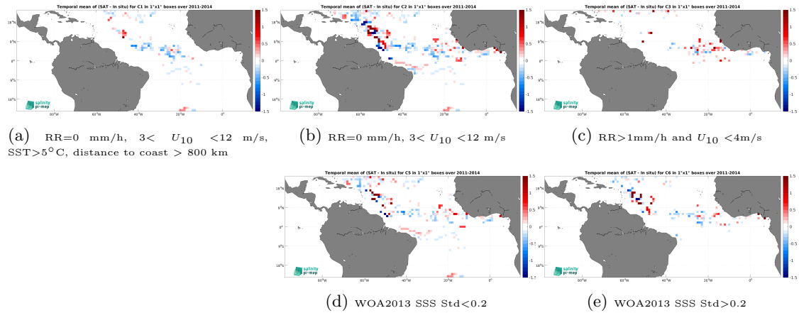
Figure 13: Temporal mean gridded over spatial boxes of size 1^\circ \times 1^\circ of \Delta\text{SSS} (Aquarius SSS L4 OI v5 - Monthly (IPRC) - Surface drifters) for 5 different subdatasets corresponding to:RR=0 mm/h, 3 < U_{10} < 12 m/s, SST >5^\circ\text{C} , distance to coast > 800 km (a), RR=0 mm/h, 3 < U_{10} < 12 m/s (b), RR >1 mm/h and U_{10} < 4 m/s (c), WOA2013 SSS Std <0.2 (d), WOA2013 SSS Std >0.2 (e).
