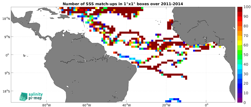
Figure 4: Number of SSS match-ups between Surface drifters SSS and the Aquarius SSS L4 OI v5 - Monthly (IPRC) SSS product for the Tropical Atlantic Ocean Pi-MEP region over 1^\circ \times 1^\circ boxes and for the full satellite product period.
