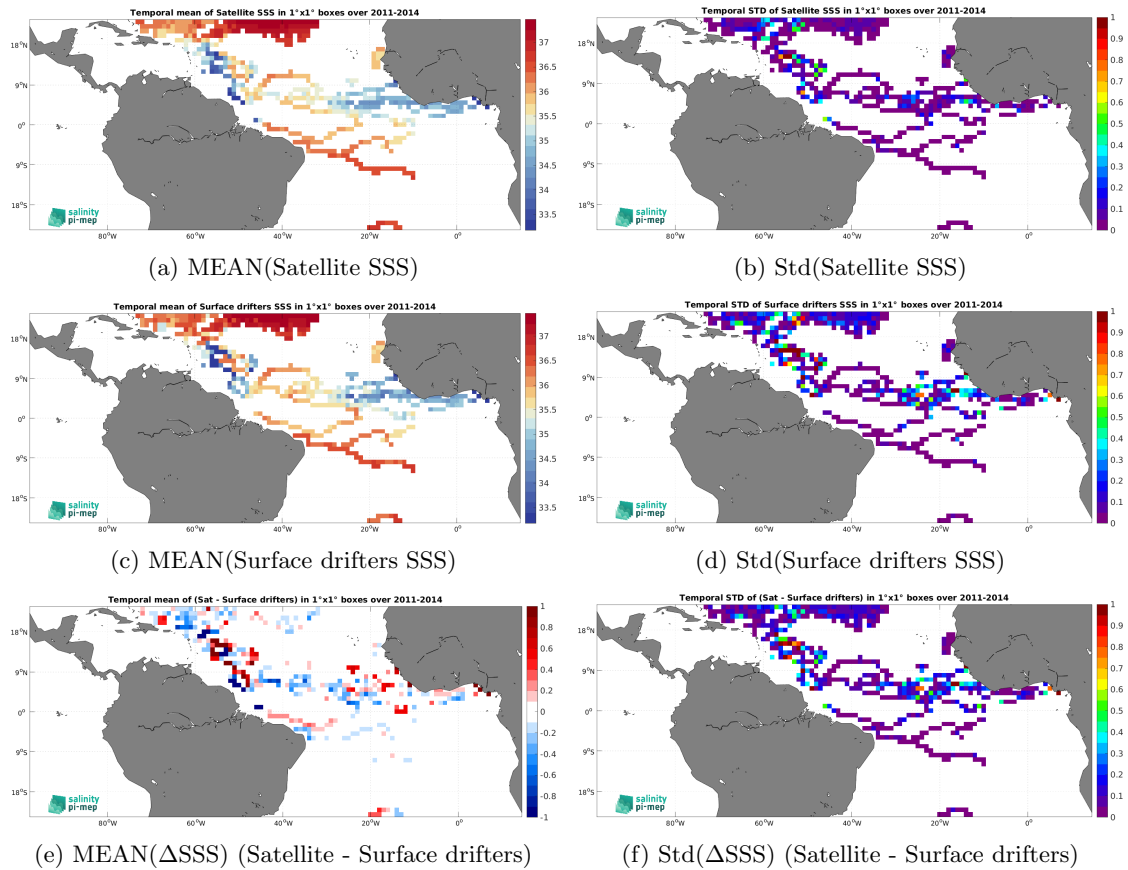
Figure 6: Temporal mean (left) and Std (right) of SSS from Aquarius SSS L4 OI v5 - Monthly (IPRC) (top), Surface drifters (middle), and of \Delta SSS (Satellite - Surface drifters). Only match-up pairs are used to generate these maps.
