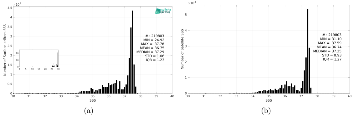
Figure 3: Histograms of SSS from Surface drifters (a) and Aquarius SSS L4 OI v5 - Monthly (IPRC) (b) considering all match-up pairs per bins of 0.1 over the Tropical Atlantic Ocean Pi-MEP region and for the full satellite product period.
