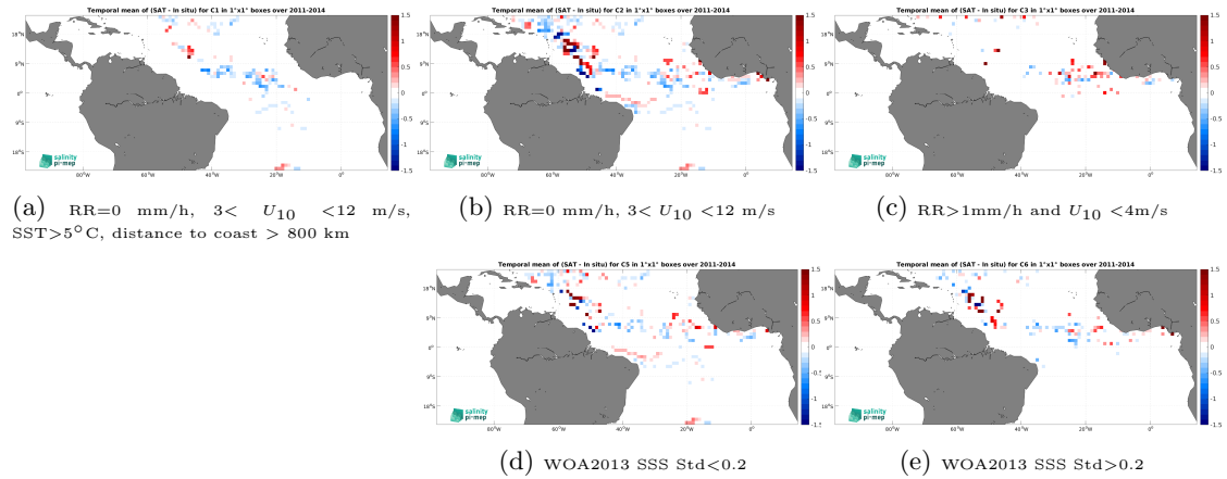
Figure 13: Temporal mean gridded over spatial boxes of size 1^\circ \times 1^\circ of \Delta SSS (Aquarius SSS L4 OI v5 - Monthly (IPRC) - Surface drifters) for 5 different subdatasets corresponding to:RR=0 mm/h, 3 < U_{10} < 12 m/s, SST >5^\circ\text{C} , distance to coast > 800 km (a), RR=0 mm/h, 3 < U_{10} < 12 m/s (b), RR >1 mm/h and U_{10} < 4 m/s (c), WOA2013 SSS Std <0.2 (d), WOA2013 SSS Std >0.2 (e).
