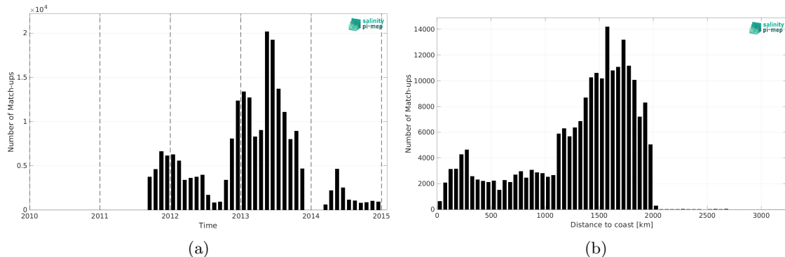
Figure 2: Number of match-ups between Surface drifters and Aquarius SSS L4 OI v5 - Monthly (IPRC) SSS as a function of time (a) and as function of the distance to coast (b) over the Tropical Atlantic Ocean Pi-MEP region and for the full satellite product period.
