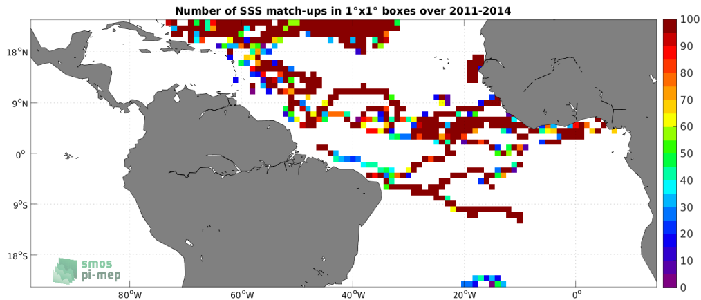
Figure 3: Number of SSS match-ups between Surface drifters SSS and the Aquarius SSS L4 OI v5 - Monthly (IPRC) SSS product for the Tropical Atlantic Ocean Pi-MEP region over 1^\circ \times 1^\circ boxes and for the full satellite product period.
