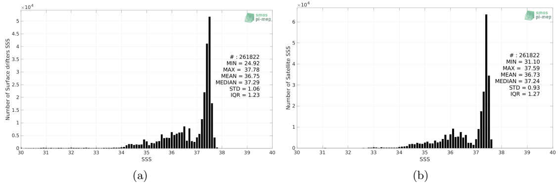
Figure 2: Histograms of SSS from Surface drifters (a) and Aquarius SSS L4 OI v5 - Monthly (IPRC) (b) considering all match-up pairs per bins of 0.1 over the Tropical Atlantic Ocean Pi-MEP region and for the full satellite product period.
