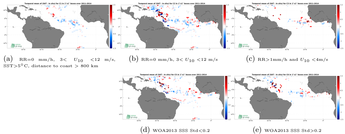
Figure 11: Temporal mean gridded over spatial boxes of size 1^\circ \times 1^\circ of \Delta SSS (Aquarius SSS L4 OI v5 - Monthly (IPRC) - Surface drifters) for 5 different subdatasets corresponding to:RR=0 mm/h, 3 < U_{10} < 12 m/s, SST >5^\circ\text{C} , distance to coast > 800 km (a), RR=0 mm/h, 3 < U_{10} < 12 m/s (b), RR >1 mm/h and U_{10} < 4 m/s (c), WOA2013 SSS Std <0.2 (d), WOA2013 SSS Std >0.2 (e).
