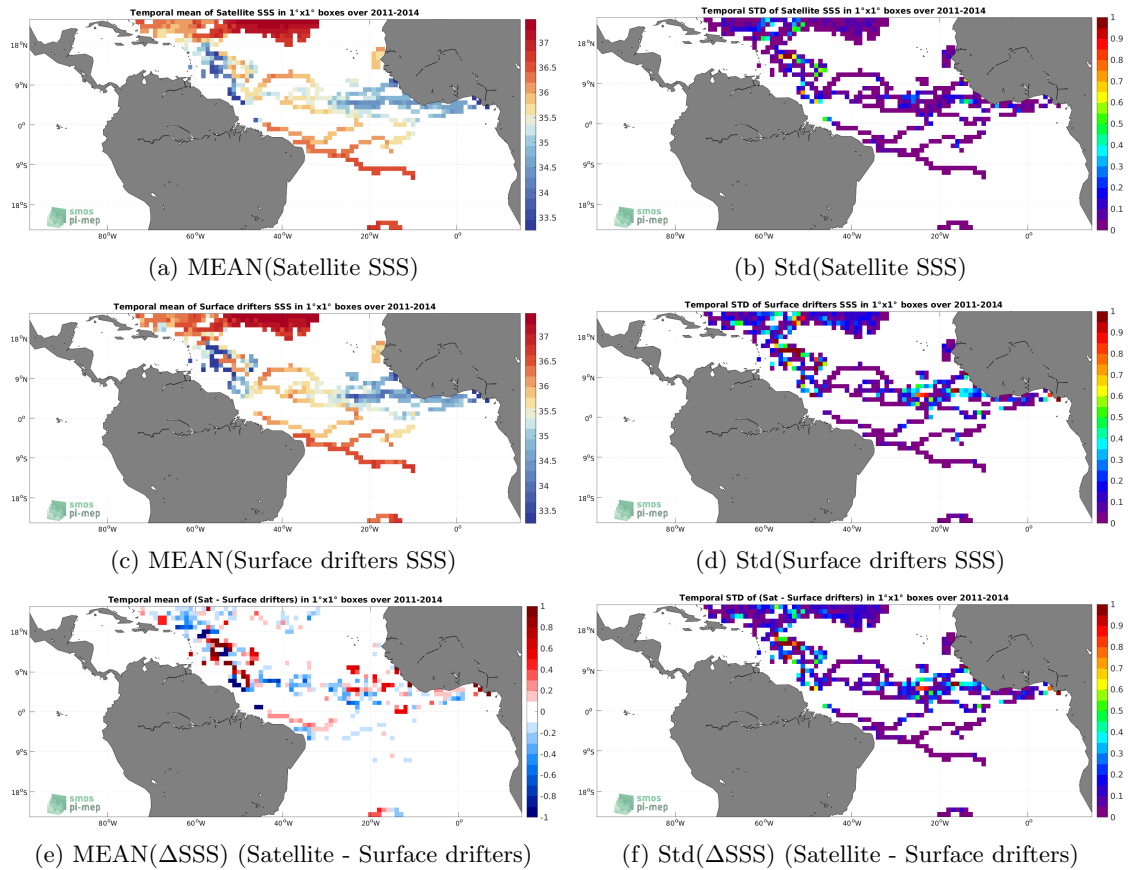
Figure 5: Temporal mean (left) and Std (right) of SSS from Aquarius SSS L4 OI v5 - Monthly (IPRC) (top), Surface drifters (middle), and of \Delta SSS (Satellite - Surface drifters). Only match-up pairs are used to generate these maps.
