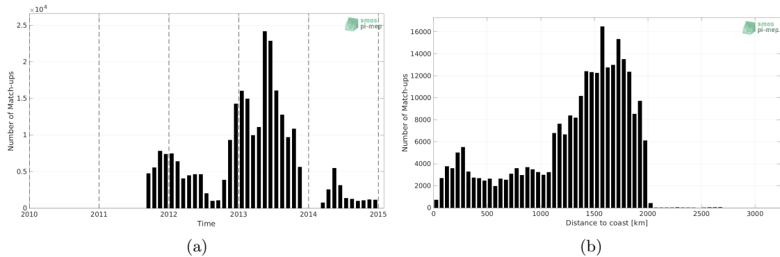
Figure 1: Number of match-ups between Surface drifters and Aquarius SSS L4 OI v5 - Monthly (IPRC) SSS as a function of time (a) and as function of the distance to coast (b) over the Tropical Atlantic Ocean Pi-MEP region and for the full satellite product period.
