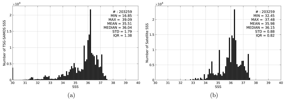
Figure 2: Histograms of SSS from TSG-SAMOS (a) and Aquarius-L4-IPRC-V4-WEEKLY (b) considering all match-up pairs per bins of 0.1 over the Tropical Atlantic Ocean Pi-MEP region and for the full satellite product period.
