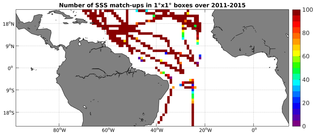
Figure 4: Number of SSS match-ups between TSG-SAMOS SSS and the Aquarius-L4-IPRC-V4-WEEKLY SSS product for the Tropical Atlantic Ocean Pi-MEP region over 1^\circ \times 1^\circ boxes and for the full satellite product period.
