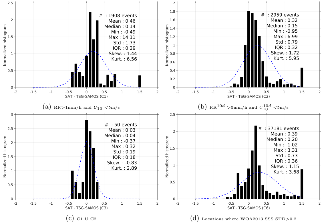
Figure 13: Normalized histogram of \Delta\text{SSS} (Aquarius-L4-IPRC-V4-WEEKLY - TSG-SAMOS) for 6 different subdatasets corresponding to: RR > 1mm/h and U_{10} < 5\text{m/s} (a), RR^{10d} > 5\text{mm/h} and U_{10}^{10d} < 5\text{m/s} (b), C1 U C2 (c), Locations where WOA2013 SSS STD > 0.2 (d).
