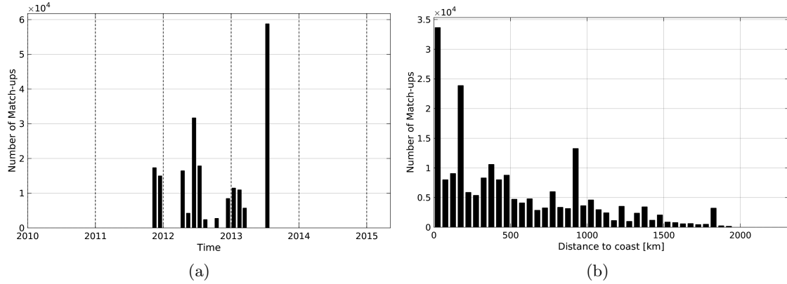
Figure 1: Number of match-ups between TSG-SAMOS and Aquarius-L4-IPRC-V4-WEEKLY SSS as a function of time (a) and as function of the distance to coast (b) over the Tropical Atlantic Ocean Pi-MEP region and for the full satellite product period.
