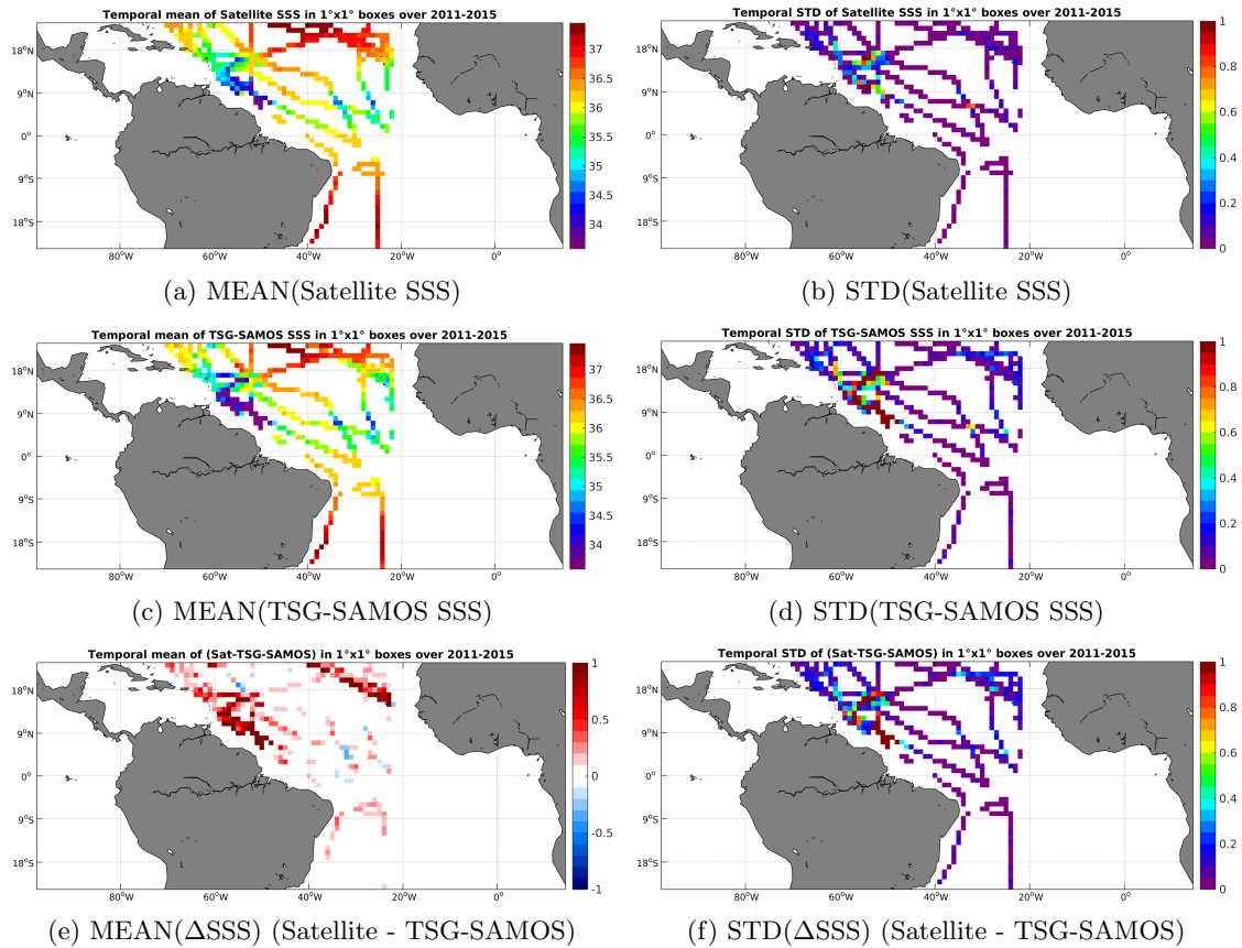
Figure 6: Temporal mean (left) and STD (right) of SSS from Aquarius-L4-IPRC-V4-WEEKLY (top), TSG-SAMOS (middle), and of \Delta SSS (Satellite - TSG-SAMOS). Only match-up pairs are used to generate these maps.
