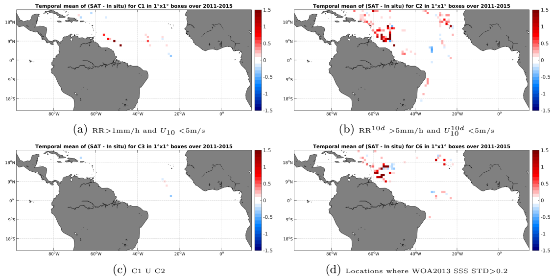
Figure 12: Temporal mean gridded over spatial boxes of size 1^\circ \times 1^\circ of \Delta SSS (Aquarius-L4-IPRC-V4-WEEKLY - TSG-SAMOS) for 4 different subdatasets corresponding to:RR >1 mm/h and U_{10} < 5 m/s (a), RR 10d > 5 mm/h and U_{10}^{10d} < 5 m/s (b), C1 U C2 (c),Locations where WOA2013 SSS STD >0.2 (d).
