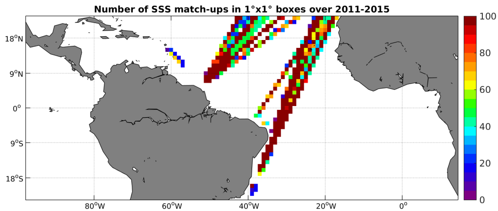
Figure 4: Number of SSS match-ups between TSG-LEGOS-DM SSS and the Aquarius-L4-IPRC-V4-WEEKLY SSS product for the Tropical Atlantic Ocean Pi-MEP region over 1°x1° boxes and for the full satellite product period.
