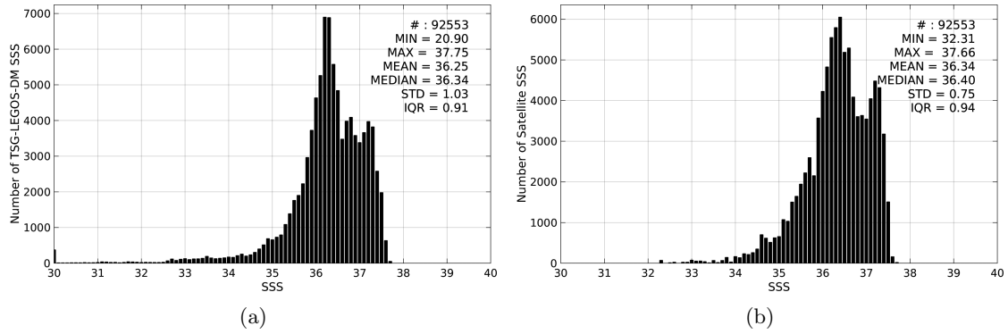
Figure 2: Histograms of SSS from TSG-LEGOS-DM (a) and Aquarius-L4-IPRC-V4-WEEKLY (b) considering all match-up pairs per bins of 0.1 over the Tropical Atlantic Ocean Pi-MEP region and for the full satellite product period.
