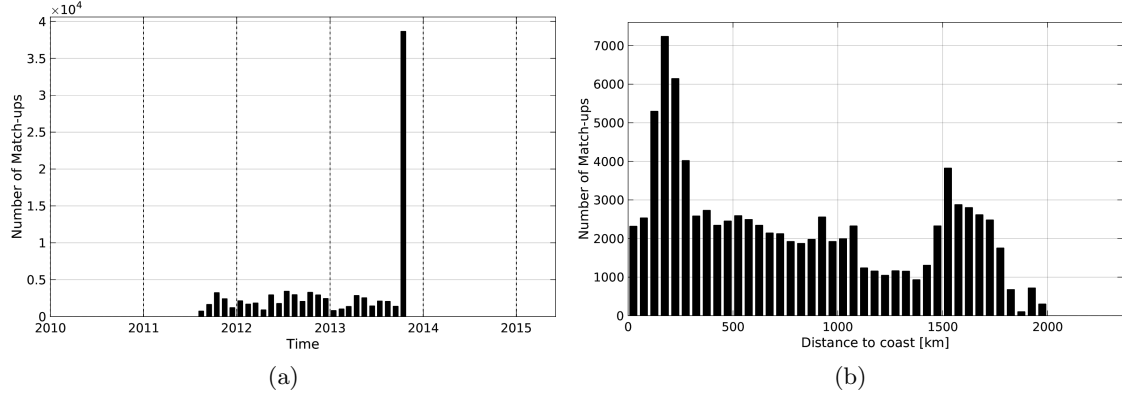
Figure 1: Number of match-ups between TSG-LEGOS-DM and Aquarius-L4-IPRC-V4-WEEKLY SSS as a function of time (a) and as function of the distance to coast (b) over the Tropical Atlantic Ocean Pi-MEP region and for the full satellite product period.
