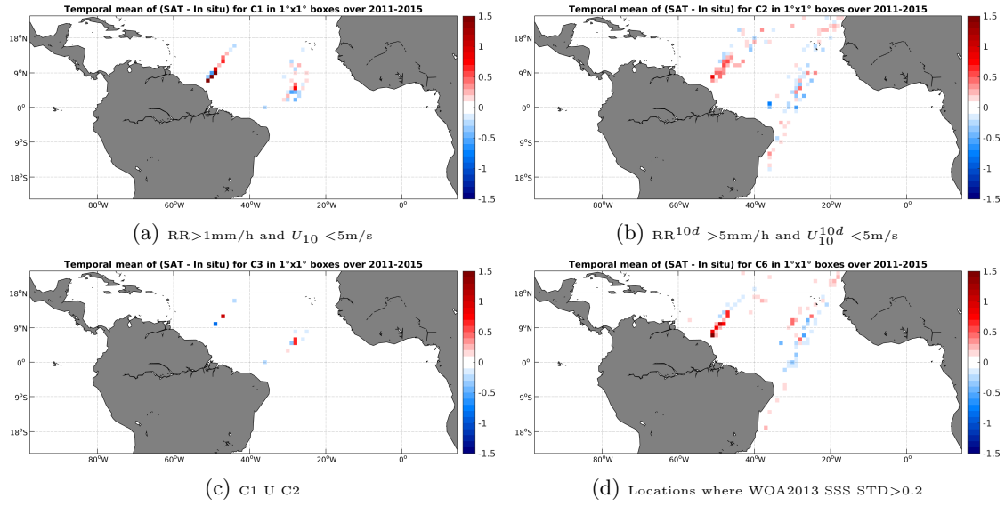
Figure 12: Temporal mean gridded over spatial boxes of size 1^\circ \times 1^\circ of \Delta SSS (Aquarius-L4-IPRC-V4-WEEKLY - TSG-LEGOS-DM) for 4 different subdatasets corresponding to: RR > 1 mm/h and U_{10} < 5 m/s (a), RR^{10d} > 5 mm/h and U_{10}^{10d} < 5 m/s (b), C1 U C2 (c), Locations where WOA2013 SSS STD > 0.2 (d).
