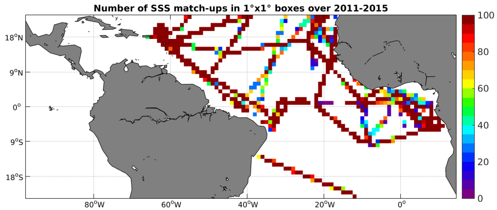
Figure 4: Number of SSS match-ups between TSG-GOSUD-Research-vessel SSS and the Aquarius-L4-IPRC-V4-WEEKLY SSS product for the Tropical Atlantic Ocean Pi-MEP region over 1^\circ \times 1^\circ boxes and for the full satellite product period.
