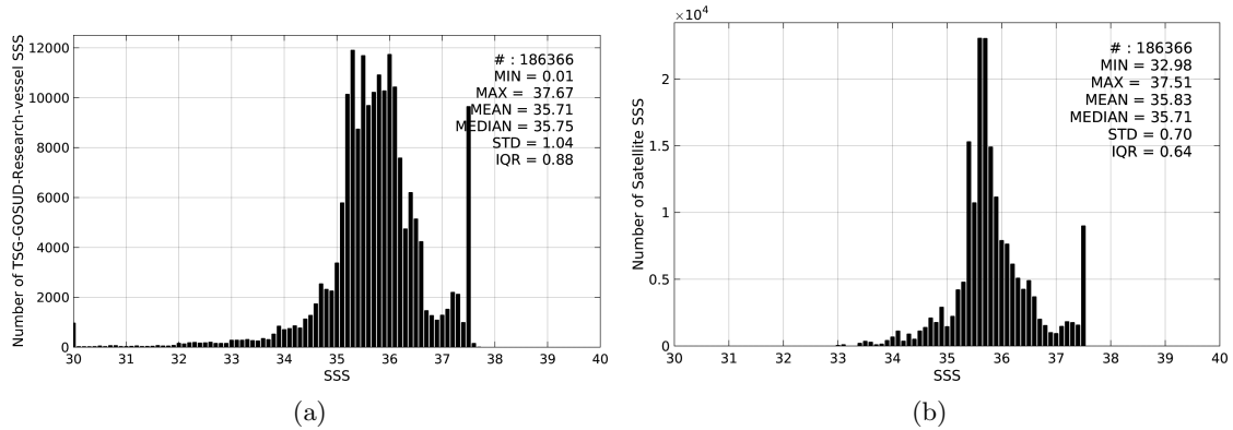
Figure 2: Histograms of SSS from TSG-GOSUD-Research-vessel (a) and Aquarius-L4-IPRC-V4-WEEKLY (b) considering all match-up pairs per bins of 0.1 over the Tropical Atlantic Ocean Pi-MEP region and for the full satellite product period.
