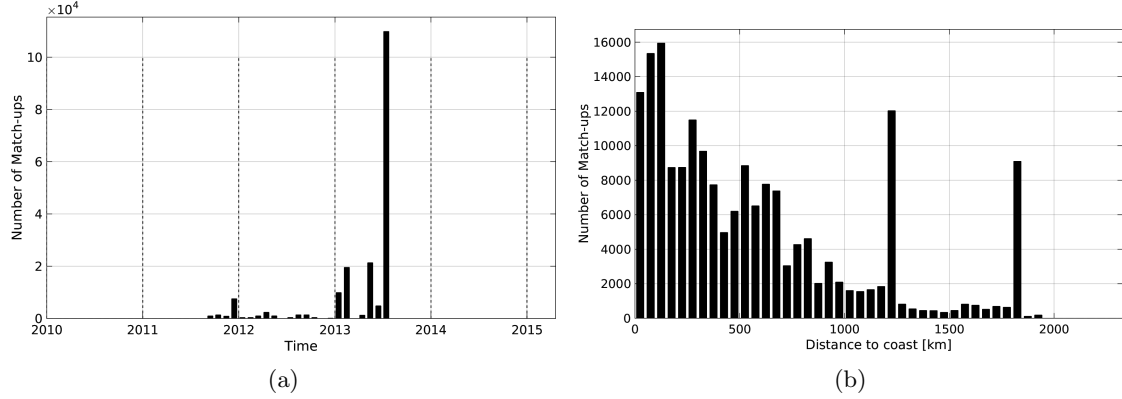
Figure 1: Number of match-ups between TSG-GOSUD-Research-vessel and Aquarius-L4-IPRC-V4-WEEKLY SSS as a function of time (a) and as function of the distance to coast (b) over the Tropical Atlantic Ocean Pi-MEP region and for the full satellite product period.
