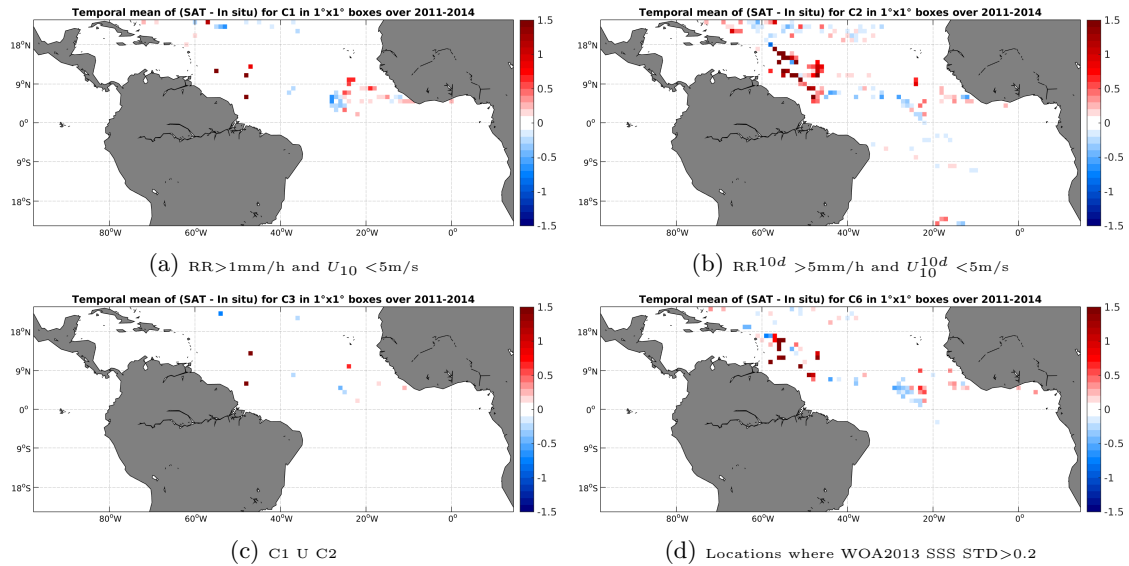
Figure 11: Temporal mean gridded over spatial boxes of size 1^\circ \times 1^\circ of \Delta SSS (Aquarius-L4-IPRC-V4-WEEKLY - Surface drifters) for 4 different subdatasets corresponding to: RR > 1\text{mm/h} and U_{10} < 5\text{m/s} (a), RR^{10d} > 5\text{mm/h} and U_{10}^{10d} < 5\text{m/s} (b), C1 U C2 (c), Locations where WOA2013 SSS STD > 0.2 (d).
