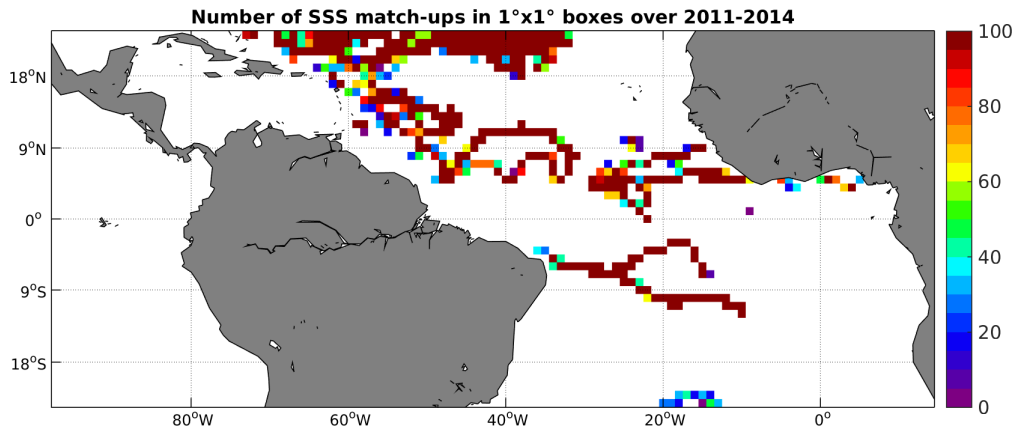
Figure 3: Number of SSS match-ups between Surface drifters SSS and the Aquarius-L4-IPRC-V4-WEEKLY SSS product for the Tropical Atlantic Ocean Pi-MEP region over 1^\circ \times 1^\circ boxes and for the full satellite product period.
