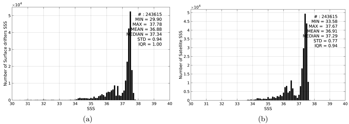
Figure 2: Histograms of SSS from Surface drifters (a) and Aquarius-L4-IPRC-V4-WEEKLY (b) considering all match-up pairs per bins of 0.1 over the Tropical Atlantic Ocean Pi-MEP region and for the full satellite product period.
