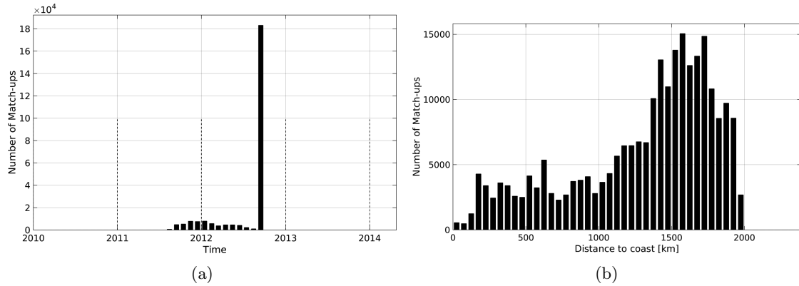
Figure 1: Number of match-ups between Surface drifters and Aquarius-L4-IPRC-V4-WEEKLY SSS as a function of time (a) and as function of the distance to coast (b) over the Tropical Atlantic Ocean Pi-MEP region and for the full satellite product period.
