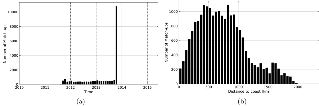
Figure 1: Number of match-ups between Argo and Aquarius-L4-IPRC-V4-WEEKLY SSS as a function of time (a) and as function of the distance to coast (b) over the Tropical Atlantic Ocean Pi-MEP region and for the full satellite product period.
