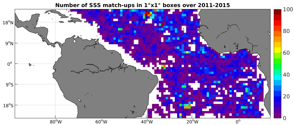
Figure 4: Number of SSS match-ups between Argo SSS and the Aquarius-L4-IPRC-V4-WEEKLY SSS product for the Tropical Atlantic Ocean Pi-MEP region over 1^\circ \times 1^\circ boxes and for the full satellite product period.
