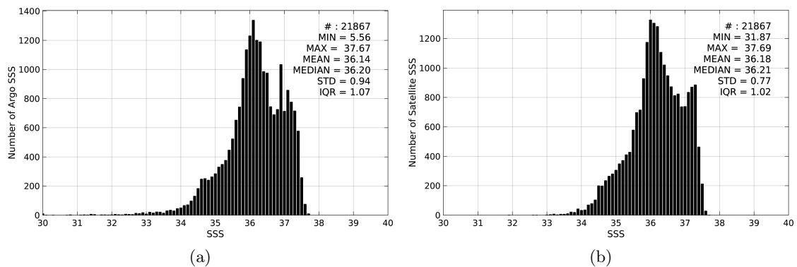
Figure 2: Histograms of SSS from Argo (a) and Aquarius-L4-IPRC-V4-WEEKLY (b) considering all match-up pairs per bins of 0.1 over the Tropical Atlantic Ocean Pi-MEP region and for the full satellite product period.
