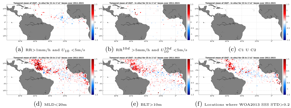
Figure 12: Temporal mean gridded over spatial boxes of size 1^\circ \times 1^\circ of \Delta SSS (Aquarius-L4-IPRC-V4-WEEKLY - Argo) for 6 different subdatasets corresponding to: RR > 1\text{mm/h} and U_{10} < 5\text{m/s} (a), RR^{10d} > 5\text{mm/h} and U_{10}^{10d} < 5\text{m/s} (b), C1 U C2 (c), MLD < 20\text{m} (d), BLT > 10\text{m} (e), Locations where WOA2013 SSS STD > 0.2 (f).
