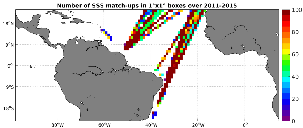
Figure 4: Number of SSS match-ups between TSG-LEGOS-DM SSS and the Aquarius-L4-IPRC-V4-MONTHLY SSS product for the Tropical Atlantic Ocean Pi-MEP region over 1^\circ \times 1^\circ boxes and for the full satellite product period.
