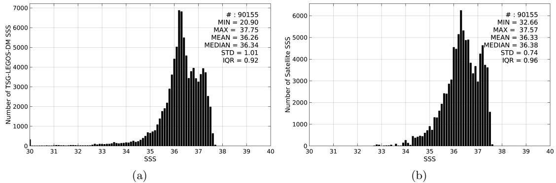
Figure 2: Histograms of SSS from TSG-LEGOS-DM (a) and Aquarius-L4-IPRC-V4-MONTHLY (b) considering all match-up pairs per bins of 0.1 over the Tropical Atlantic Ocean Pi-MEP region and for the full satellite product period.
