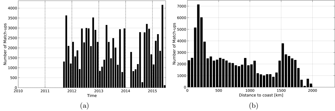
Figure 1: Number of match-ups between TSG-LEGOS-DM and Aquarius-L4-IPRC-V4-MONTHLY SSS as a function of time (a) and as function of the distance to coast (b) over the Tropical Atlantic Ocean Pi-MEP region and for the full satellite product period.
