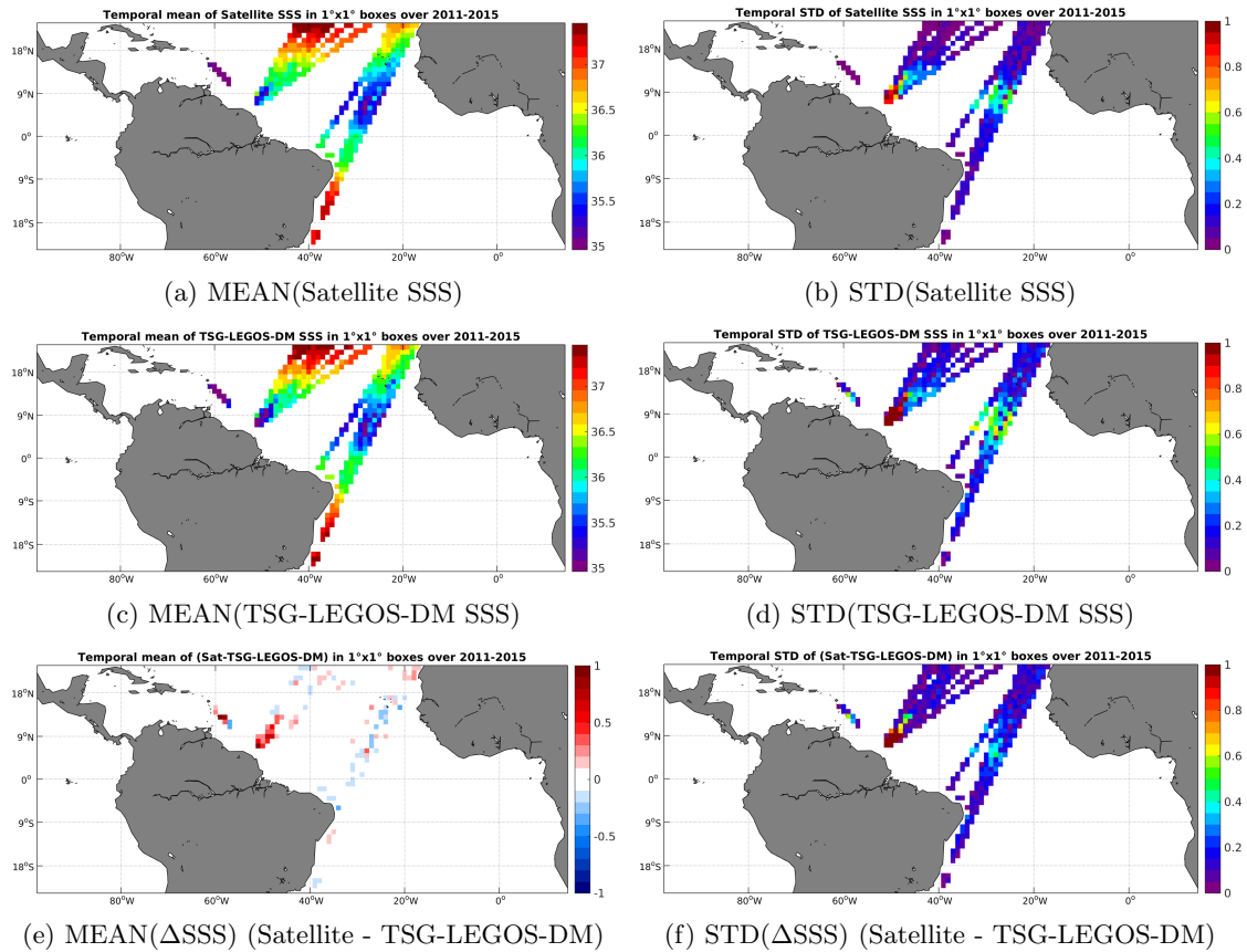
Figure 6: Temporal mean (left) and STD (right) of SSS from Aquarius-L4-IPRC-V4-MONTHLY (top), TSG-LEGOS-DM (middle), and of \Delta SSS (Satellite - TSG-LEGOS-DM). Only match-up pairs are used to generate these maps.
