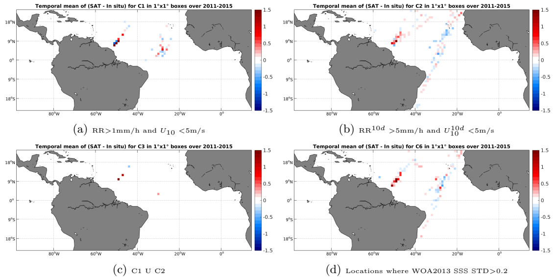
Figure 12: Temporal mean gridded over spatial boxes of size 1^\circ \times 1^\circ of \Delta SSS (Aquarius-L4-IPRC-V4-MONTHLY - TSG-LEGOS-DM) for 4 different subdatasets corresponding to:RR>1mm/h and U_{10} < 5\text{m/s} (a), RR^{10d} > 5\text{mm/h} and U_{10}^{10d} < 5\text{m/s} (b), C1 U C2 (c),Locations where WOA2013 SSS STD>0.2 (d).
