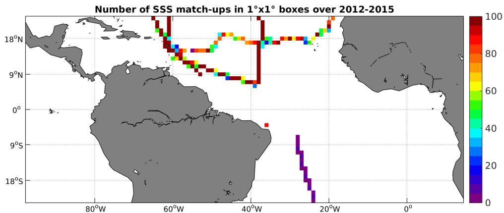
Figure 4: Number of SSS match-ups between TSG-GOSUD-Sailing-ship SSS and the Aquarius-L4-IPRC-V4-MONTHLY SSS product for the Tropical Atlantic Ocean Pi-MEP region over 1^\circ \times 1^\circ boxes and for the full satellite product period.
