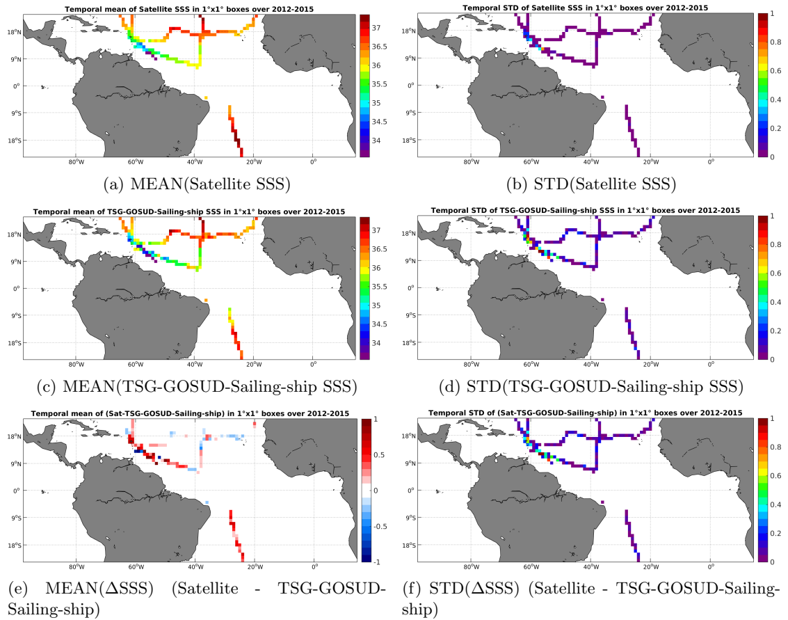
Figure 6: Temporal mean (left) and STD (right) of SSS from Aquarius-L4-IPRC-V4-MONTHLY (top), TSG-GOSUD-Sailing-ship (middle), and of \Delta SSS (Satellite - TSG-GOSUD-Sailing-ship). Only match-up pairs are used to generate these maps.
