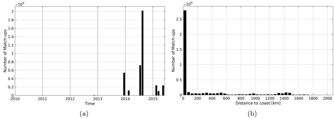
Figure 1: Number of match-ups between TSG-GOSUD-Sailing-ship and Aquarius-L4-IPRC-V4-MONTHLY SSS as a function of time (a) and as function of the distance to coast (b) over the Tropical Atlantic Ocean Pi-MEP region and for the full satellite product period.
