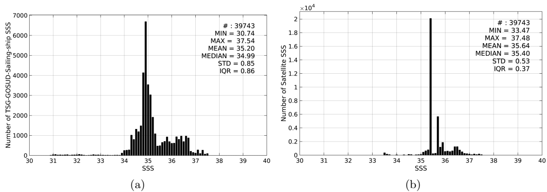
Figure 2: Histograms of SSS from TSG-GOSUD-Sailing-ship (a) and Aquarius-L4-IPRC-V4-MONTHLY (b) considering all match-up pairs per bins of 0.1 over the Tropical Atlantic Ocean Pi-MEP region and for the full satellite product period.
