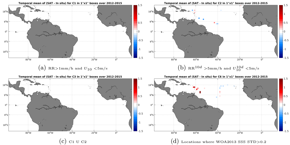
Figure 12: Temporal mean gridded over spatial boxes of size 1^\circ \times 1^\circ of \Delta SSS (Aquarius-L4-IPRC-V4-MONTHLY - TSG-GOSUD-Sailing-ship) for 4 different subdatasets corresponding to: RR > 1\text{mm/h} and U_{10} < 5\text{m/s} (a), RR^{10d} > 5\text{mm/h} and U_{10}^{10d} < 5\text{m/s} (b), C1 U C2 (c), Locations where WOA2013 SSS STD > 0.2 (d).
