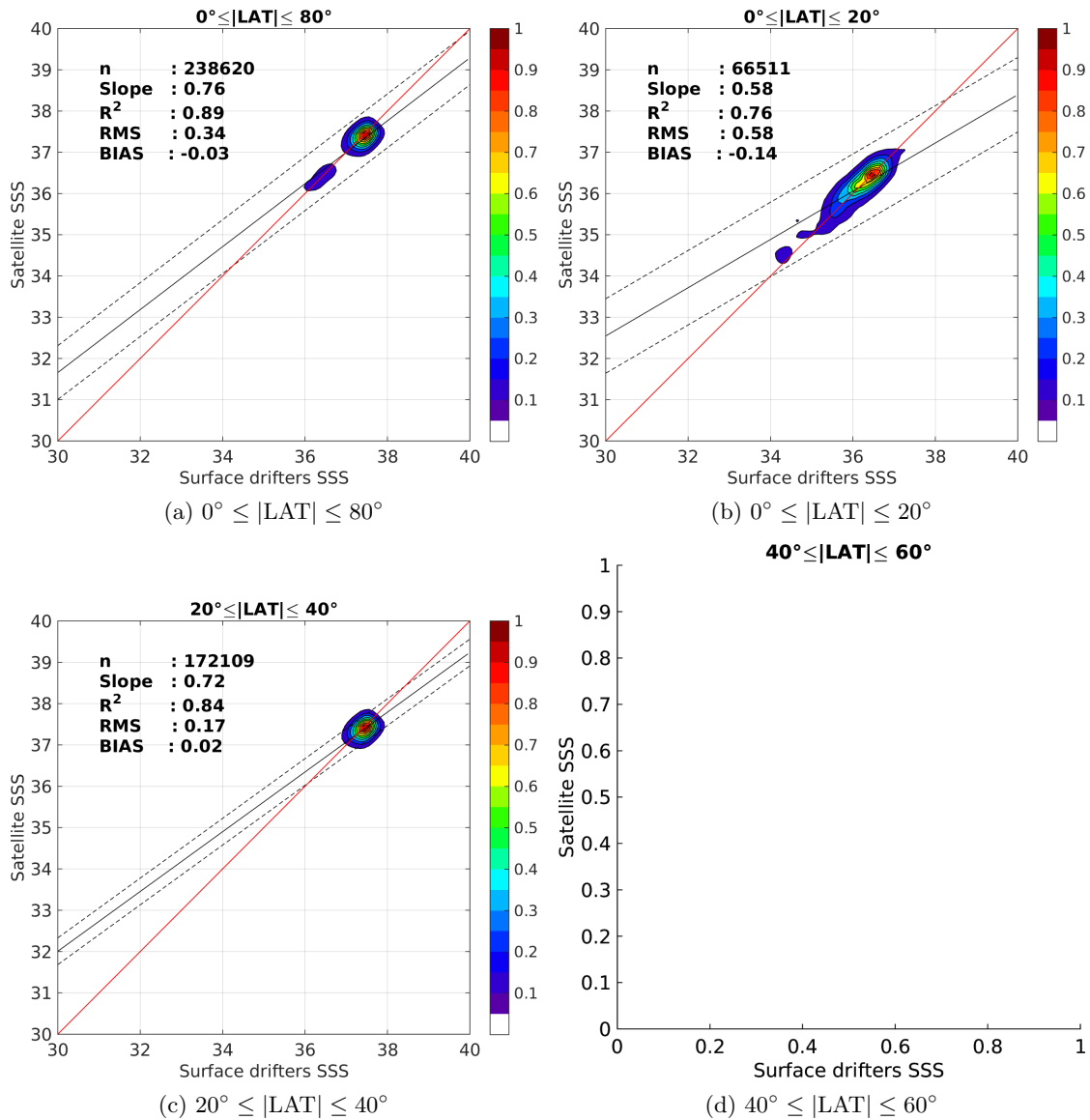
Figure 8: Contour maps of the concentration of Aquarius-L4-IPRC-V4-MONTHLY SSS (y-axis) versus Surface drifters SSS (x-axis) at match-up pairs for different latitude bands. For each plot, the red line shows x=y . The black thin and dashed lines indicate a linear fit through the data cloud and the \pm 95\% confidence levels, respectively. The number match-up pairs n , the slope and R^2 coefficient of the linear fit, the root mean square (RMS) and the mean bias between satellite and in situ data are indicated for each latitude band in each plots.
