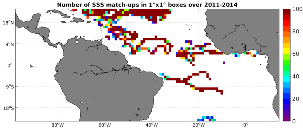
Figure 3: Number of SSS match-ups between Surface drifters SSS and the Aquarius-L4-IPRC-V4-MONTHLY SSS product for the Tropical Atlantic Ocean Pi-MEP region over 1^\circ \times 1^\circ boxes and for the full satellite product period.
