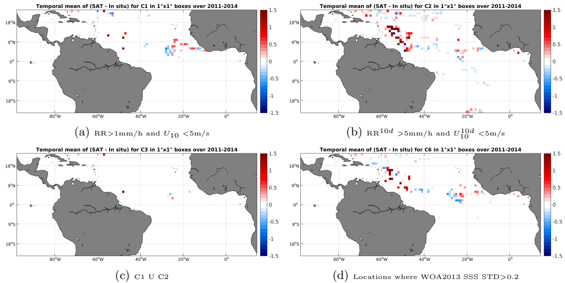
Figure 11: Temporal mean gridded over spatial boxes of size 1^\circ \times 1^\circ of \Delta SSS (Aquarius-L4-IPRC-V4-MONTHLY - Surface drifters) for 4 different subdatasets corresponding to: RR > 1\text{mm/h} and U_{10} < 5\text{m/s} (a), RR^{10d} > 5\text{mm/h} and U_{10}^{10d} < 5\text{m/s} (b), C1 U C2 (c), Locations where WOA2013 SSS STD > 0.2 (d).
