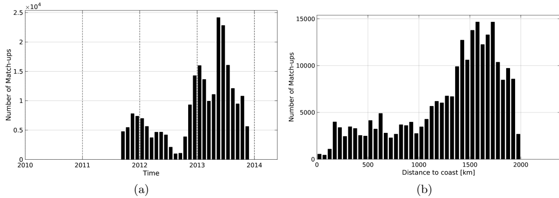
Figure 1: Number of match-ups between Surface drifters and Aquarius-L4-IPRC-V4-MONTHLY SSS as a function of time (a) and as function of the distance to coast (b) over the Tropical Atlantic Ocean Pi-MEP region and for the full satellite product period.
