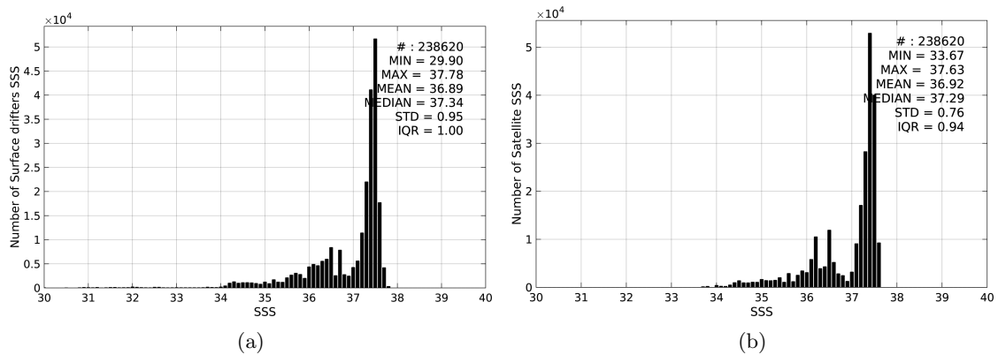
Figure 2: Histograms of SSS from Surface drifters (a) and Aquarius-L4-IPRC-V4-MONTHLY (b) considering all match-up pairs per bins of 0.1 over the Tropical Atlantic Ocean Pi-MEP region and for the full satellite product period.
