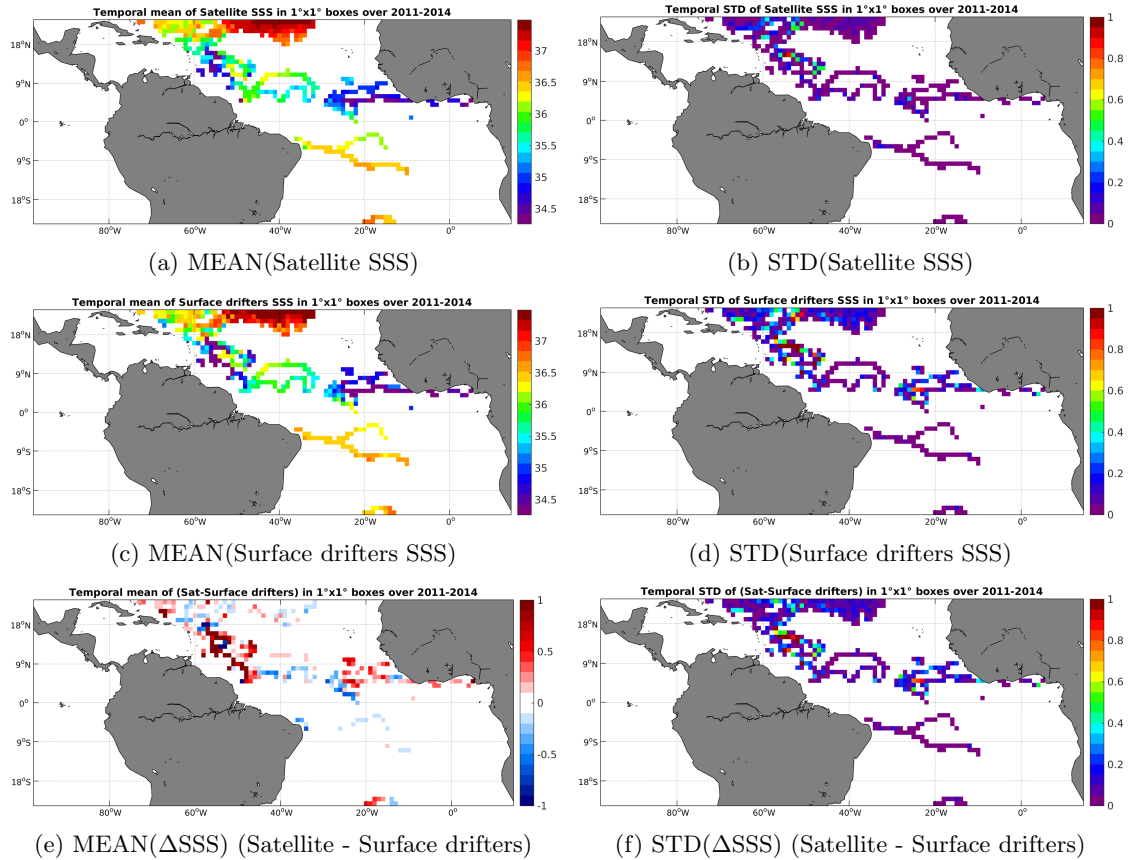
Figure 5: Temporal mean (left) and STD (right) of SSS from Aquarius-L4-IPRC-V4-MONTHLY (top), Surface drifters (middle), and of \Delta SSS (Satellite - Surface drifters). Only match-up pairs are used to generate these maps.
