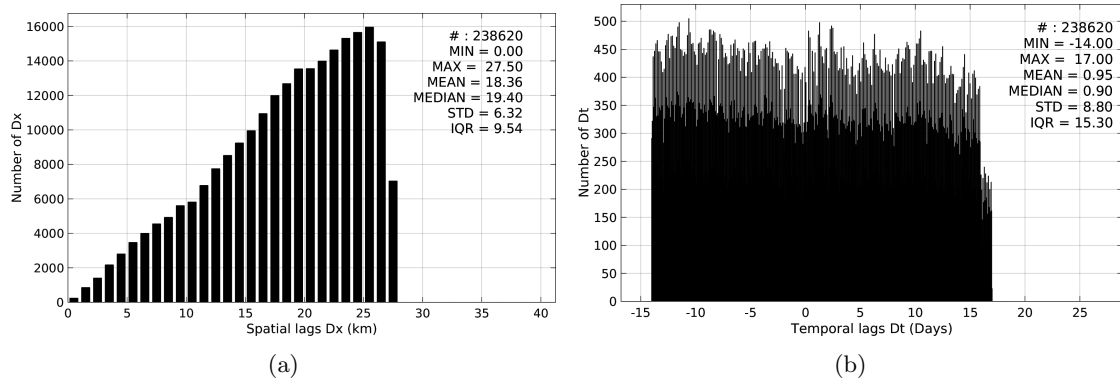
Figure 4: Histograms of the spatial (a) and temporal (b) lags between the time of the Surface drifters measurements and the date of the corresponding Aquarius-L4-IPRC-V4-MONTHLY SSS product.
