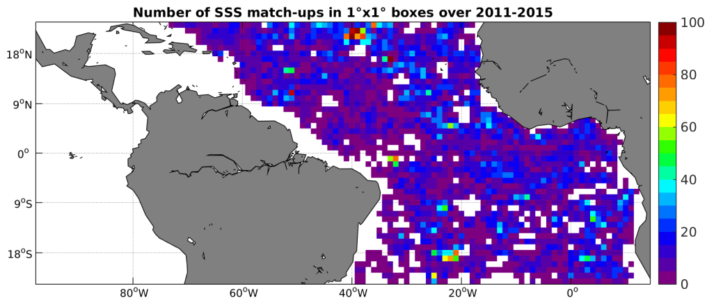
Figure 4: Number of SSS match-ups between Argo SSS and the Aquarius-L4-IPRC-V4-MONTHLY SSS product for the Tropical Atlantic Ocean Pi-MEP region over 1^{\circ} \times 1^{\circ} boxes and for the full satellite product period.
