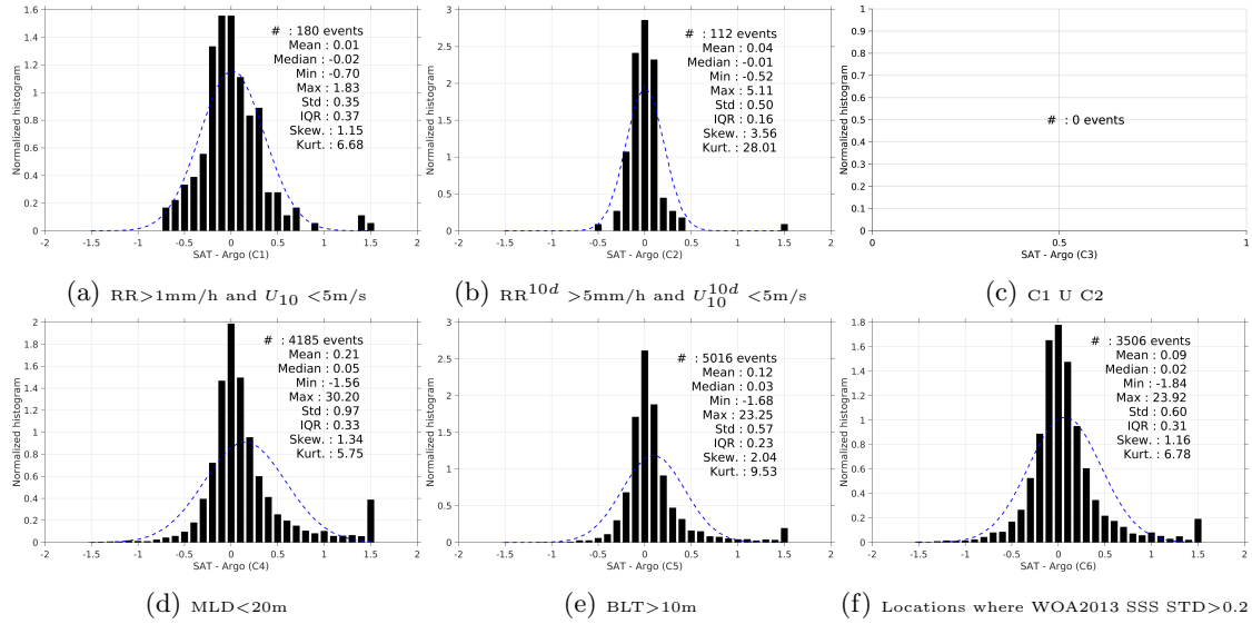
Figure 13: Normalized histogram of \Delta SSS (Aquarius-L4-IPRC-V4-MONTHLY - Argo) for 6 different subdatasets corresponding to: RR > 1mm/h and U_{10} < 5 m/s (a), RR^{10d} > 5 mm/h and U_{10}^{10d} < 5 m/s (b), C1 U C2 (c), MLD < 20m (d), BLT > 10m (e), Locations where WOA2013 SSS STD > 0.2 (f).
