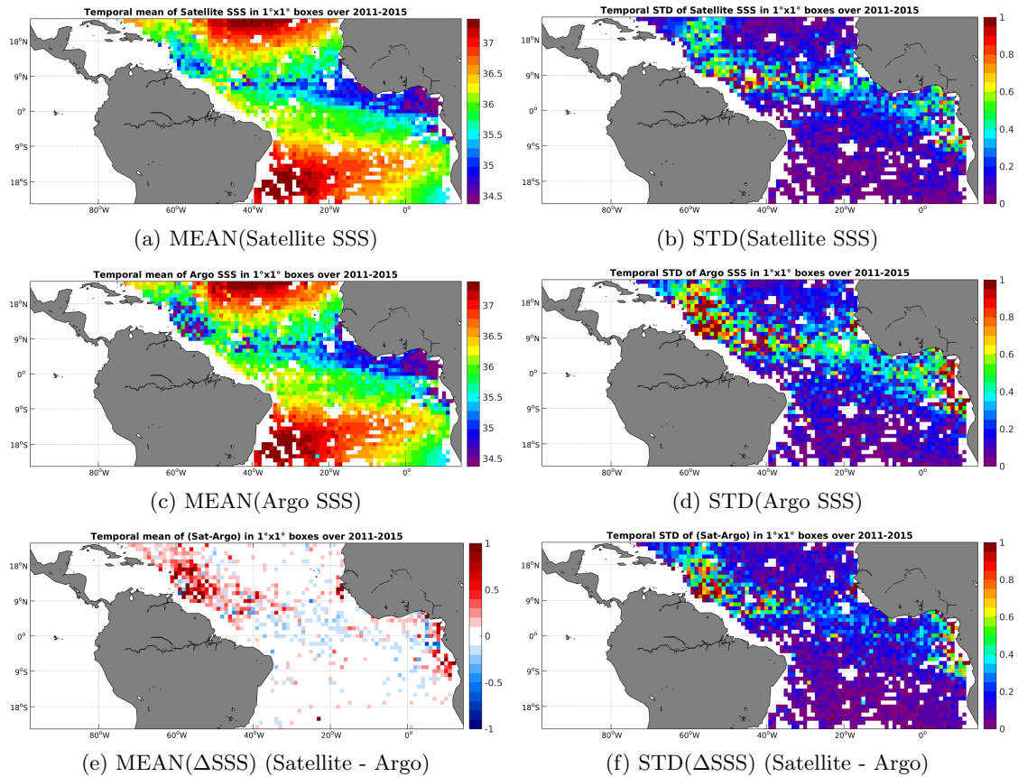
Figure 6: Temporal mean (left) and STD (right) of SSS from Aquarius-L4-IPRC-V4-MONTHLY (top), Argo (middle), and of \Delta SSS (Satellite - Argo). Only match-up pairs are used to generate these maps.
