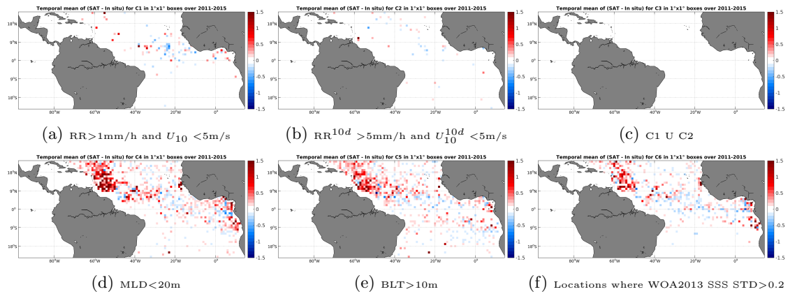
Figure 12: Temporal mean gridded over spatial boxes of size 1^\circ \times 1^\circ of \Delta SSS (Aquarius-L4-IPRC-V4-MONTHLY - Argo) for 6 different subdatasets corresponding to: RR > 1\text{mm/h} and U_{10} < 5\text{m/s} (a), RR^{10d} > 5\text{mm/h} and U_{10}^{10d} < 5\text{m/s} (b), C1 U C2 (c), MLD < 20\text{m} (d), BLT > 10\text{m} (e), Locations where WOA2013 SSS STD > 0.2 (f).
