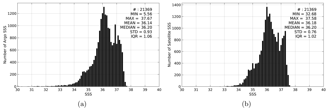
Figure 2: Histograms of SSS from Argo (a) and Aquarius-L4-IPRC-V4-MONTHLY (b) considering all match-up pairs per bins of 0.1 over the Tropical Atlantic Ocean Pi-MEP region and for the full satellite product period.
