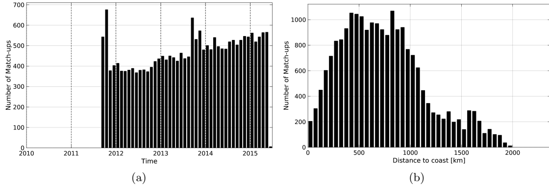
Figure 1: Number of match-ups between Argo and Aquarius-L4-IPRC-V4-MONTHLY SSS as a function of time (a) and as function of the distance to coast (b) over the Tropical Atlantic Ocean Pi-MEP region and for the full satellite product period.
