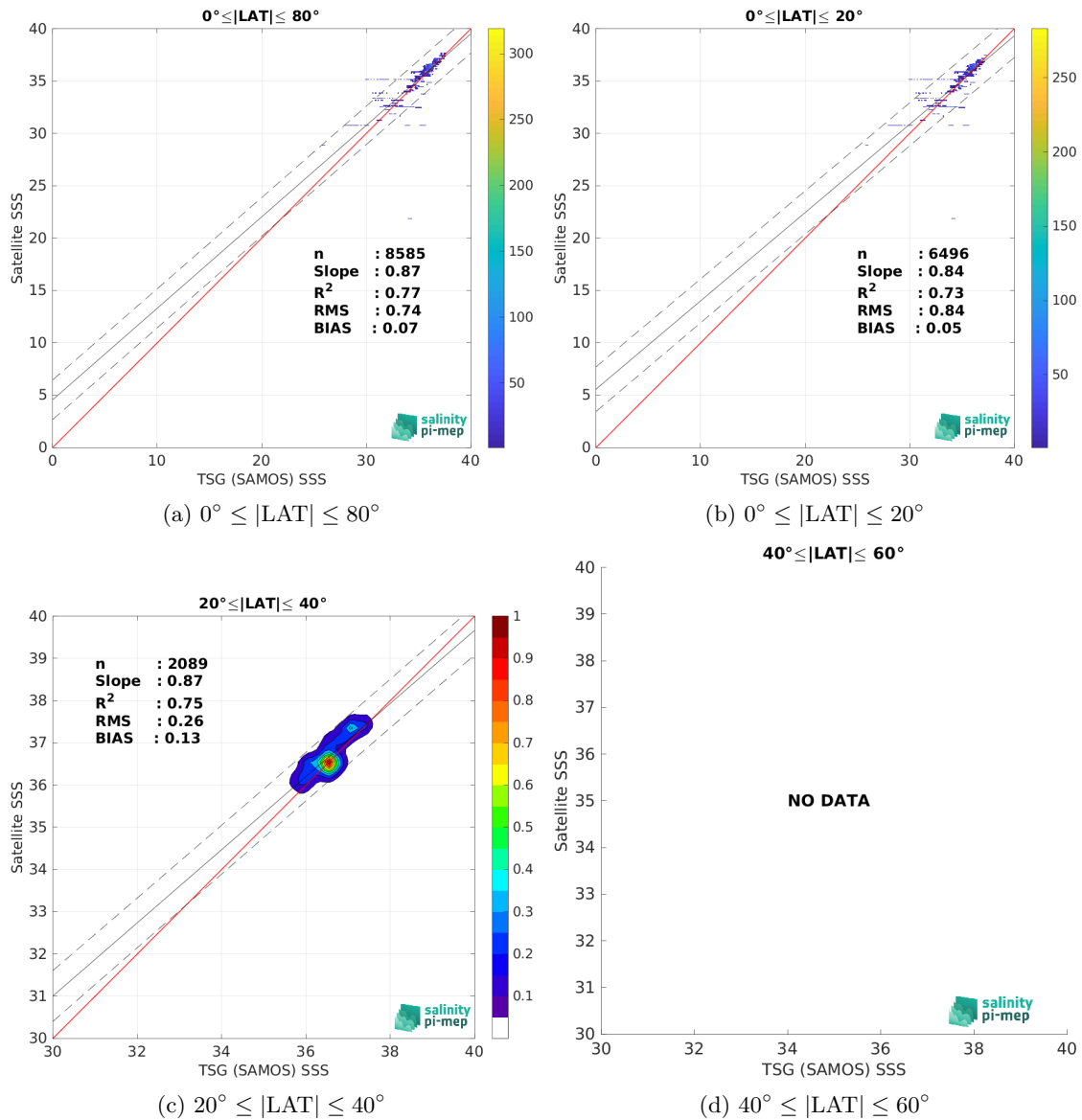
Figure 10: Contour maps of the concentration of Aquarius SSS L3 OR v5 - 7-Day running (NASA-GSFC) SSS (y-axis) versus TSG (SAMOS) SSS (x-axis) at match-up pairs for different latitude bands. For each plot, the red line shows x=y . The black thin and dashed lines indicate a linear fit through the data cloud and the \pm 95\% confidence levels, respectively. The number match-up pairs n , the slope and R^2 coefficient of the linear fit, the root mean square (RMS) and the mean bias between satellite and in situ data are indicated for each latitude band in each plots.
