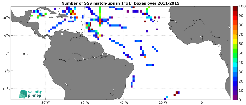
Figure 5: Number of SSS match-ups between TSG (SAMOS) SSS and the Aquarius SSS L3 OR v5 - 7-Day running (NASA-GSFC) SSS product for the Tropical Atlantic Ocean Pi-MEP region over 1^\circ \times 1^\circ boxes and for the full satellite product period.
