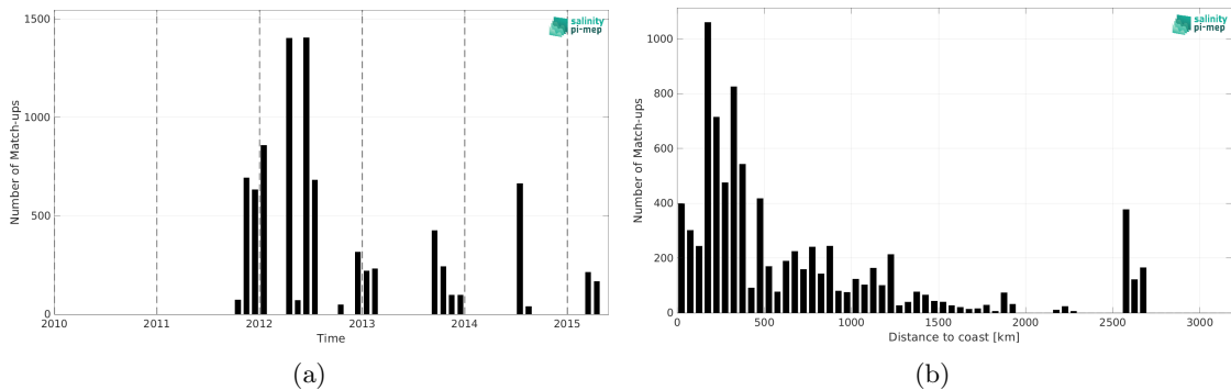
Figure 2: Number of match-ups between TSG (SAMOS) and Aquarius SSS L3 OR v5 - 7-Day running (NASA-GSFC) SSS as a function of time (a) and as function of the distance to coast (b) over the Tropical Atlantic Ocean Pi-MEP region and for the full satellite product period.
