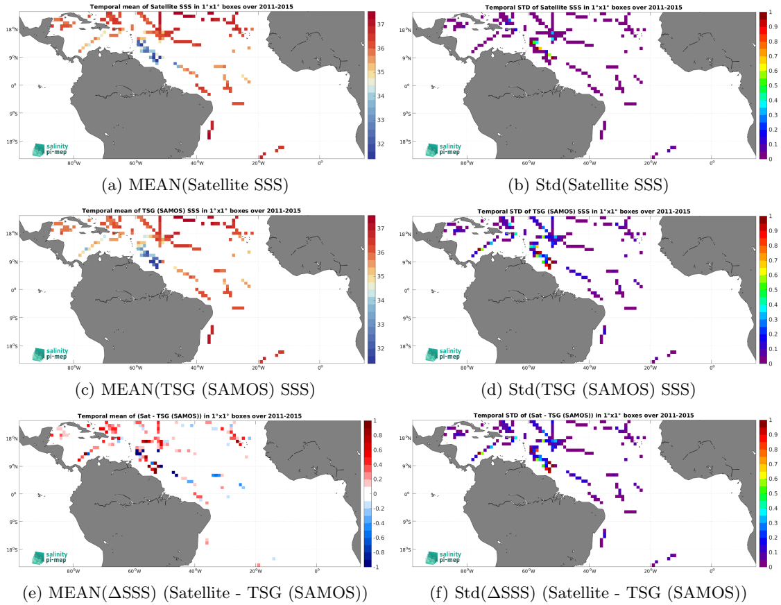
Figure 7: Temporal mean (left) and Std (right) of SSS from Aquarius SSS L3 OR v5 - 7-Day running (NASA-GSFC) (top), TSG (SAMOS) (middle), and of \Delta\text{SSS} (Satellite - TSG (SAMOS)). Only match-up pairs are used to generate these maps.
