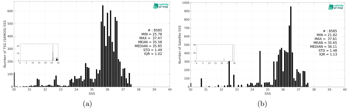
Figure 3: Histograms of SSS from TSG (SAMOS) (a) and Aquarius SSS L3 OR v5 - 7-Day running (NASA-GSFC) (b) considering all match-up pairs per bins of 0.1 over the Tropical Atlantic Ocean Pi-MEP region and for the full satellite product period.
