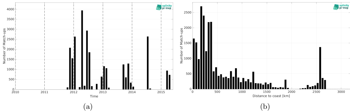
Figure 1: Number of match-ups between TSG (SAMOS) and Aquarius SSS L3 OR v5 - 7-Day running (NASA-GSFC) SSS as a function of time (a) and as function of the distance to coast (b) over the Tropical Atlantic Ocean Pi-MEP region and for the full satellite product period.
