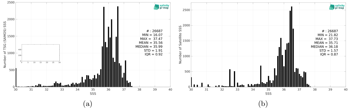
Figure 2: Histograms of SSS from TSG (SAMOS) (a) and Aquarius SSS L3 OR v5 - 7-Day running (NASA-GSFC) (b) considering all match-up pairs per bins of 0.1 over the Tropical Atlantic Ocean Pi-MEP region and for the full satellite product period.
