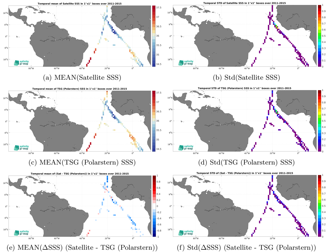
Figure 7: Temporal mean (left) and Std (right) of SSS from Aquarius SSS L3 OR v5 - 7-Day running (NASA-GSFC) (top), TSG (Polarstern) (middle), and of \Delta SSS (Satellite - TSG (Polarstern)). Only match-up pairs are used to generate these maps.
