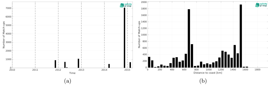
Figure 2: Number of match-ups between TSG (Polarstern) and Aquarius SSS L3 OR v5 - 7-Day running (NASA-GSFC) SSS as a function of time (a) and as function of the distance to coast (b) over the Tropical Atlantic Ocean Pi-MEP region and for the full satellite product period.
