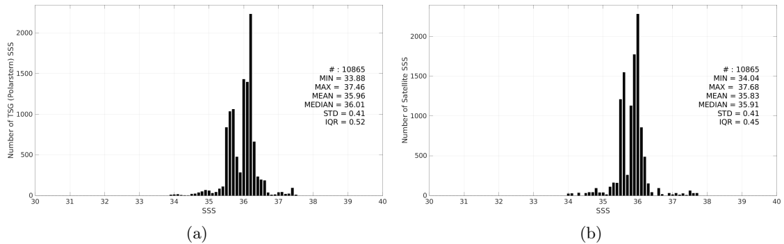
Figure 3: Histograms of SSS from TSG (Polarstern) (a) and Aquarius SSS L3 OR v5 - 7-Day running (NASA-GSFC) (b) considering all match-up pairs per bins of 0.1 over the Tropical Atlantic Ocean Pi-MEP region and for the full satellite product period.
