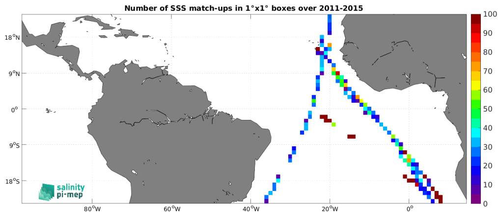
Figure 5: Number of SSS match-ups between TSG (Polarstern) SSS and the Aquarius SSS L3 OR v5 - 7-Day running (NASA-GSFC) SSS product for the Tropical Atlantic Ocean Pi-MEP region over 1^\circ \times 1^\circ boxes and for the full satellite product period.
