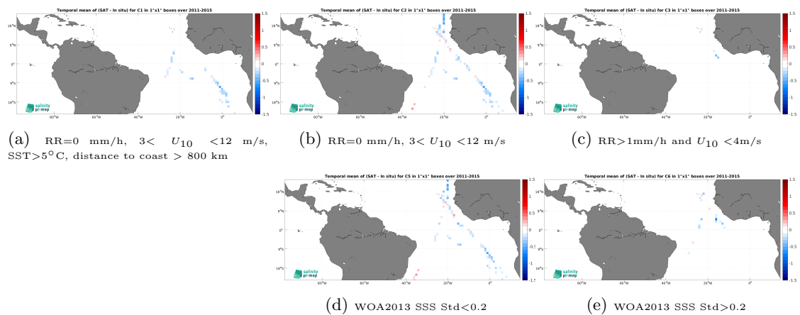
Figure 14: Temporal mean gridded over spatial boxes of size 1^\circ \times 1^\circ of \Delta SSS (Aquarius SSS L3 OR v5 - 7-Day running (NASA-GSFC) - TSG (Polarstern)) for 5 different subdatasets corresponding to:RR=0 mm/h, 3 < U_{10} < 12 m/s, SST >5^\circ\text{C} , distance to coast > 800 km (a), RR=0 mm/h, 3 < U_{10} < 12 m/s (b), RR >1 mm/h and U_{10} < 4 m/s (c), WOA2013 SSS Std <0.2 (d), WOA2013 SSS Std >0.2 (e).
