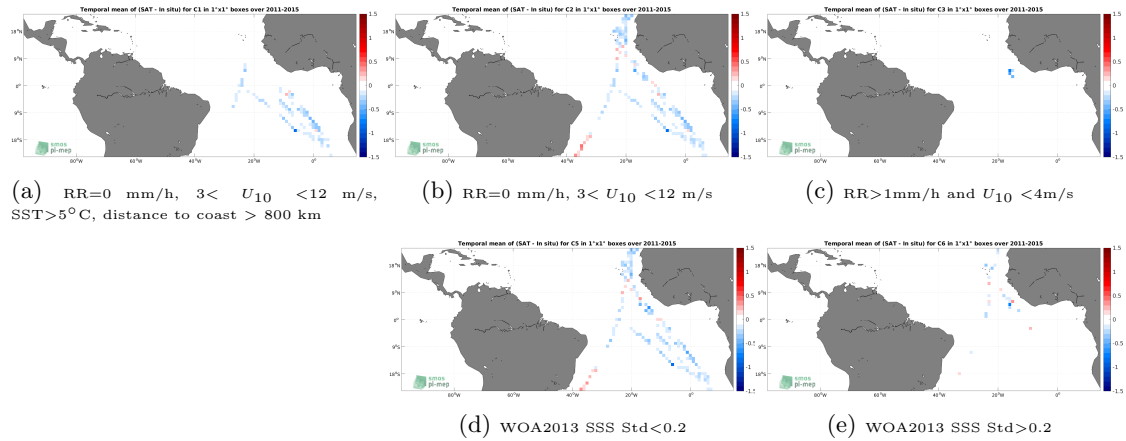
Figure 12: Temporal mean gridded over spatial boxes of size 1^\circ \times 1^\circ of \Delta SSS (Aquarius SSS L3 OR v5 - 7-Day running (NASA-GSFC) - TSG (Polarstern)) for 5 different subdatasets corresponding to:RR=0 mm/h, 3 < U_{10} < 12 m/s, SST >5^\circ\text{C} , distance to coast > 800 km (a), RR=0 mm/h, 3 < U_{10} < 12 m/s (b), RR >1 mm/h and U_{10} < 4 m/s (c), WOA2013 SSS Std <0.2 (d), WOA2013 SSS Std >0.2 (e).
