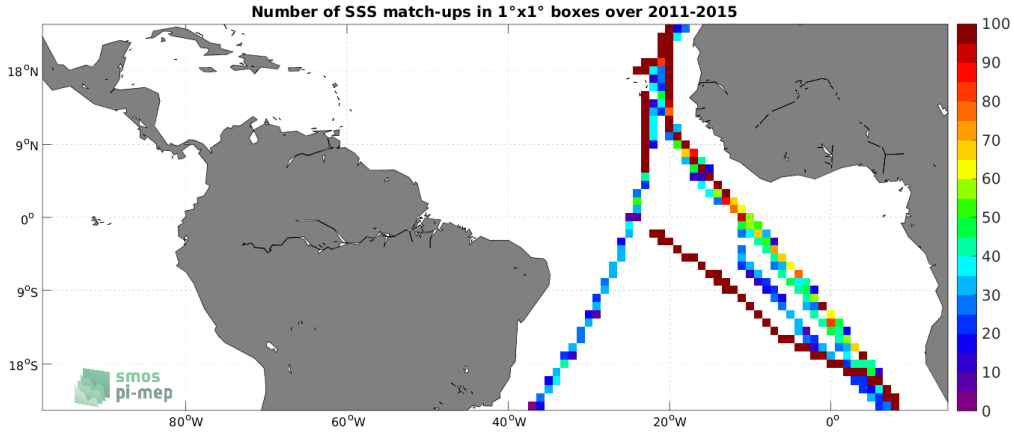
Figure 4: Number of SSS match-ups between TSG (Polarstern) SSS and the Aquarius SSS L3 OR v5 - 7-Day running (NASA-GSFC) SSS product for the Tropical Atlantic Ocean Pi-MEP region over 1^\circ \times 1^\circ boxes and for the full satellite product period.
