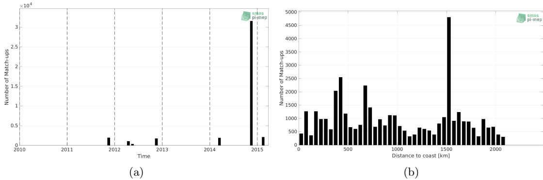
Figure 1: Number of match-ups between TSG (Polarstern) and Aquarius SSS L3 OR v5 - 7-Day running (NASA-GSFC) SSS as a function of time (a) and as function of the distance to coast (b) over the Tropical Atlantic Ocean Pi-MEP region and for the full satellite product period.
