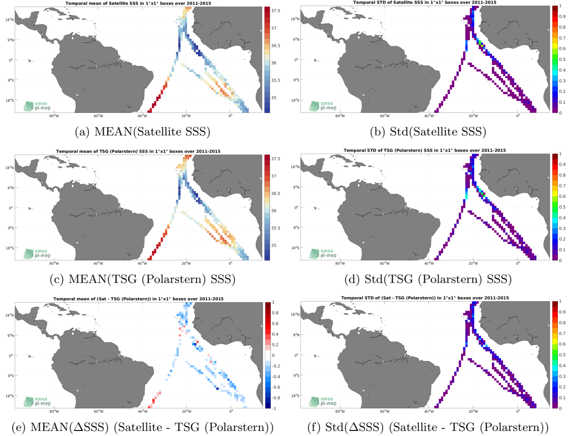
Figure 6: Temporal mean (left) and Std (right) of SSS from Aquarius SSS L3 OR v5 - 7-Day running (NASA-GSFC) (top), TSG (Polarstern) (middle), and of \Delta\text{SSS} (Satellite - TSG (Polarstern)). Only match-up pairs are used to generate these maps.
