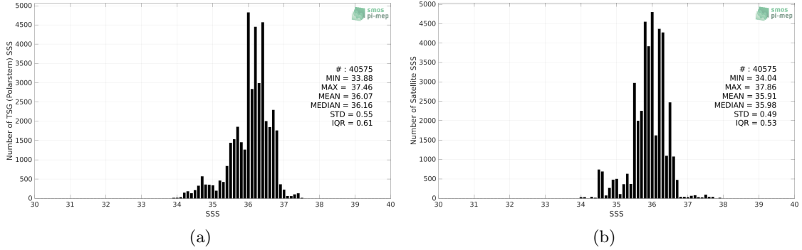
Figure 2: Histograms of SSS from TSG (Polarstern) (a) and Aquarius SSS L3 OR v5 - 7-Day running (NASA-GSFC) (b) considering all match-up pairs per bins of 0.1 over the Tropical Atlantic Ocean Pi-MEP region and for the full satellite product period.
