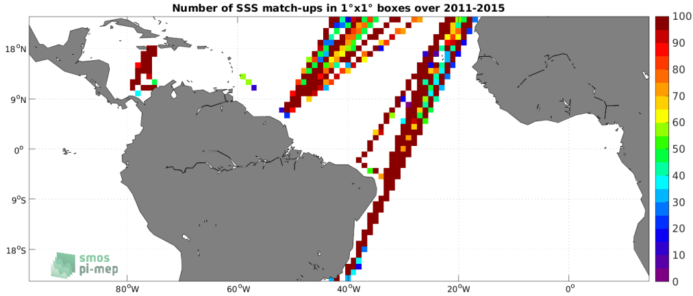
Figure 4: Number of SSS match-ups between TSG (LEGOS-DM) SSS and the Aquarius SSS L3 OR v5 - 7-Day running (NASA-GSFC) SSS product for the Tropical Atlantic Ocean Pi-MEP region over 1^\circ \times 1^\circ boxes and for the full satellite product period.
