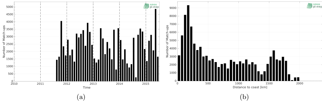
Figure 1: Number of match-ups between TSG (LEGOS-DM) and Aquarius SSS L3 OR v5 - 7-Day running (NASA-GSFC) SSS as a function of time (a) and as function of the distance to coast (b) over the Tropical Atlantic Ocean Pi-MEP region and for the full satellite product period.
