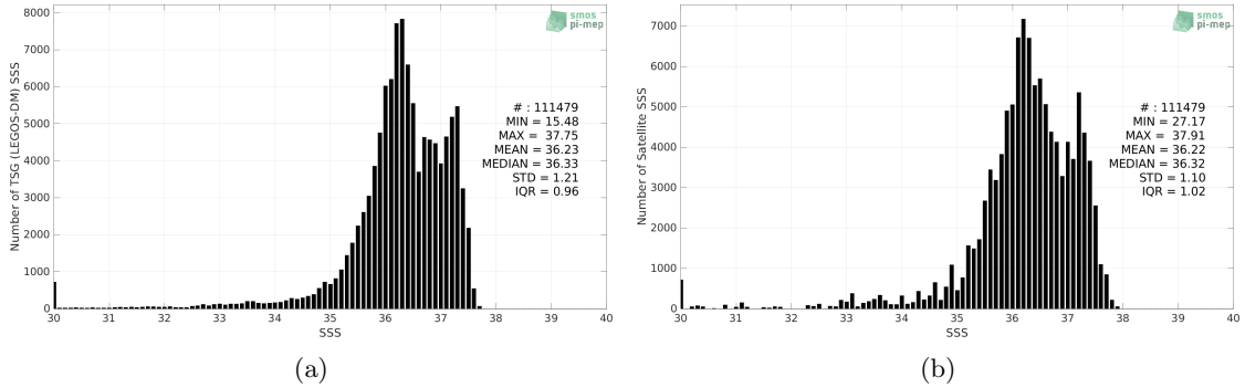
Figure 2: Histograms of SSS from TSG (LEGOS-DM) (a) and Aquarius SSS L3 OR v5 - 7-Day running (NASA-GSFC) (b) considering all match-up pairs per bins of 0.1 over the Tropical Atlantic Ocean Pi-MEP region and for the full satellite product period.
