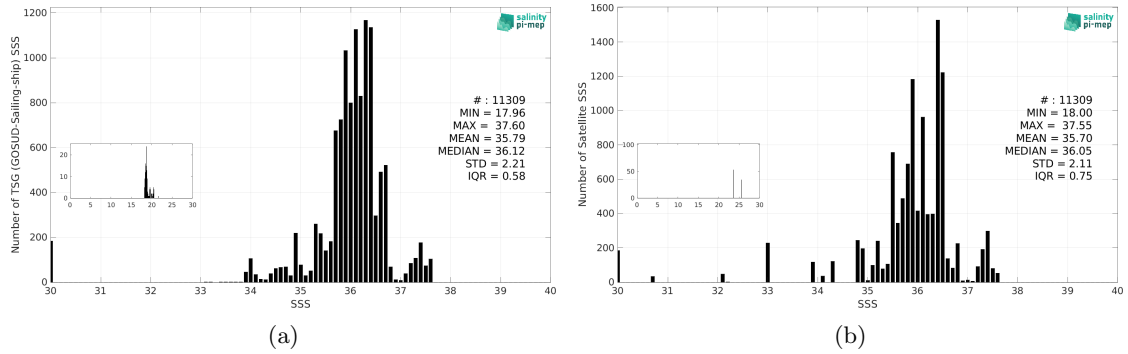
Figure 3: Histograms of SSS from TSG (GOSUD-Sailing-ship) (a) and Aquarius SSS L3 OR v5 - 7-Day running (NASA-GSFC) (b) considering all match-up pairs per bins of 0.1 over the Tropical Atlantic Ocean Pi-MEP region and for the full satellite product period.
