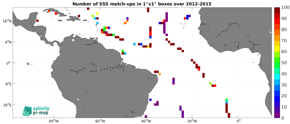
Figure 5: Number of SSS match-ups between TSG (GOSUD-Sailing-ship) SSS and the Aquarius SSS L3 OR v5 - 7-Day running (NASA-GSFC) SSS product for the Tropical Atlantic Ocean Pi-MEP region over 1^\circ \times 1^\circ boxes and for the full satellite product period.
