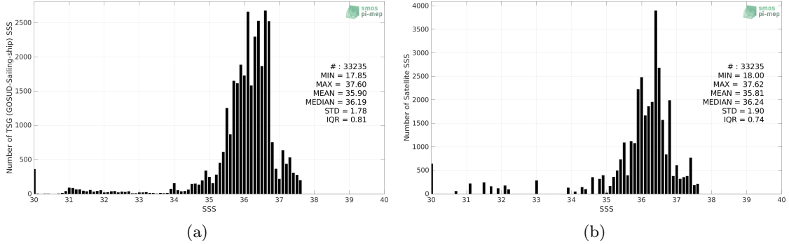
Figure 2: Histograms of SSS from TSG (GOSUD-Sailing-ship) (a) and Aquarius SSS L3 OR v5 - 7-Day running (NASA-GSFC) (b) considering all match-up pairs per bins of 0.1 over the Tropical Atlantic Ocean Pi-MEP region and for the full satellite product period.
