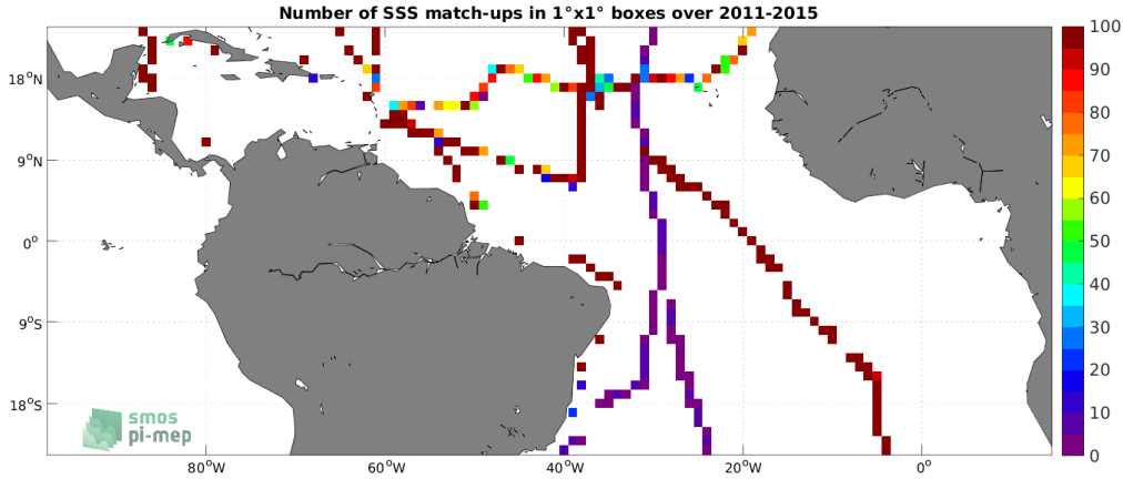
Figure 4: Number of SSS match-ups between TSG (GOSUD-Sailing-ship) SSS and the Aquarius SSS L3 OR v5 - 7-Day running (NASA-GSFC) SSS product for the Tropical Atlantic Ocean Pi-MEP region over 1^\circ \times 1^\circ boxes and for the full satellite product period.
