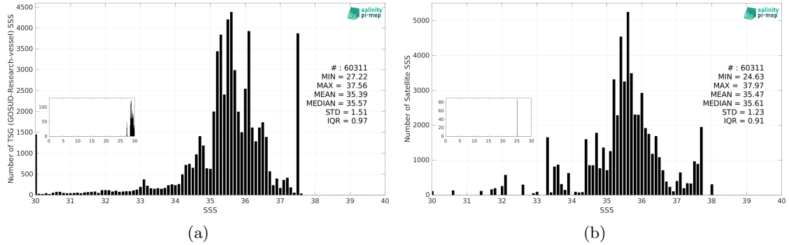
Figure 3: Histograms of SSS from TSG (GOSUD-Research-vessel) (a) and Aquarius SSS L3 OR v5 - 7-Day running (NASA-GSFC) (b) considering all match-up pairs per bins of 0.1 over the Tropical Atlantic Ocean Pi-MEP region and for the full satellite product period.
