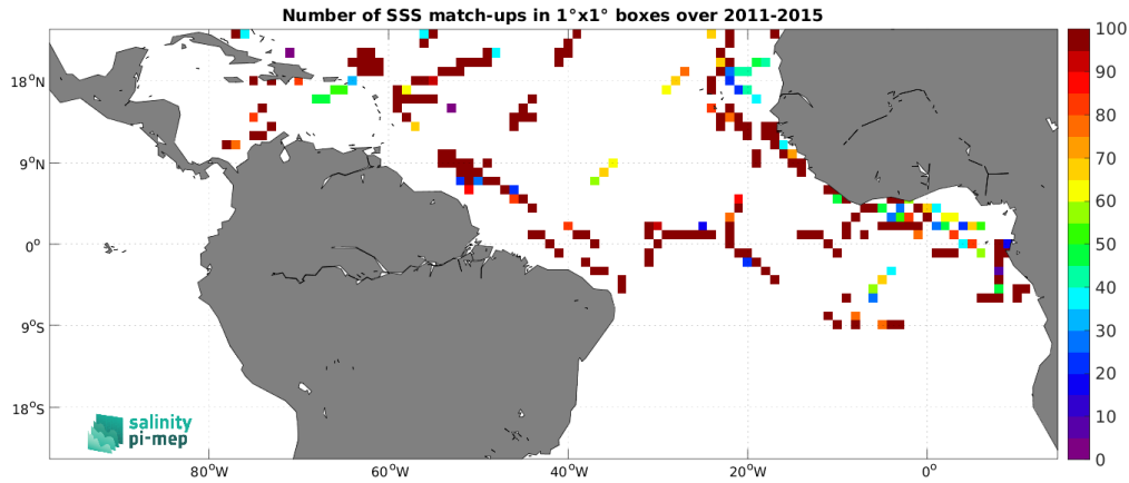
Figure 5: Number of SSS match-ups between TSG (GOSUD-Research-vessel) SSS and the Aquarius SSS L3 OR v5 - 7-Day running (NASA-GSFC) SSS product for the Tropical Atlantic Ocean Pi-MEP region over 1^\circ \times 1^\circ boxes and for the full satellite product period.
