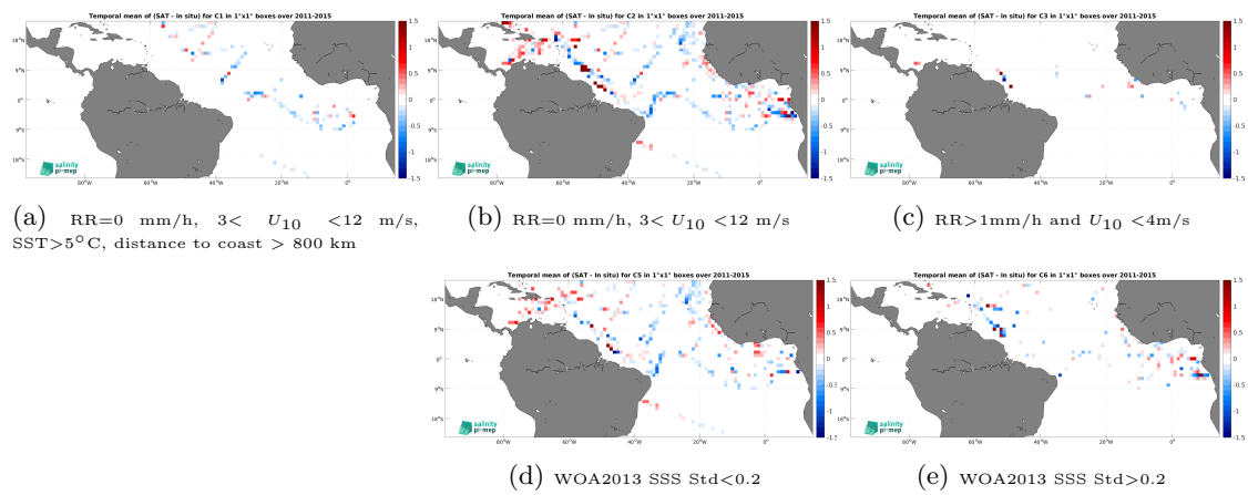
Figure 12: Temporal mean gridded over spatial boxes of size 1^\circ \times 1^\circ of \Delta SSS (Aquarius SSS L3 OR v5 - 7-Day running (NASA-GSFC) - TSG (GOSUD-Research-vessel)) for 5 different subdatasets corresponding to:RR=0 mm/h, 3 < U_{10} < 12 m/s, SST >5^\circ\text{C} , distance to coast > 800 km (a), RR=0 mm/h, 3 < U_{10} < 12 m/s (b), RR >1 mm/h and U_{10} < 4 m/s (c), WOA2013 SSS Std <0.2 (d), WOA2013 SSS Std >0.2 (e).
