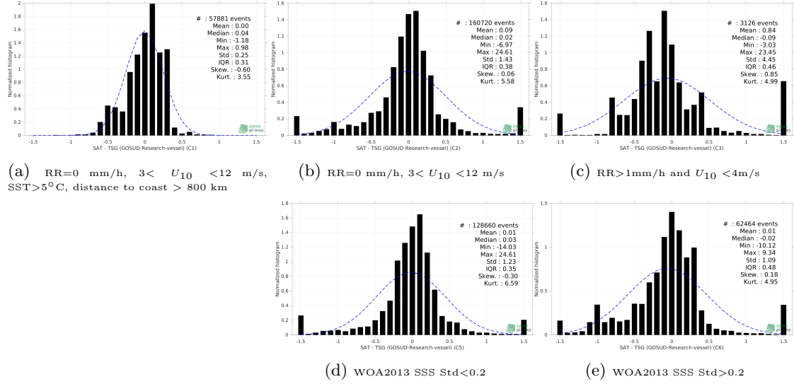
Figure 13: Normalized histogram of \Delta\text{SSS} (Aquarius SSS L3 OR v5 - 7-Day running (NASA-GSFC) - TSG (GOSUD-Research-vessel)) for 5 different subdatasets corresponding to: RR=0 mm/h, 3 < U_{10} < 12 m/s, SST > 5^\circ\text{C} , distance to coast > 800 km (a), RR=0 mm/h, 3 < U_{10} < 12 m/s (b), RR > 1 mm/h and U_{10} < 4 m/s (c), WOA2013 SSS Std < 0.2 (d), WOA2013 SSS Std > 0.2 (e).
