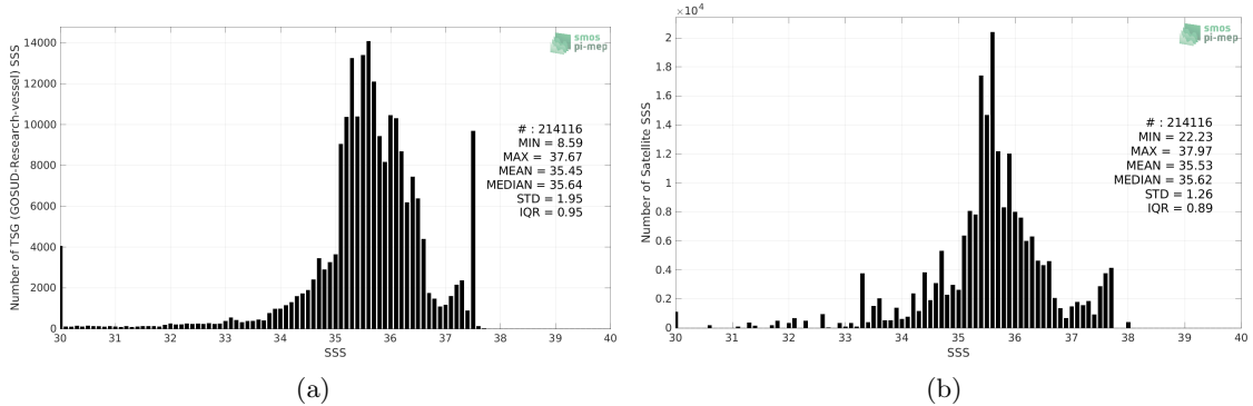
Figure 2: Histograms of SSS from TSG (GOSUD-Research-vessel) (a) and Aquarius SSS L3 OR v5 - 7-Day running (NASA-GSFC) (b) considering all match-up pairs per bins of 0.1 over the Tropical Atlantic Ocean Pi-MEP region and for the full satellite product period.
