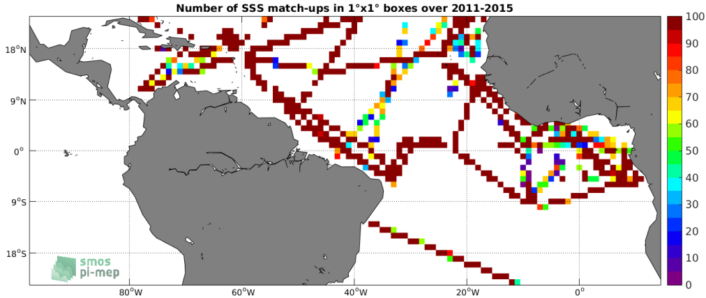
Figure 4: Number of SSS match-ups between TSG-GOSUD-Research-vessel SSS and the Aquarius-L3-OR-V5-7DAY-RUNNING-1DEG SSS product for the Tropical Atlantic Ocean Pi-MEP region over 1^\circ \times 1^\circ boxes and for the full satellite product period.
