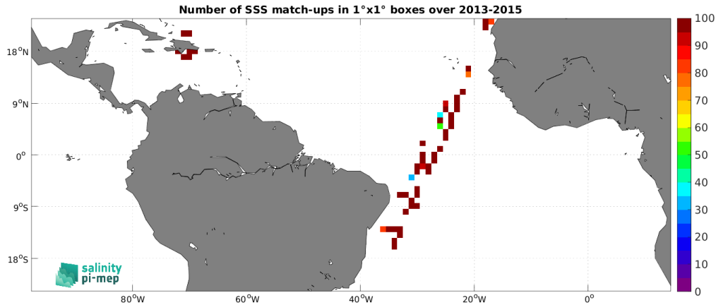
Figure 5: Number of SSS match-ups between TSG (CSIC-UTM) SSS and the Aquarius SSS L3 OR v5 - 7-Day running (NASA-GSFC) SSS product for the Tropical Atlantic Ocean Pi-MEP region over 1^\circ \times 1^\circ boxes and for the full satellite product period.
