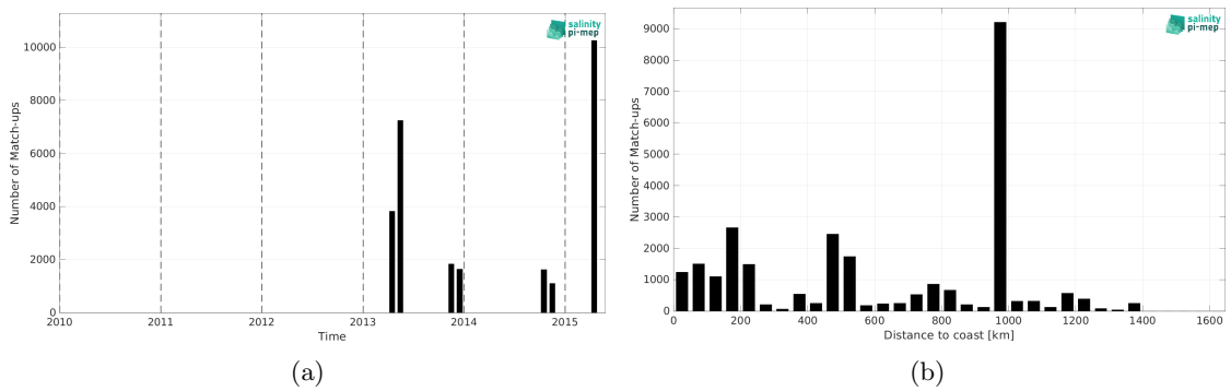
Figure 2: Number of match-ups between TSG (CSIC-UTM) and Aquarius SSS L3 OR v5 - 7-Day running (NASA-GSFC) SSS as a function of time (a) and as function of the distance to coast (b) over the Tropical Atlantic Ocean Pi-MEP region and for the full satellite product period.
