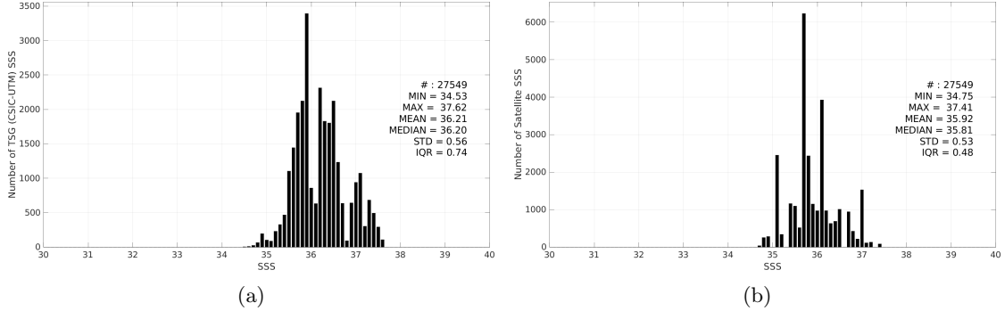
Figure 3: Histograms of SSS from TSG (CSIC-UTM) (a) and Aquarius SSS L3 OR v5 - 7-Day running (NASA-GSFC) (b) considering all match-up pairs per bins of 0.1 over the Tropical Atlantic Ocean Pi-MEP region and for the full satellite product period.
