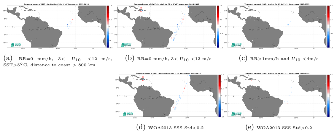
Figure 14: Temporal mean gridded over spatial boxes of size 1^\circ \times 1^\circ of \Delta\text{SSS} (Aquarius SSS L3 OR v5 - 7-Day running (NASA-GSFC) - TSG (CSIC-UTM)) for 5 different subdatasets corresponding to:RR=0 mm/h, 3 < U_{10} < 12 m/s, SST >5^\circ\text{C} , distance to coast > 800 km (a), RR=0 mm/h, 3 < U_{10} < 12 m/s (b), RR >1 mm/h and U_{10} < 4 m/s (c), WOA2013 SSS Std <0.2 (d), WOA2013 SSS Std >0.2 (e).
