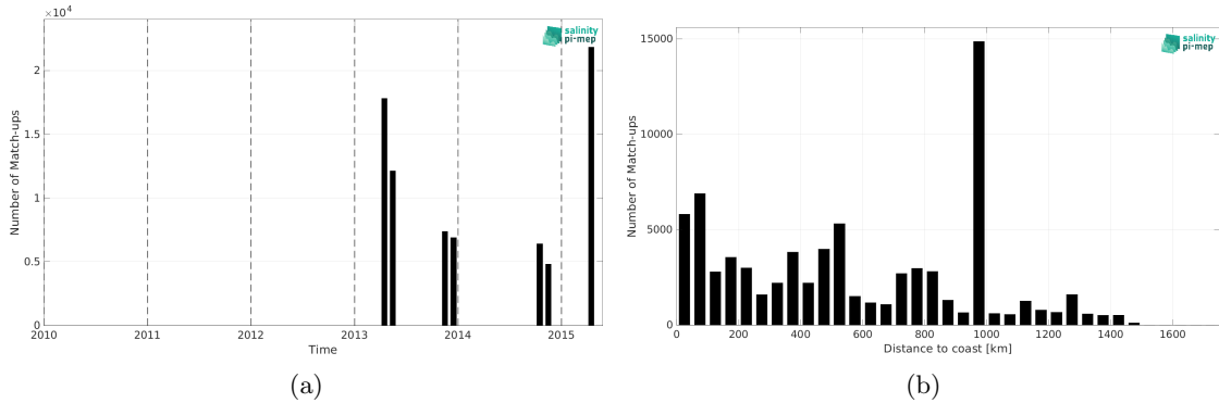
Figure 1: Number of match-ups between TSG (CSIC-UTM) and Aquarius SSS L3 OR v5 - 7-Day running (NASA-GSFC) SSS as a function of time (a) and as function of the distance to coast (b) over the Tropical Atlantic Ocean Pi-MEP region and for the full satellite product period.
