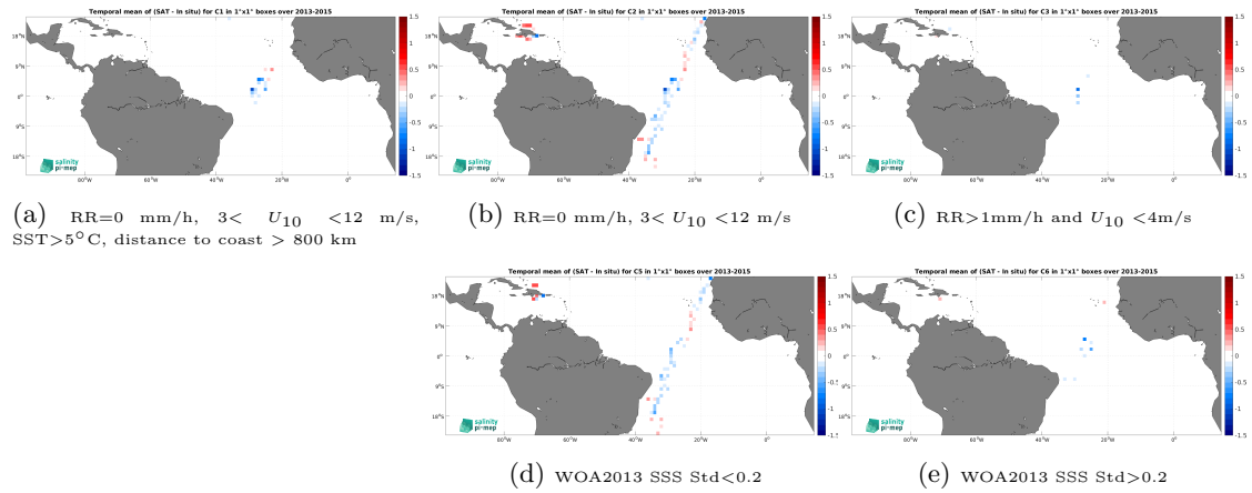
Figure 12: Temporal mean gridded over spatial boxes of size 1^{\circ}\times 1^{\circ} of \Delta\text{SSS} (Aquarius SSS L3 OR v5 - 7-Day running (NASA-GSFC) - TSG (CSIC-UTM)) for 5 different subdatasets corresponding to:RR=0 mm/h, 3 < U_{10} < 12 m/s, SST > 5^{\circ}\text{C} , distance to coast > 800 km (a), RR=0 mm/h, 3 < U_{10} < 12 m/s (b), RR > 1 mm/h and U_{10} < 4 m/s (c), WOA2013 SSS Std < 0.2 (d), WOA2013 SSS Std > 0.2 (e).
