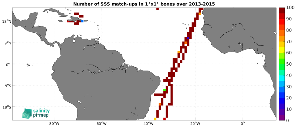
Figure 4: Number of SSS match-ups between TSG (CSIC-UTM) SSS and the Aquarius SSS L3 OR v5 - 7-Day running (NASA-GSFC) SSS product for the Tropical Atlantic Ocean Pi-MEP region over 1^\circ \times 1^\circ boxes and for the full satellite product period.
