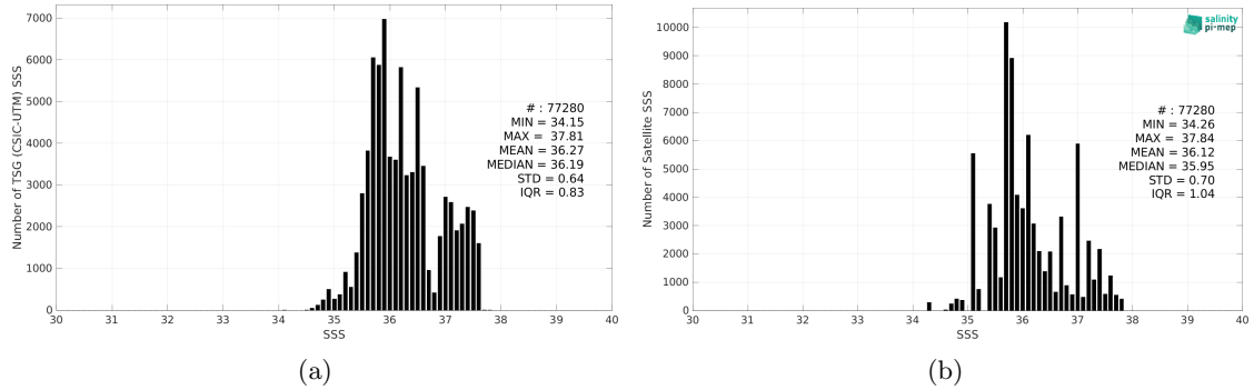
Figure 2: Histograms of SSS from TSG (CSIC-UTM) (a) and Aquarius SSS L3 OR v5 - 7-Day running (NASA-GSFC) (b) considering all match-up pairs per bins of 0.1 over the Tropical Atlantic Ocean Pi-MEP region and for the full satellite product period.
