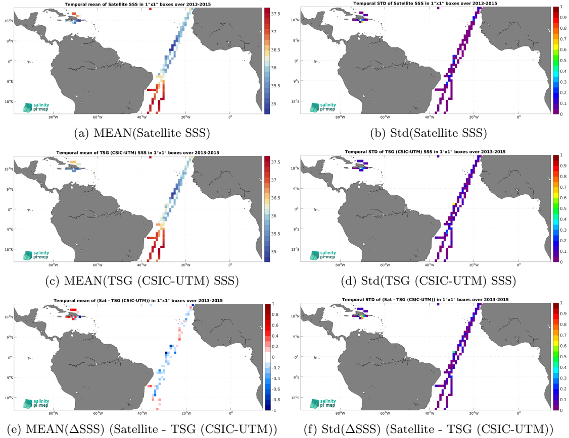
Figure 6: Temporal mean (left) and Std (right) of SSS from Aquarius SSS L3 OR v5 - 7-Day running (NASA-GSFC) (top), TSG (CSIC-UTM) (middle), and of \Delta\text{SSS} (Satellite - TSG (CSIC-UTM)). Only match-up pairs are used to generate these maps.
