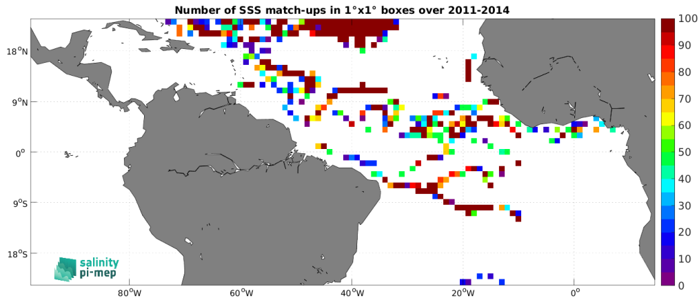
Figure 4: Number of SSS match-ups between Surface drifters SSS and the Aquarius SSS L3 OR v5 - 7-Day running (NASA-GSFC) SSS product for the Tropical Atlantic Ocean Pi-MEP region over 1^\circ \times 1^\circ boxes and for the full satellite product period.
