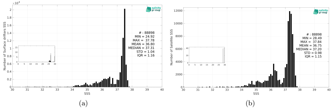
Figure 3: Histograms of SSS from Surface drifters (a) and Aquarius SSS L3 OR v5 - 7-Day running (NASA-GSFC) (b) considering all match-up pairs per bins of 0.1 over the Tropical Atlantic Ocean Pi-MEP region and for the full satellite product period.
