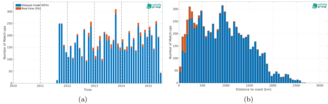
Figure 2: Number of match-ups between Argo and Aquarius SSS L3 OR v5 - 7-Day running (NASA-GSFC) SSS as a function of time (a) and as function of the distance to coast (b) over the Tropical Atlantic Ocean Pi-MEP region and for the full satellite product period.
