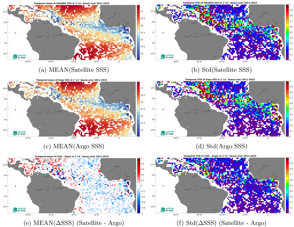
Figure 7: Temporal mean (left) and Std (right) of SSS from Aquarius SSS L3 OR v5 - 7-Day running (NASA-GSFC) (top), Argo (middle), and of \Delta SSS (Satellite - Argo). Only match-up pairs are used to generate these maps.
