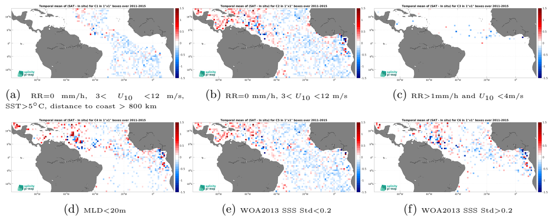
Figure 14: Temporal mean gridded over spatial boxes of size 1^\circ \times 1^\circ of \Delta SSS (Aquarius SSS L3 OR v5 - 7-Day running (NASA-GSFC) - Argo) for 6 different subdatasets corresponding to:RR=0 mm/h, 3 < U_{10} < 12 m/s, SST >5^\circ C, distance to coast > 800 km (a), RR=0 mm/h, 3 < U_{10} < 12 m/s (b), RR >1 mm/h and U_{10} < 4 m/s (c),MLD <20 m (d),WOA2013 SSS Std <0.2 (e),WOA2013 SSS Std >0.2 (f).
