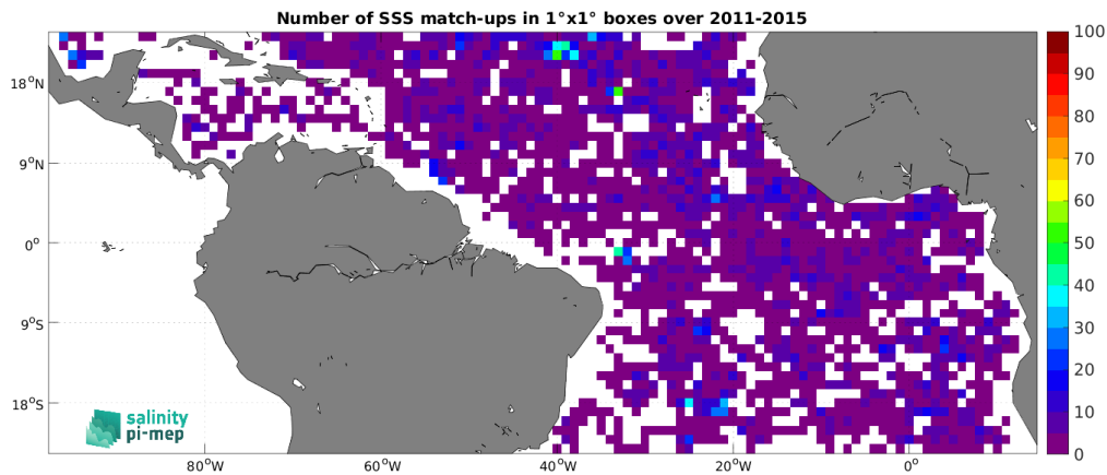
Figure 5: Number of SSS match-ups between Argo SSS and the Aquarius SSS L3 OR v5 - 7-Day running (NASA-GSFC) SSS product for the Tropical Atlantic Ocean Pi-MEP region over 1^\circ \times 1^\circ boxes and for the full satellite product period.
