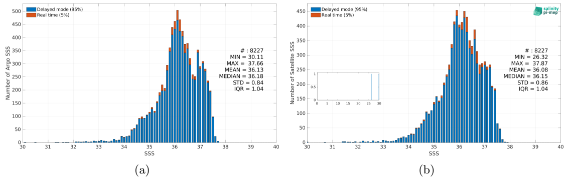
Figure 3: Histograms of SSS from Argo (a) and Aquarius SSS L3 OR v5 - 7-Day running (NASA-GSFC) (b) considering all match-up pairs per bins of 0.1 over the Tropical Atlantic Ocean Pi-MEP region and for the full satellite product period.
