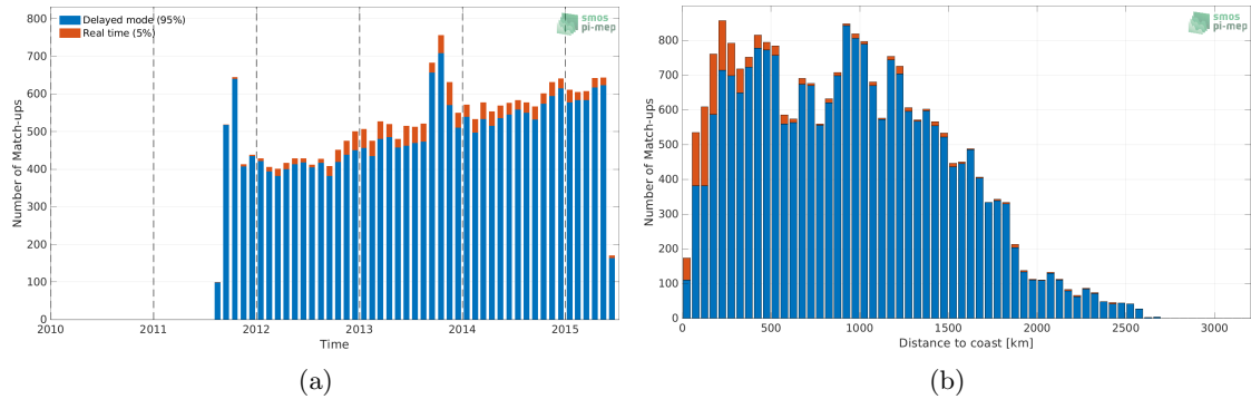
Figure 1: Number of match-ups between Argo and Aquarius SSS L3 OR v5 - 7-Day running (NASA-GSFC) SSS as a function of time (a) and as function of the distance to coast (b) over the Tropical Atlantic Ocean Pi-MEP region and for the full satellite product period.
