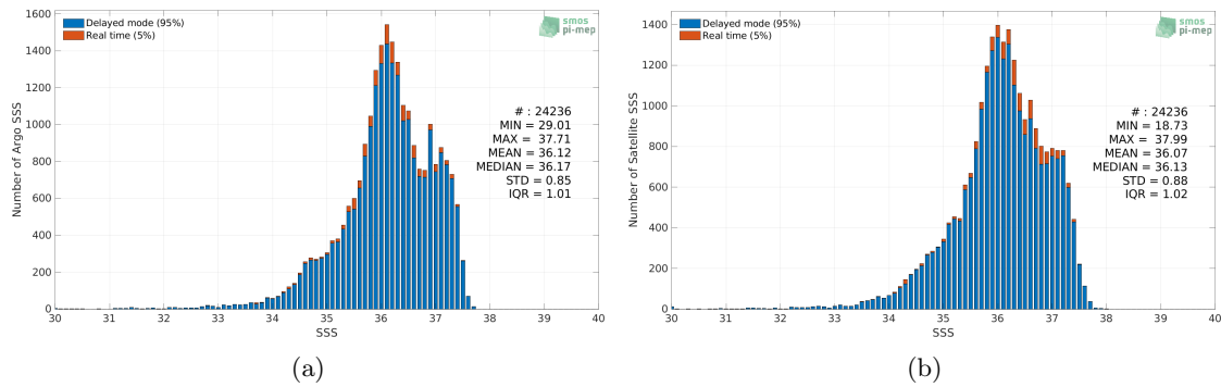
Figure 2: Histograms of SSS from Argo (a) and Aquarius SSS L3 OR v5 - 7-Day running (NASA-GSFC) (b) considering all match-up pairs per bins of 0.1 over the Tropical Atlantic Ocean Pi-MEP region and for the full satellite product period.
