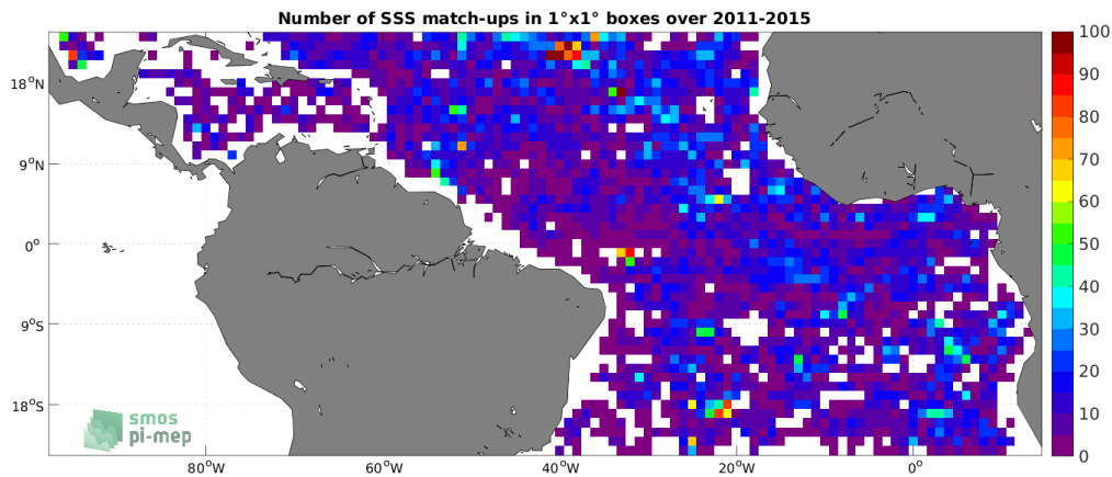
Figure 4: Number of SSS match-ups between Argo SSS and the Aquarius SSS L3 OR v5 - 7-Day running (NASA-GSFC) SSS product for the Tropical Atlantic Ocean Pi-MEP region over 1^\circ \times 1^\circ boxes and for the full satellite product period.
